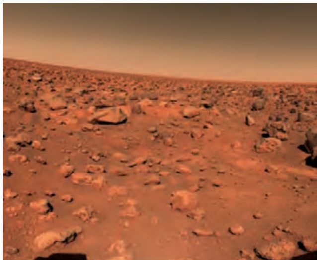
Figure 21.8. Mosaic of the Viking 2 landing site showing a flat, rocky, and dusty plain. Pitted rocks in the foreground suggest that they are volcanic basalts and the angular homogeneous rock field suggests that they are distal ejecta, perhaps from the fresh crater Mie to the east of the landing site. The lighter-toned trough in the middle of the image, in front of the large rocks, has been interpreted as an ice wedge polygon. Mosaic shows flat terrain at 1 km and 100 m scales, but rougher at the several meter length scale, consistent with MOLA-derived slopes and radar results. (For a color version of this figure, please refer to the color plate section or to the e-Book version of this chapter.)
