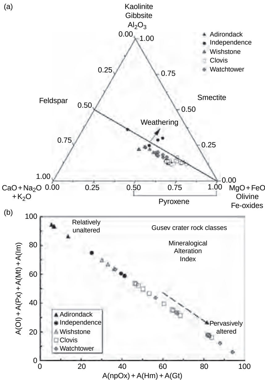
Figure 23.2. Chemical and mineralogical alteration indices for rock classes in the Columbia Hills, Gusev crater.
