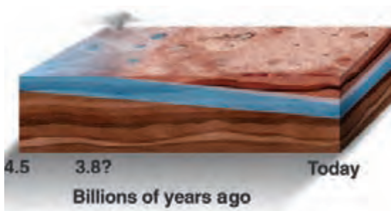
Figure 26.2. Hypothetical distribution of habitable environments, shown in light blue with wavy lines, in the Martian crust during its history. Surface and near-surface environments might have been habitable early in Martian history, whereas any habitable environments today might be restricted to a zone that lies a few kilometers below the surface. Graphics by Cheryse Triano, TopSpin Design Works. (For a color version of this figure, please refer to the color plate section or to the e-Book version of this chapter.)
