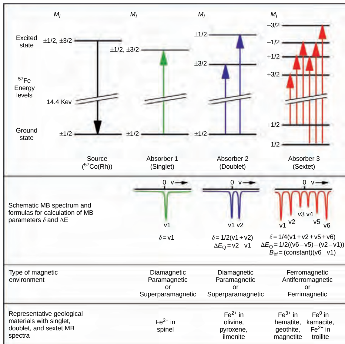
Figure 15.1. Energy level diagrams for ^{57}\text{Fe} for the cases of singlet, doublet, and sextet transmission Mössbauer spectra; schematic representation of the corresponding MB spectra and equations used for calculation of MB parameters \delta , \Delta E_Q , and B_{hf} ; and representative geologic materials. MER MB spectra are measured in backscatter geometry, so the MB spectra are emission peaks (i.e., essentially the inverse of the typical laboratory transmission geometry spectra shown here). For MER instruments (Klingelhöfer et al. , 2003), \delta is measured with respect to the center point of the spectrum of metallic Fe foil at approximately the same temperature as the sample. For peak centers in units of mm/s and B_{hf} in units of tesla (T), the constant in the formula B_{hf} = (\text{constant})(v_6 - v_1) equals 3.101. (For a color version of this figure, please refer to the color plate section or to the e-Book version of this chapter.)
