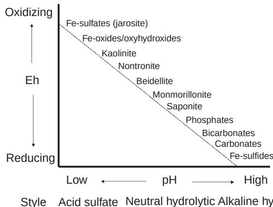
Figure 23.4. General environmental conditions and styles of weathering for the formation of secondary phases that might be present on Mars. Note: These conditions are provided only in a general sense. Formation conditions vary substantially for these phases.
