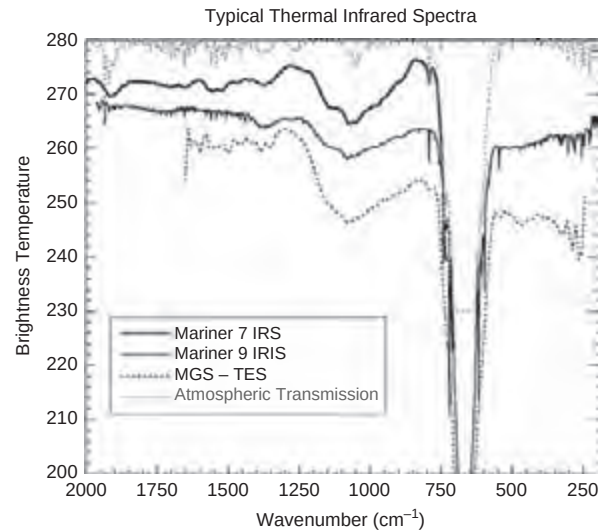
Figure 2.2. Typical thermal infrared spectra of Mars. The Mariner 7 IRS spectrum is an average of five spectra over Meridiani Sinus (M7 99:104). The Mariner 9 IRIS spectrum is an average of 1700 spectra acquired after orbit 100 (largely clear atmosphere). A typical TES spectrum from early in the mission is also shown. A calculated transmission spectrum for the Martian atmosphere multiplied by 50 and offset by 230 K is shown as the gray dashed line (Crisp, 1990).
