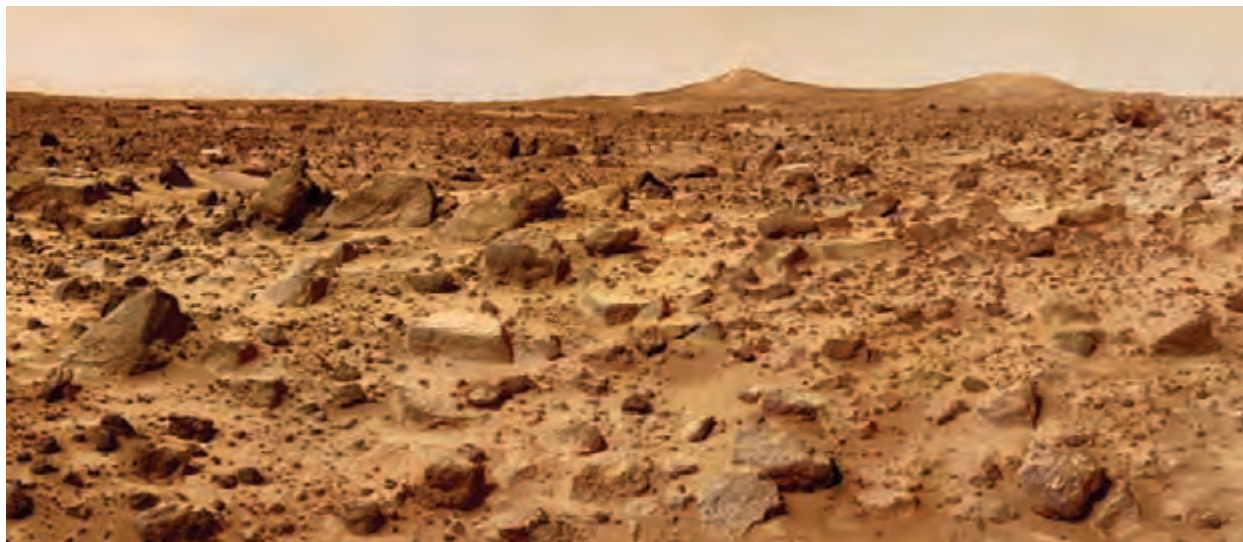
Figure 21.9. Mosaic of the Mars Pathfinder landing site showing an undulating, ridge-trough, moderately dusty and rocky plain. Large rocks in the middle left of the image appear stacked or imbricated on a ridge, with a trough behind it that trends toward the northeast. Streamlined hills on the horizon, the ridge-trough topography, and angular to subrounded boulders are consistent with depositional plains deposited by catastrophic floods, as expected from the setting of the site downstream from the mouth of the Ares Valles outflow channel. Note dust coating the tops of rocks. Mosaic shows this site to have the roughest terrain at 1 km, 100 m, and several-meter length scales, consistent with MOLA-derived slopes, radar roughness, and MOC stereogrammetry and photoclinometry results. (For a color version of this figure, please refer to the color plate section or to the e-Book version of this chapter.)
