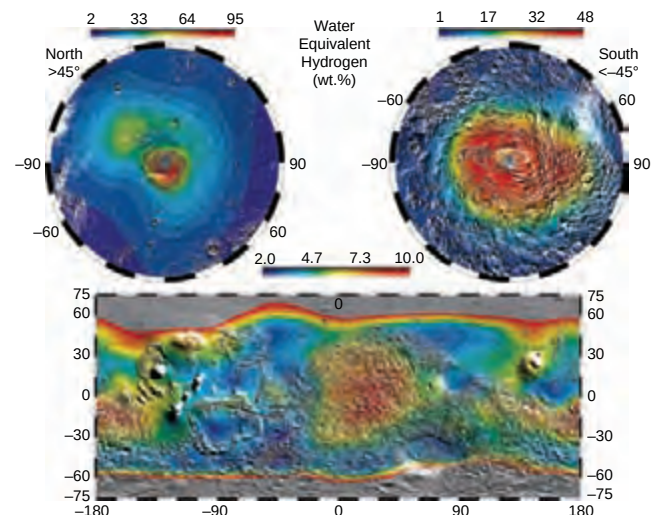
Figure 6.8. (above) Maps of water-equivalent hydrogen overlaid on shaded relief maps of Mars. The top maps are stereographic projections north of +45° latitudes (left) and south of -45° latitudes (right). The bottom map is a cylindrical projection between ±75° latitude.
