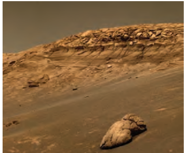
Figure 26.13. View eastward across Endurance crater to Burns Cliff. Eolian dune field deposits occur as tilted beds located in lower part of the cliff at left. Finely layered eolian sand sheet strata comprise the middle of the cliff, and the interdune/playa lake strata form the uppermost part of the cliff. Approximate true color Pancam image from sol 248, sequence P2269, filters 753 nm, 535 nm, and 480 nm. (For a color version of this figure, please refer to the color plate section or to the e-Book version of this chapter.)
