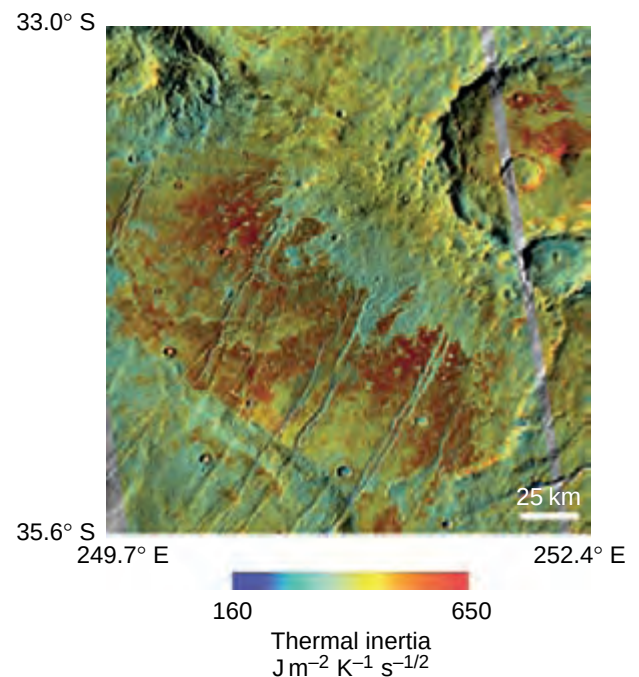
Figure 10.12. Exposed bedrock in the southern highlands. THEMIS thermal inertia mosaic (100 m/pixel resolution) overlaid onto a THEMIS daytime temperature mosaic, centered at 251.0° E, 34.3° S.
