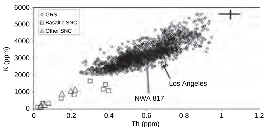
Figure 5.10. K and Th mass fractions (mg/kg) in 5° × 5° smoothed pixels from Mars Odyssey GRS data compared to basaltic (includes olivine phyric) SNC and other SNC meteorites. GRS data collected through March 2005. Uncertainty is shown for a typical GRS data point. SNC data are from Lodders (1998) and Meyer (2003) and references therein. Note that all but two meteorites (basaltic shergottite Los Angeles and nakhlite NWA 817) plot substantially below GRS data, implying that the meteorites are not representative of typical Martian surface materials.
