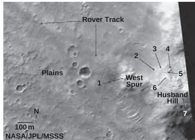
Figure 14.3. Mars Orbiter Camera image (R2001024) showing locations in Gusev crater described in this work. Numbered locations are as follows: (1) Clovis outcrop; (2) Wishstone float rock; (3) Peace/Alligator outcrop; (4) Larry's Lookout; (5) Backstay float rock; (6) Independence outcrop; and (7) Irvine float rock.
