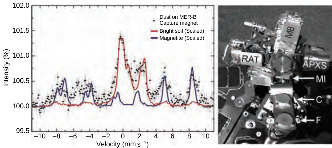
Figure 16.9. Mars Exploration Rover Opportunity Mössbauer spectrum (sols 328–330) of Martian airborne dust as attracted to the capture magnet. To the right, a navigation camera context image from sol 328 showing the Microscopic Imager (MI) in position for imaging of the capture magnet (C). Following MI imaging, the turret of the robotic arm was turned by approximately 180^\circ for placing the Mössbauer (MB) spectrometer on the capture magnet. Also labeled in the figure is the filter magnet (F), as well as the remaining IDD instruments (RAT, APXS). (For a color version of this figure, please refer to the color plate section or to the e-Book version of this chapter.)
