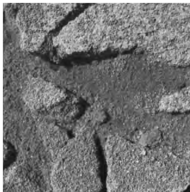
Figure 20.12. Spirit MI image of a disrupted soil crust containing well-sorted 200–300 \mu\text{m} grains, overlying finer material (darker zones in image). Weak soil crusts of varying thicknesses and strengths are common at both MER landing sites. Image 2M170218789IFFAAEEP2976M2F1, obtained on Sol 494 with direct illumination from the upper left, spans about 31 mm.
