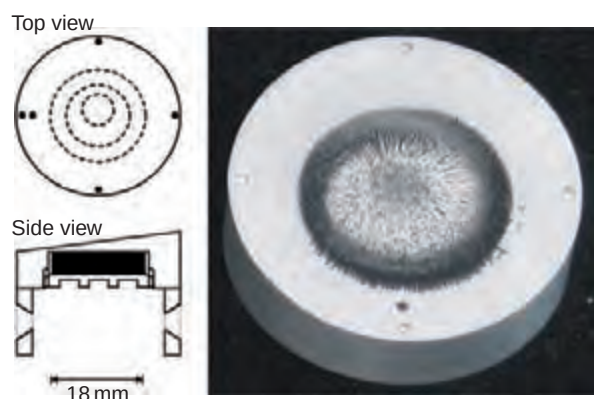
Figure 16.12. Spontaneous formation of magnetic chains in the laboratory with a sample of synthetic magnetite (BASF black pigment). The magnet shown is the Mars Pathfinder tip plate magnet. This magnet was designed to create a range of magnetic field gradients across the surface of the magnet by an asymmetric position of the central disk magnet and a wedged surface of the aluminum structure. On the image (right) this variation of magnetic fields can be seen reflected in the varying separation between the particle chains particularly along the inner rim of the ring on the surface of the magnet. The small dots in the surface of the structure serve as orientation markers. (For a color version of this figure, please refer to the color plate section or to the e-Book version of this chapter.)
