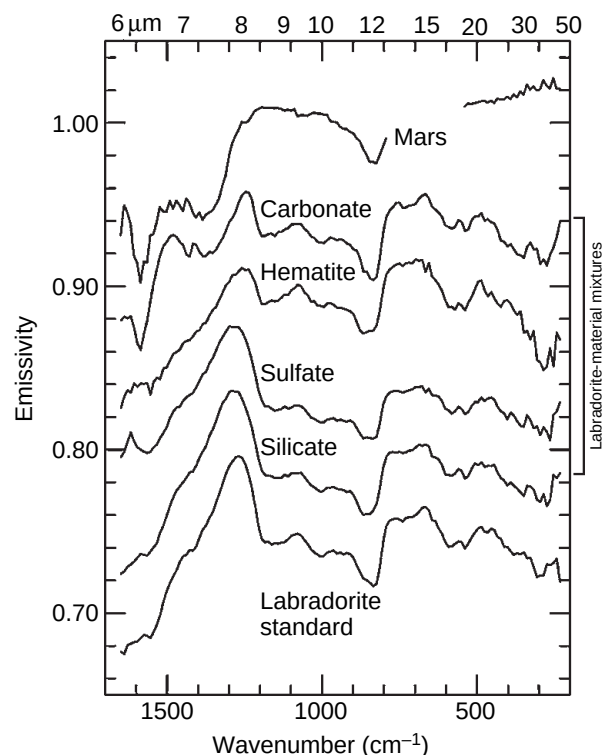
Figure 9.9. Mars dust, labradorite standard, and labradorite-material mixture spectra (offset). The spectral shape of labradorite is modified considerably with added carbonate at 1300\text{ cm}^{-1} , coincident with a fundamental carbonate absorption. The spectral shape outside this spectral region is not appreciably modified because strong silicate absorptions coincide with the other carbonate absorptions. Only the labradorite-carbonate mixture has a notable effect on the spectral shape, except for a peak present in the labradorite-sulfate mixture at 1640\text{ cm}^{-1} due to the bound water in gypsum. (From Bandfield, J. L., T. D. Glotch, and P. R. Christensen, Spectroscopic identification of carbonates in the Martian dust, Science 301 , 1084–87, 2003. Reprinted with permission from AAAS.)
