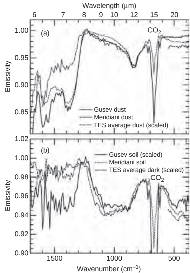
Figure 14.5. The spectra of light-toned dust and dark-toned soil observed by Mini-TES and TES. (a) The light-toned dusty mantle observed at both landing sites is remarkably similar at each and to the average global dust observed by TES (Bandfield and Smith, 2003). (b) Dark-toned soil observed in the rover tracks in Gusev (“Tracks,” p3660, sol 89) and in a sand pile in Meridiani (“Auk,” p3839, sol 197) (Yen et al. , 2005) look similar to the global average dark-toned surfaces observed by TES (Bandfield and Smith, 2003). The Gusev soil has a dust component that causes the mismatch at wavenumbers > 1300.
