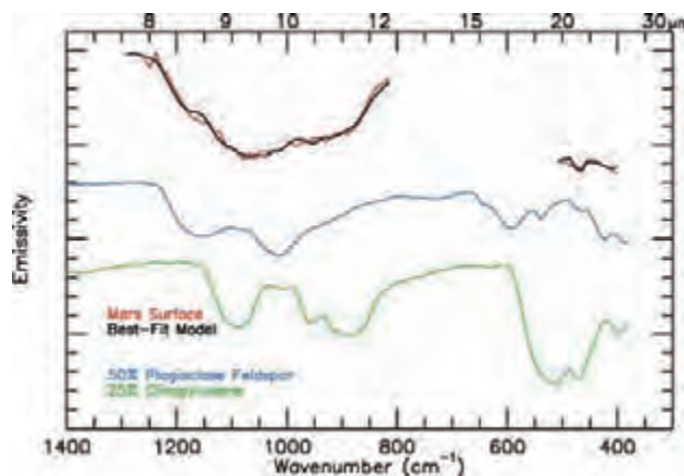
Figure 9.2. Deconvolution of TES basalt spectrum of Cimmeria. TES spectra from this region are well matched by plagioclase, pyroxene, and minor olivine and other phases. (Adapted from Christensen et al. , 2000b.) (For a color version of this figure, please refer to the color plate section or to the e-Book version of this chapter.)
