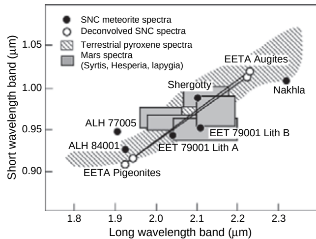
Figure 17.5. Long- and short-wavelength band positions for terrestrial pyroxenes (Cloutis and Gaffey, 1991), SNC meteorites (McFadden, 1987; Sunshine et al. , 1993; Bishop et al. , 1994), and dark regions of Mars (Singer et al. , 1980; Mustard et al. , 1993). Deconvolved spectra for EET 79001 shergottite (Sunshine et al. , 1993) are from separate pigeonite and augite phases.
