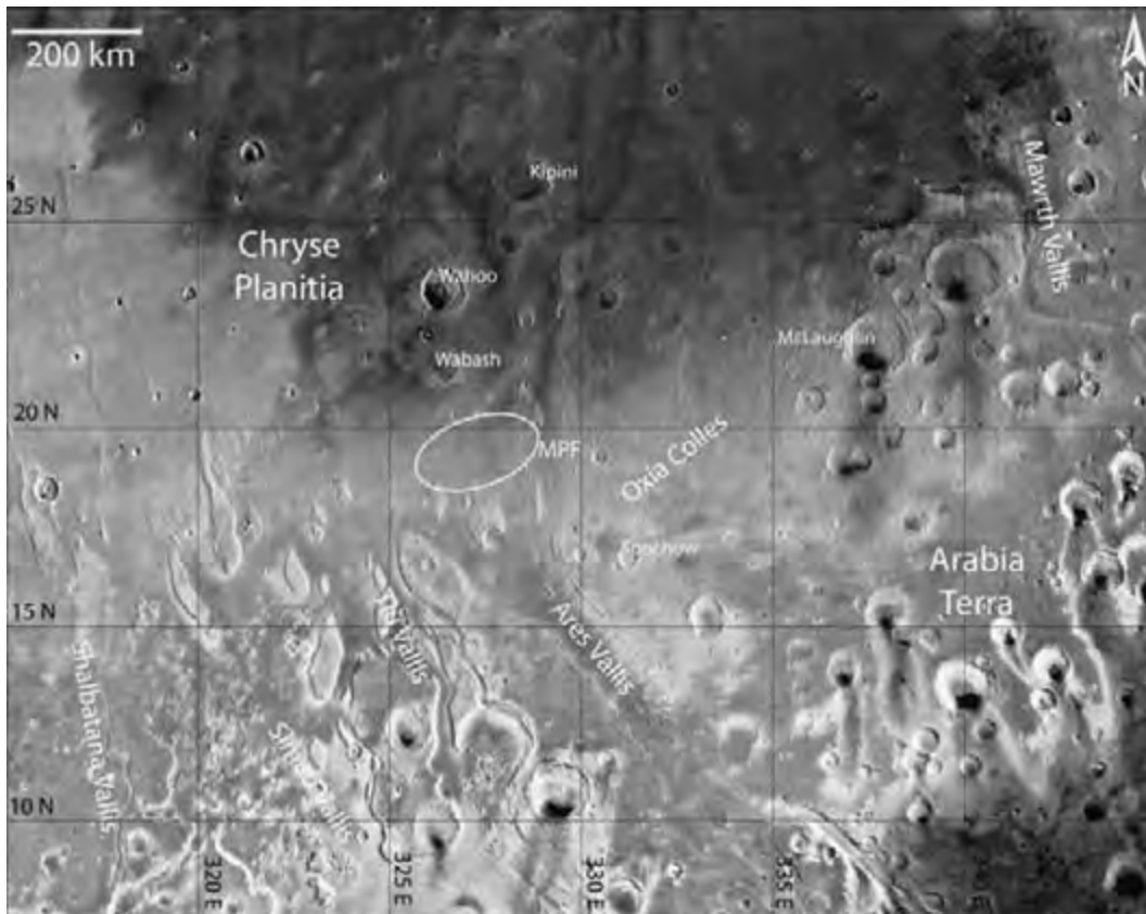
Figure 21.2. Regional mosaic of Chryse Planitia, Ares Vallis, and the Mars Pathfinder landing ellipse. Mosaic shows catastrophic outflow channels cutting the heavily cratered (ancient) terrain to the south and flowing to the lower northern plains. Ares Vallis is about 100 km wide and 2 km deep. Streamlined islands produced during the flooding are located throughout the scene. The Mars Pathfinder landing ellipse shown is 200 km by 100 km and lies about 100 km north of the mouth of the channel where it exits the highlands, and thus was interpreted to be a depositional plain composed of materials deposited by the floods. Characterization of the surface after landing supports this interpretation.
