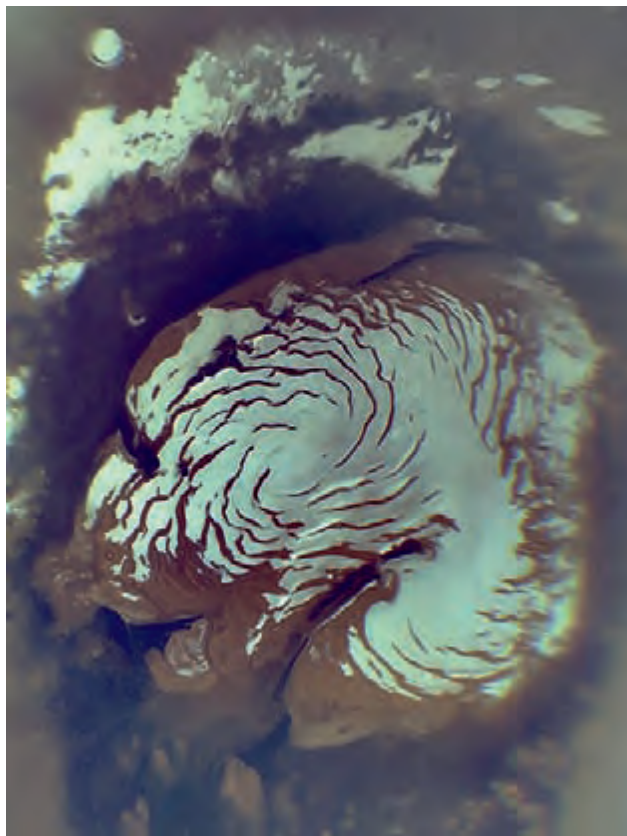
Figure 8.16. Initial MRO/MARCI 600, 550, 425 nm RGB color composite image of the north polar cap, acquired at the start of MRO orbital operations in late September 2006. The northern summer residual water ice cap seen here is about 1000 km in diameter. MARCI resolution is about 900 m/pixel. The resolution decrease on the right side of the field of view is an artifact of the map projection used here. (For a color version of this figure, please refer to the color plate section or to the e-Book version of this chapter.)
