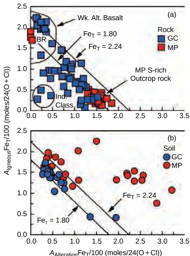
Figure 15.8. Plots of A_{\text{igneous}} \text{Fe}_T/100 versus A_{\text{alteration}} \text{Fe}_T/100 for (a) rock and (b) soil at Gusev crater (GC) and Meridiani Planum (MP). Solid lines correspond to \text{Fe}_T = 2.24 and 1.80 moles/24(O+Cl). Weakly Altered Basalts (Wk. Alt. Basalt) plot near the upper left corner of (a). Assuming that all unaltered Martian rocks have \text{Fe}_T > 1.0 moles/24(O+Cl) and A_{\text{alteration}} \text{Fe}_T/100 \sim 0 moles/24(O+Cl), compositions that plot on the y-axis of (a) with \text{Fe}_T < 1.0 moles/24(O+Cl) are rocks altered in an open system without retention of Fe-bearing alteration products. Independence Class (Ind. Class) rocks, for example, are examples of rocks that show evidence for alteration in an open system. Samples that plot along a line of constant \text{Fe}_T (e.g., \text{Fe}_T = 2.24 and 1.80 moles/24(O+Cl)) are only potentially related by isochemical alteration (on an \text{H}_2\text{O} -free basis), because all elemental concentrations must be considered to validate isochemical alteration. For example, in (a), Bounce Rock (BR) and MP S-rich outcrop rocks plot along the line with \text{Fe}_T = 1.80 moles/24(O+Cl) but are not related by isochemical alteration because of differences in major element chemistry (e.g., Rieder et al. , 2004). (For a color version of this figure, please refer to the color plate section or to the e-Book version of this chapter.)
