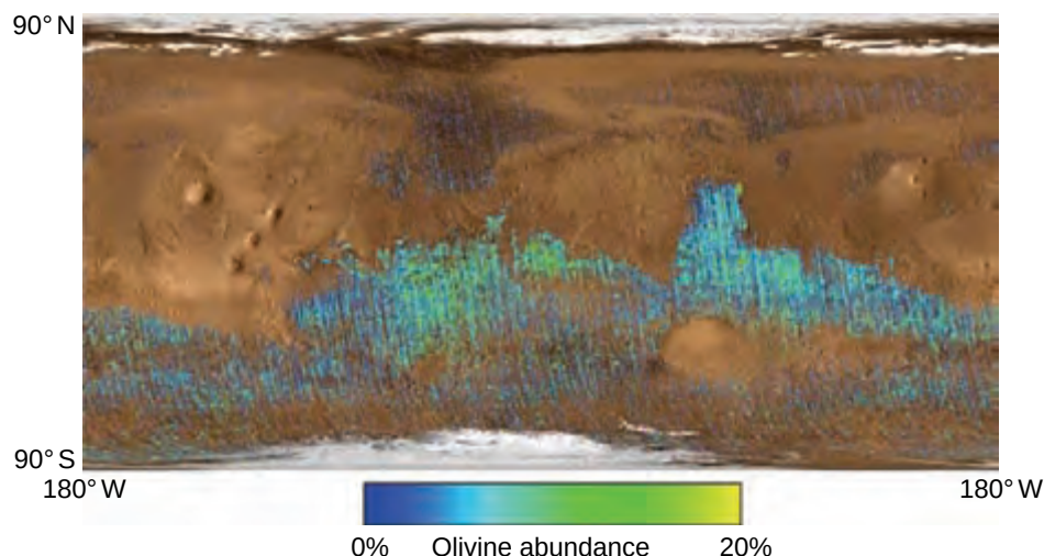
Figure 9.5. TES mineral map of olivine superimposed on the MOLA shaded relief map for location. (Based on McSween et al. , 2006.) (For a color version of this figure, please refer to the color plate section or to the e-Book version of this chapter.)
