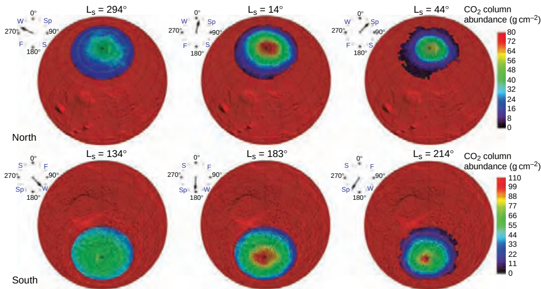
Figure 25.9. Maps of CO 2 column abundance in the northern and southern hemispheres (poleward of 60^\circ ) are compared to cap edge functions (solid red line) and the extent of the polar night (dashed green line). In both hemispheres, the maximum column abundance occurs near the pole during the recession. In the southern hemisphere, the distribution is asymmetric, with peak column abundance occurring at the location of the perennial CO 2 cap.
