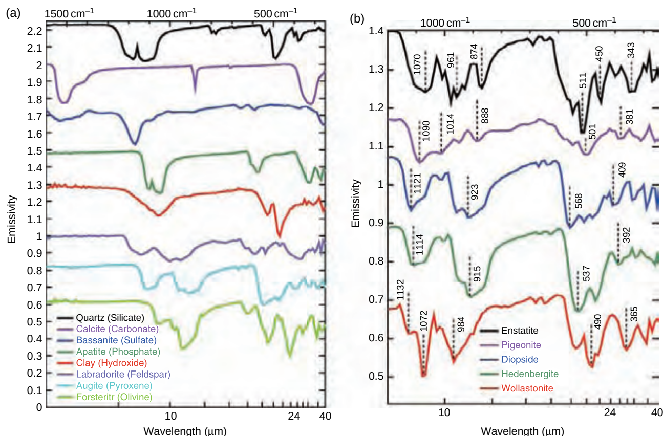
Figure 9.1. Infrared spectra of representative minerals. (a) Major mineral groups; (b) Pyroxene minerals. Band centers are indicated in \text{cm}^{-1} . (For a color version of this figure, please refer to the color plate section or to the e-Book version of this chapter.)
