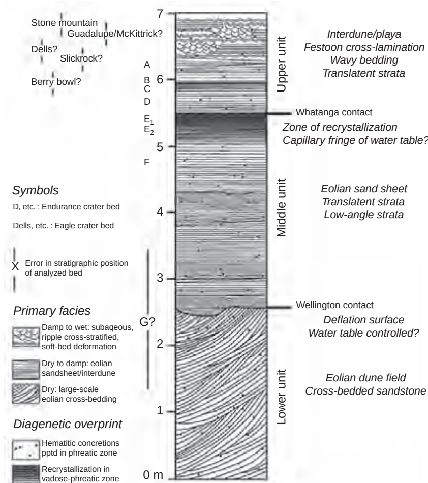
Figure 26.14. Schematic cross section of bedrock units exposed at Burns cliff, Endurance crater. The sedimentary structures and textures are consistent with a “wetting upward” transition from an eolian dune field (bottom) to eolian sheet sands to interdune/playa lake rippled sands (top). (Illustration from Grotzinger et al. , 2005. Reproduced with permission from Elsevier.)
