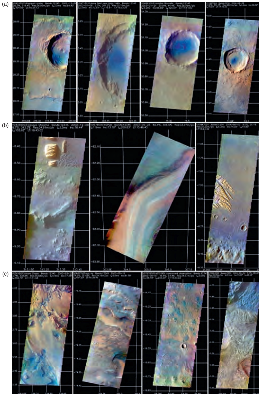
Figure 8.4. (a) Examples of "Blue Crater Materials" observed in false-color THEMIS-VIS images. VIS imaging sequences V04333003, V04733003, V04893003, and V11997004. (b) Examples of "Layered Materials" observed in false color THEMIS-VIS images. VIS imaging sequences V04359003, V06780004, and V10947001. (c) Examples of "Etched Terrain" observed in false-color THEMIS-VIS images. VIS imaging sequences V05618015, V06317005, V07676005, V10963002.
