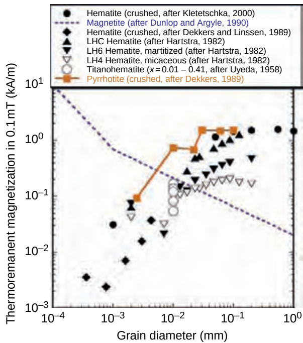
Figure 11.3. TRM magnetizations for the three main candidate minerals that could constitute the source of the magnetic anomalies on Mars. (For a color version of this figure, please refer to the color plate section or to the e-Book version of this chapter.)
