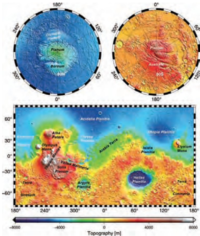
Figure 1.1. Global topography of Mars from the MGS MOLA experiment. (Credit: NASA and the Mars Global Surveyor Mars Orbiter Laser Altimeter Team.)
