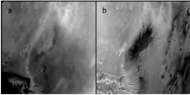
Figure 19.3. Images of Juventae Chasma (looking to the northeast) acquired by Viking Orbiter 1 under different phase angles ( g ): (a) Image 759A67 ( g = 113^\circ ); (b) Image 334S41/43 ( g = 37^\circ ). At high phase angles the strongly forward-scattering sand deposits in the interior of Juventae are brighter than the neighboring plains, whereas at lower phase angles, the low-albedo sand deposits are darker than the plains.
