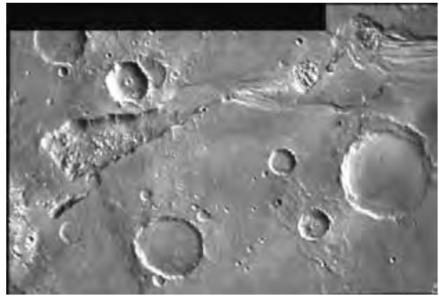
Figure 26.5. Ravi Vallis catastrophic outflow channel. Source region at left suggests eruption of liquid water from the subsurface. Well-defined channel and erosion features indicate flow of liquid water over the surface toward the upper right.
