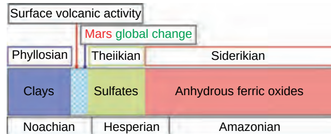
Figure 7.21. An OMEGA-derived Mars mineralogical history/timeline. (For a color version of this figure, please refer to the color plate section or to the e-Book version of this chapter.)
