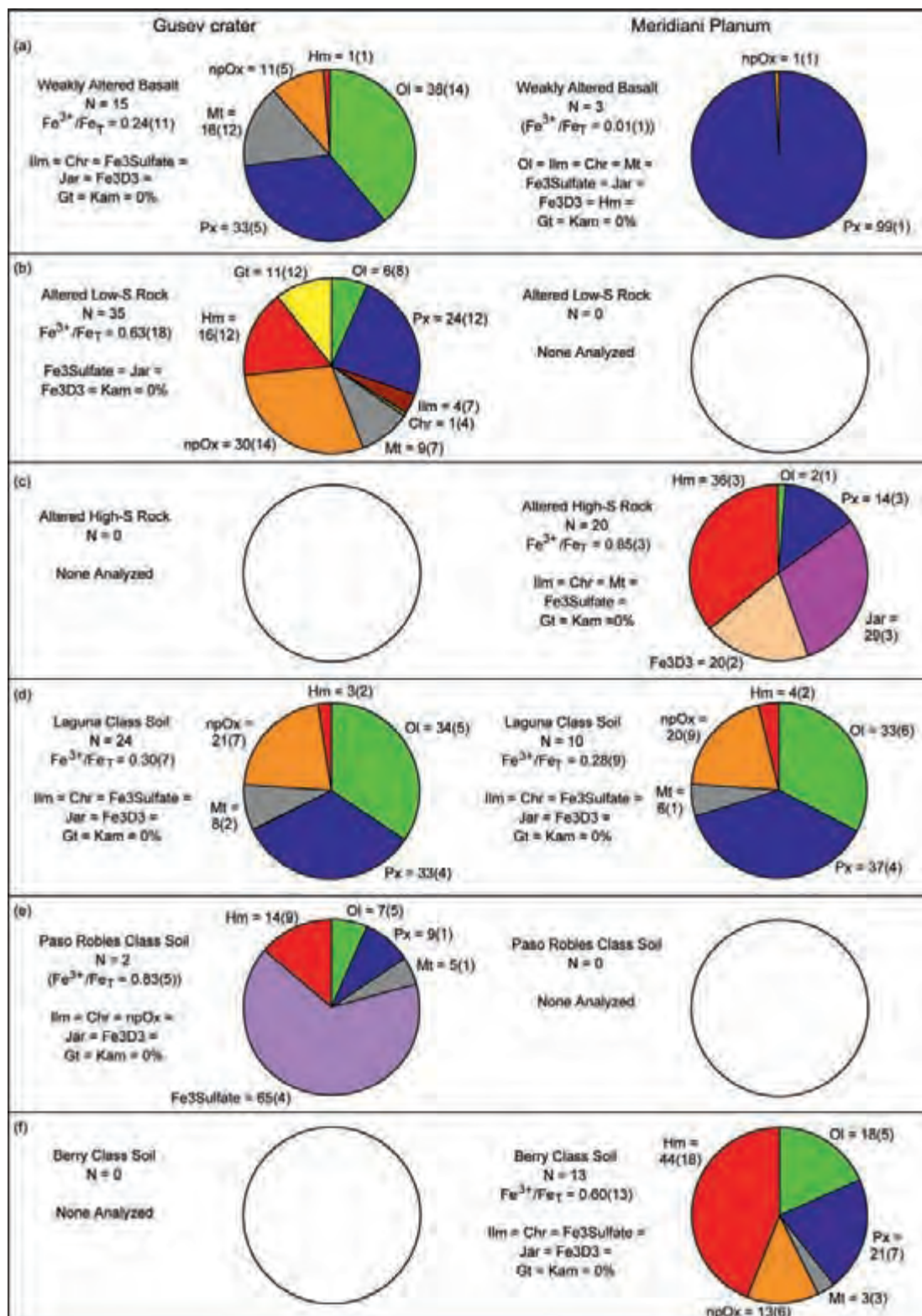
Figure 15.9. Pie diagrams showing the average values ( 1\sigma standard deviation in parenthesis) of Fe from Fe-bearing phases ( A_x , where x = \text{Ol, Px, Ilm, Chr, Mt, npOx, Fe3Sulfate, Fe3D3, Jar, Hm, and Gt} ) for rock and soil supergroups at Gusev crater (as of sol 602) and Meridiani Planum (as of sol 557): (a) Weakly Altered Basalt, (b) Altered Low-S Rock, and (c) Altered High-S Rock for RAT-ground surfaces, (d) Laguna Class soil, (e) Paso Robles Class soil, and (f) Berry Class soil. Altered High-S Rock and Berry Class soil are not present at Gusev crater and Altered Low-S Rock and Paso Robles Class soil are not present at Meridiani Planum. The distribution of Fe from Fe-bearing phases for Gusev crater Weakly Altered Basalt (a) is very similar to that for Laguna Class soil (d), except the latter has more Fe from npOx. The meteorite supergroup (not shown), whose distinguishing characteristic is kamacite as an Fe-bearing phase, includes two rocks from Meridiani Planum (Heat Shield and Barberton) and no rocks from Gusev crater. The average concentrations of Fe associated with iron-bearing phases ( A_x\text{Fe}_T/100 ) are given in Table 15.3.
