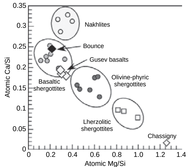
Figure 17.8. Geochemical classification diagram for SNC meteorites (Ouri et al. , 2003), also showing compositions of Gusev basalts and Bounce Rock analyzed by the Mars Exploration Rovers.
