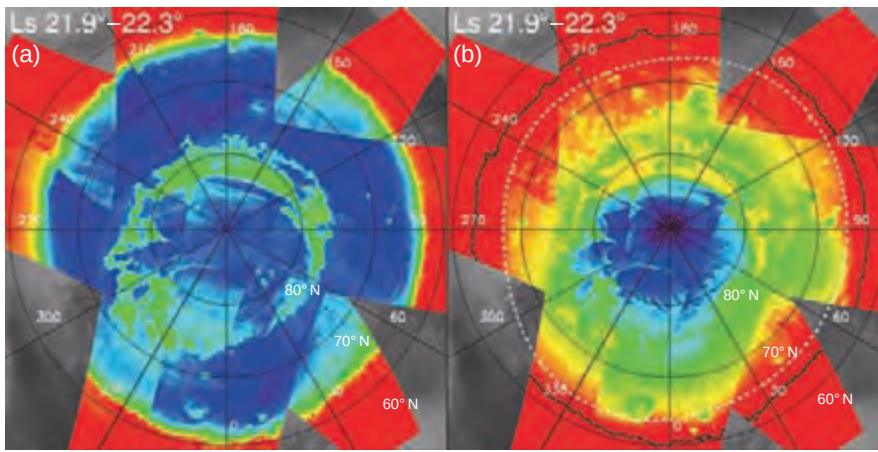
Figure 7.3. Seasonal evolution of the northern polar cap: spatial distribution of spectral signatures of H 2 O ice and CO 2 ice observed by OMEGA in early northern spring ( L_s = 22^\circ , March 2006). (a) Band depth of the H 2 O ice absorption feature at 1.5 \mu\text{m} . The rainbow scale covers the range from 60% (black) to 0% (red); (b) band depth of the CO 2 ice absorption feature at 1.43 \mu\text{m} , also from 60% (black) to 0% (red). The annulus observed by TES between the boundary of bright regions (black line on panel (b)) and that of regions at the equilibrium temperature of CO 2 ice (the so-called “crocus line,” white dashes, from Titus et al. , 2003) is confirmed as being constituted of H 2 O frost. At this season, the strongest CO 2 ice signatures (corresponding to large mean grain sizes) are observed over regions corresponding to the central parts of the north permanent cap.
