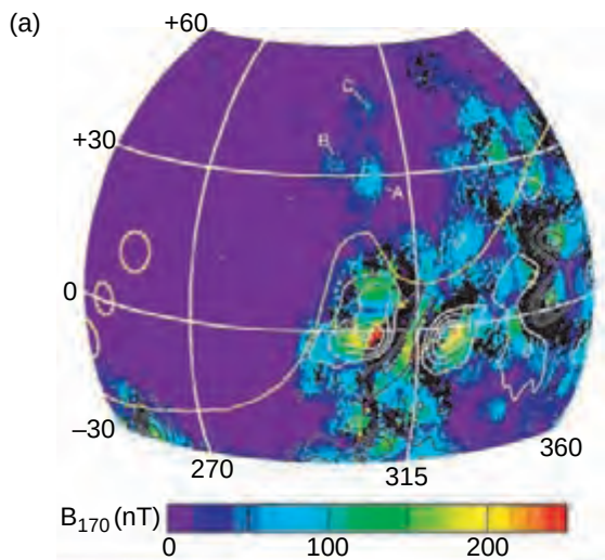
Figure 11.2. (a) The crustal magnetic field strength at 170 km altitude, as inferred from electron reflectometry, is averaged in 0.5^\circ \times 0.5^\circ bins (color scale). All data were obtained at 2 a.m. local time. Double-sided loss cones were observed in black regions within 45^\circ of the equator, indicating that the spacecraft was on closed crustal magnetic field lines (miniature magnetospheres – see Figure b). Contours show the radial component of the magnetic field measured by the MAG at 400 km (Connerney et al. , 2001) (white: negative; black: positive). The locations of the Tharsis volcanoes and the dichotomy boundary are shown in orange (based on Lillis et al. , 2004). (b) A global map of Martian magnetization at 170 km altitude derived from electron reflectometer measurements superimposed on a shaded relief map of MGS MOLA topography (based on Mitchell et al. , 2007). Grayscale regions have B_{170} < 10 nT. Crustal magnetic field lines form closed loops in the black regions where the electron reflectometer method cannot be used. Labels indicate the centers of the impact basins of Utopia (U), Hellas (H), Argyre (A), and Isidis (I) as well as the volcanoes Elysium (e), Syrtis Major (s), Apollinaris (o), Tyrrhena (t), Hadriaca (h), Peneus (p) and Amphitrites (a). (For a color version of this figure, please refer to the color plate section or to the e-Book version of this chapter.)
