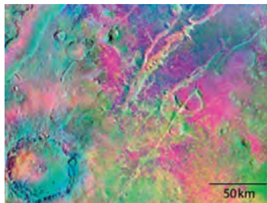
Figure 10.1. Olivine-rich basalts in Nili Fossae. Decorrelation-stretched (DCS) infrared mosaic of Nili Fossae region (20° N to 23.5° N, 75° E to 80° E). DCS bands 9 (12.57 \mu\text{m} ), 7 (11.04 \mu\text{m} ), and 5 (9.35 \mu\text{m} ) are displayed as red, green, and blue, respectively. Olivine exposures are magenta to purple-blue in color. North is to the top in all images. North is up in all figures unless otherwise noted. (For a color version of this figure, please refer to the color plate section or to the e-Book version of this chapter.)
