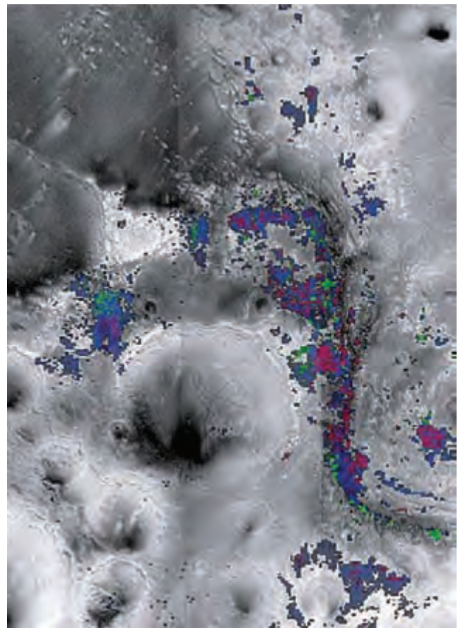
Figure 7.20. Clays in Mawrth Vallis. Distribution, over an HRSC mosaic (3 contiguous maps), of the minerals identified by OMEGA through their 1.93 \mu\text{m} (hydration, blue), 2.20 \mu\text{m} (montmorillonite, green), and 2.30 \mu\text{m} (Mg/Fe-rich smectites, red) features. (For a color version of this figure, please refer to the color plate section or to the e-Book version of this chapter.)
