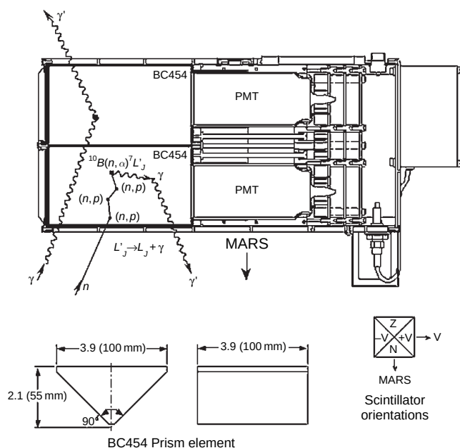
Figure 6.1. A line drawing of the sensor element of MONS showing the different kinds of neutron and gamma-ray interactions.
