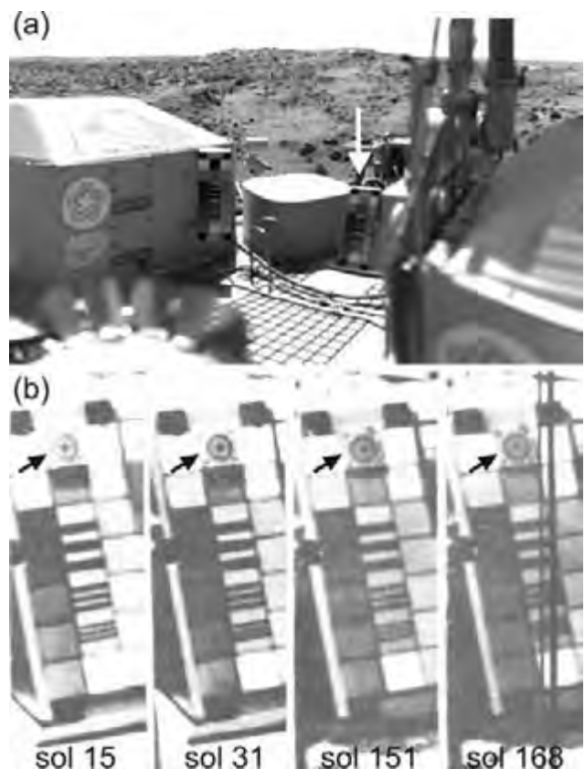
Figure 16.6. Bull’s-eye magnet (arrow) on one of the Reference Test Charts (RTC) for the cameras onboard Viking Lander 1. (a) Location of RTC on lander deck. (b) Accumulation of magnetic, wind-blown dust over time.
