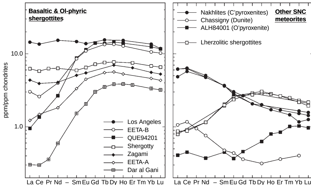
Figure 22.3. REE concentrations in Martian meteorites.
