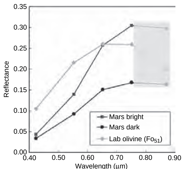
Figure 8.5. Mars bright and dark region spectra from Mustard and Bell (1994) and laboratory olivine spectrum convolved to THEMIS-VIS band passes. Shading indicates spectral region with considerable uncertainty because of scattered light in the 860 nm THEMIS-VIS data (McConnochie et al. , 2006).
