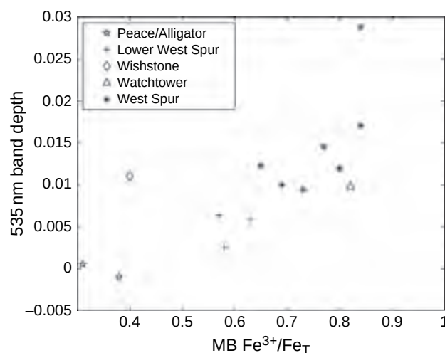
Figure 13.5. Plot of \text{Fe}^{3+}/\text{Fe}_T as measured by Spirit ’s Mössbauer spectrometer (MB) versus 535 nm band depth for areas in the Columbia Hills that were subjected to in situ examinations.
