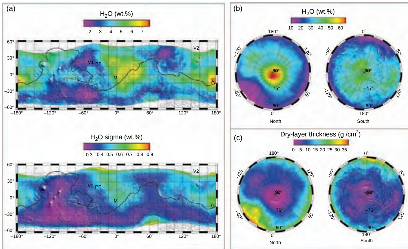
Figure 5.4. (a) Map of the mass fraction (%) of H 2 O (stoichiometrically determined from H content) and the I_{sm} in the equatorial region of Mars. The black outline and letters are as in Figure 5.3. (b) Lower-limit H 2 O content in the polar regions based on models shown in Figure 5.7 with the assumption that there is no dry layer, that is, that the H 2 O is homogeneously distributed. The high H 2 O contents suggest that the ice was deposited on the surface of the soil with modest amounts of dust mixed into the ice as it was being deposited. (c) Map of the maximum dry-layer thickness in the polar regions based on models shown in Figure 5.7, but in this case the assumption is made that the lower layer is actually pure ice, 100% H 2 O.
