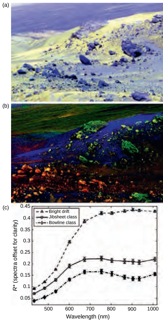
Figure 13.3. (a) False-color composite (red=673 nm, green=535 nm, blue=432 nm) of the sol 608 P2582 Whittaker/Bowline scene. (b) Composite of endmember fraction images of spectrally distinct rock and soil components (red=Bowline type rocks; green=Whittaker/Hillary [Jibsheet class] type rocks; blue=bright drift soil). (c) Spectra of materials mapped out in the fraction image composite image. R^* is the radiance factor normalized by the solar elevation angle (Bell et al. , 2006b). (For a color version of this figure, please refer to the color plate section or to the e-Book version of this chapter.)
