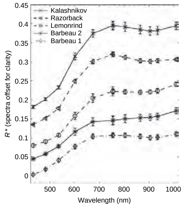
Figure 13.27. Spectra of coating/fracture-fill materials from Endurance crater. An example of the “red rind” material from the Shoemakers Patio area at Eagle crater is also provided, from the target named Kalashnikov. The Barbeau 2 material spectrum is offset upward by 0.02.
