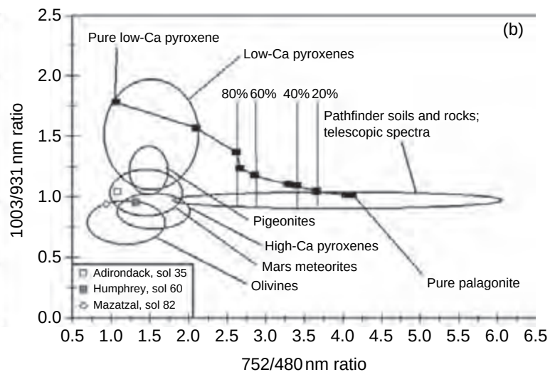
Figure 13.10. (a) Pancam spectra of grinding debris and dark, “pristine” inner rock surfaces exposed by the RAT on the Gusev plains rocks Adirondack, Humphrey, and Mazatzal. (b) Ratios of the spectra in (a) compared to laboratory-derived spectral parameterizations of olivines, pyroxenes, Martian meteorites, and pyroxene-palagonite mixtures studied by Cloutis and Bell (2003). The Gusev rock spectra appear consistent with an olivine- or high-Ca-pyroxene dominated basaltic composition. (Figure after McSween et al. , 2006b.)
