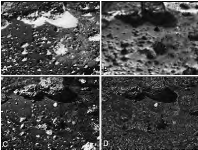
Figure 12.4. Fraction images and RMS error image from spectral mixture analysis of an MPF component left eye image segment from the S0185 SuperPan octant. (a)–(c) represent, respectively the shade, bright drift, and rock image endmembers. (d) is the RMS error image. The bright rock with the high RMS error image is a detection of the Black Rock spectral class.
