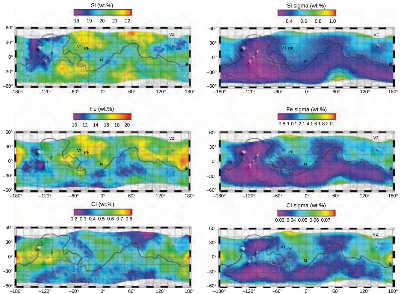
Figure 5.3. Maps of the Si, Fe, and Cl mass fractions (left) and of the 1.s_m (right) variation at each point on Mars, in the equatorial zone where H concentrations are low enough to allow for ready calculation of elemental abundances. s_m is basically the instrumental uncertainty at each point (as an absolute, not relative, mass fraction) and consequently unrelated to the standard deviation of the sample population. Data have been smoothed using a mean filter. The data are displayed over a shaded relief map of Mars, with mission landing sites indicated (V1: Viking 1 in Chryse Planitia; V2: Viking 2 in Utopia Planitia; PF: Pathfinder in Ares Vallis; M: Opportunity in Meridiani Planum; G: Spirit in Gusev crater). The black outline is the 0 km contour, which roughly corresponds to the boundary between the southern highlands and northern lowlands. (For a color version of this figure, please refer to the color plate section or to the e-Book version of this chapter.)
