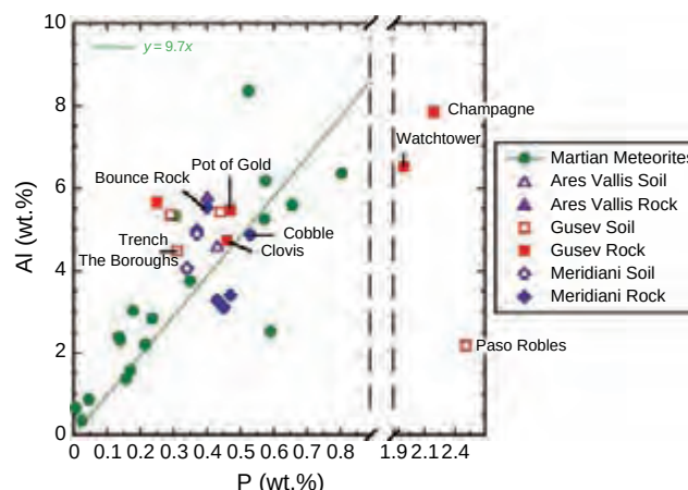
Figure 4.24. Aluminum versus phosphorus content for different Martian samples. Note the break in the x -axis. (For a color version of this figure, please refer to the color plate section or to the e-Book version of this chapter.)
