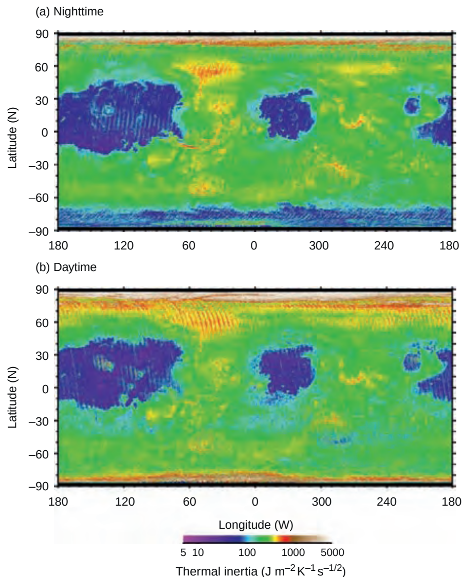
Figure 18.8. Global map of the thermal inertia of Mars based on TES (a) nighttime and (b) daytime bolometric brightness temperature observations (see Putzig and Mellon, 2007b). Maps are generated by a median filter of 36 seasons over 3 Mars years and are binned at 1/20^\circ per pixel. Nighttime and daytime maps cover descending and ascending orbit track of the MGS spacecraft, respectively, and are also referred to nightside and dayside maps (Putzig and Mellon, 2007b). In the polar regions both maps contain thermal inertia results derived from temperature observations of an illuminated surface during polar summer. Local times transition between nighttime hours and daytime hours as the orbit track passes within a few degrees of the pole and transitions between the nightside and dayside orbit tracks. Large low-thermal-inertia regions (shades of blue) are believed to be dominated by surface dust deposits. Higher thermal inertias represent changes in soil grain size, duricrust, rocks, or some combination. Few areas exist indicating bedrock. Differences between nighttime and daytime maps may be related to surface heterogeneity. See text for discussion. (For a color version of this figure, please refer to the color plate section or to the e-Book version of this chapter.)
