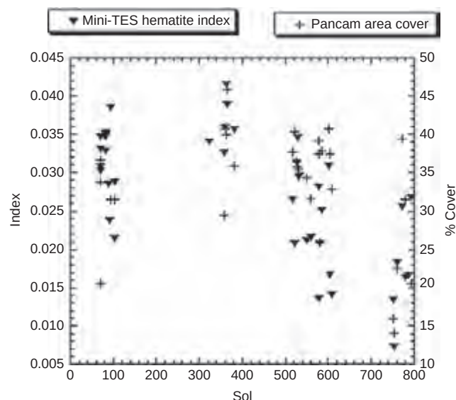
Figure 13.40. Pancam berry cover and Mini-TES hematite index with Sol.
