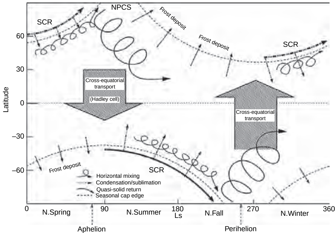
Figure 25.3. The components of the \text{H}_2\text{O} cycle, including the migration of \text{H}_2\text{O} ice along the edge of the retreating seasonal caps (Montmessin et al. , 2004). SCR: Seasonal Cap Retreat; NPCS: North Polar Cap Sublimation.
