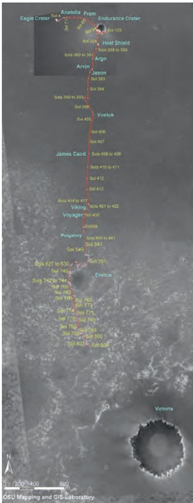
Figure 13.16. Opportunity's traverse in Meridiani Planum as of sol 810 (May 5, 2006). (Base map from MGS/MOC [NASA/JPL/MSSS]. Traverse mapping by T. Parker, R. Li, and the MER/Athena Science Team.) (For a color version of this figure, please refer to the color plate section or to the e-Book version of this chapter.)
