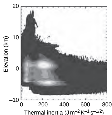
Figure 18.13. A 2D histogram of TES-based nighttime thermal inertia (Figure 18.8a) and MGS MOLA elevation (see Putzig, 2006). Shades of gray indicate frequency of occurrence. Over most of Mars high and low thermal inertia values occur at all elevations. Exceptions are that the highest elevations (mountain peaks) are dominated by lower thermal inertia values and that the lowest elevations are dominated by higher thermal inertia values. See text for additional discussion. Histogram bin sizes are 400 m for elevation and 5 for thermal inertia. Levels are 1 occurrence and 1/20, 1/10, 1/5, 1/3, and 1/2 of the maximum frequency.
