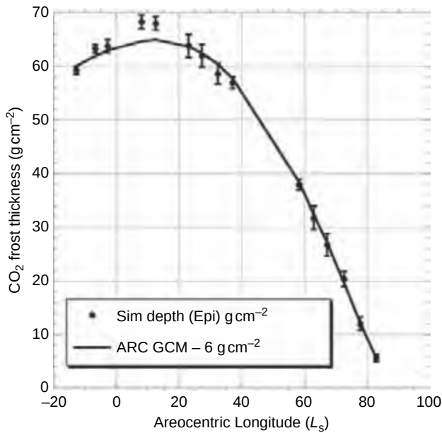
Figure 6.2. Comparison between the CO 2 frost thickness as a function of season poleward of +85° latitude and the calibrated simulation of those thicknesses using measured epithermal neutron counting rates.
