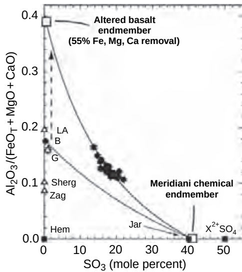
Figure 24.12. Plot of molar (\text{Al}_2\text{O}_3/(\text{FeO}_T + \text{MgO} + \text{CaO})) versus \text{SO}_3 for the abraded portions of the Burns formation outcrop. Also plotted are the compositions of Martian meteorites (LA – Los Angeles; Sherg – Shergotty; Zag – Zagami), Martian surface basalts (B – Bounce Rock; G – Gusev crater plains basalts), selected mineral compositions (Hem – hematite; Jar – jarosite; various Ca-, Mg- and \text{Fe}^{2+} -sulfates as \text{X}^{2+}\text{SO}_4 ). The composition of the Burns formation is consistent with mixing between an “altered” Martian basalt and a chemical endmember consisting of a variety of sulfate minerals and hematite. Variations in the Burns formation composition are in part stratigraphically controlled ( \text{SO}_3 decreases down section) and result mainly from variations in Mg and Al and are interpreted to be due to diagenetic redistribution of soluble salts (e.g., Clark et al. , 2005). (Adapted from Squyres et al. , 2006a.)
