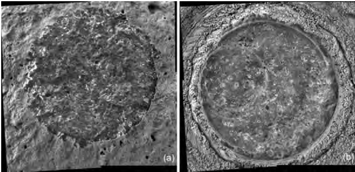
Figure 20.17. Spirit MI mosaics of target “Chisel” on rock “Wishstone” before (a) acquired on Sol 333 and after (b) acquired on Sol 334) RAT grinding. Each mosaic is about 5 cm across; all images taken while target was fully shadowed.
