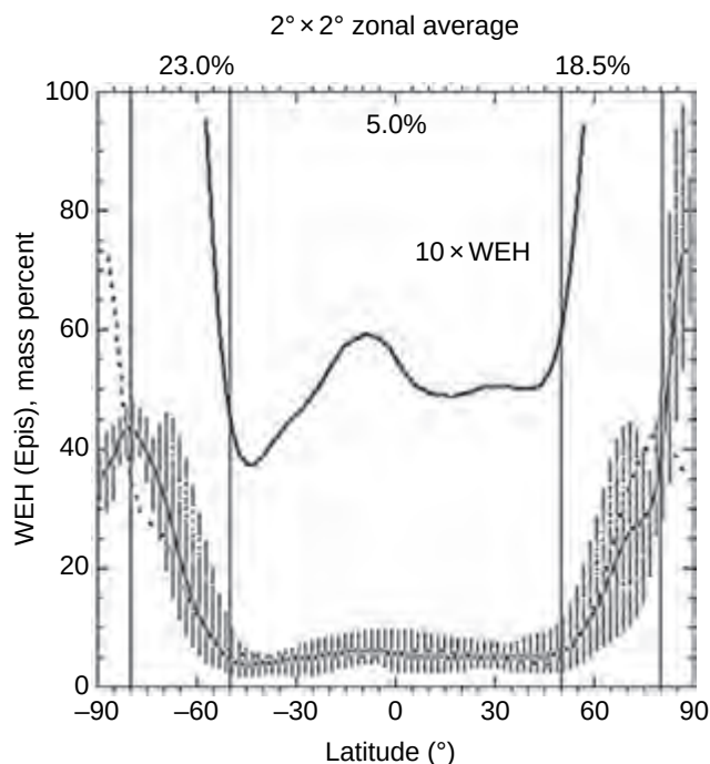
Figure 6.9. 2^\circ \times 2^\circ zonal averages of WEH abundance calculated using Prism 1 epithermal neutron counting rates. See the text for details.
