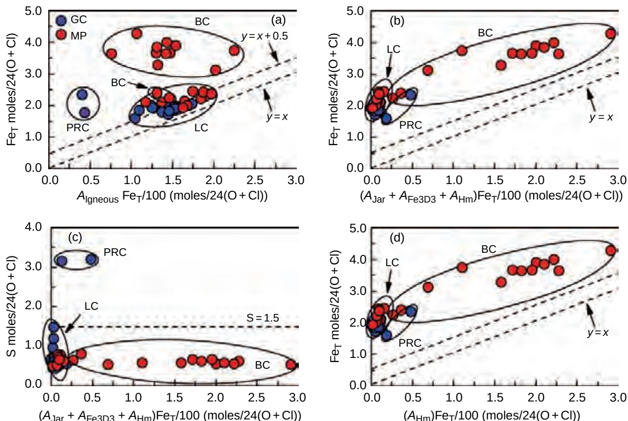
Figure 15.7. Diagrams for assignment of MER soil samples to supergroups (Laguna Class soil, Paso Robles Class soil, and Berry Class soil). (a) \text{Fe}_T versus A_{\text{Igneous}}\text{Fe}_T/100 . Soils form into Laguna Class (LC), Paso Robles Class (PRC) and Berry Class (BC) supergroups, except for two BC soils that have LC affinities. (b) \text{Fe}_T versus (A_{\text{Jar}} + A_{\text{Fe3D3}} + A_{\text{Hm}})\text{Fe}_T/100 . BC soils are distinguished from LC soils. (c) S versus (A_{\text{Jar}} + A_{\text{Fe3D3}} + A_{\text{Hm}})\text{Fe}_T/100 . The three soil supergroups form into different regions. LC and BC supergroups have S concentrations within the range for Altered Low-S Rock (Figure 15.6c). PRC soils at Gusev crater have the highest S concentrations measured on Mars. (d) \text{Fe}_T versus A_{\text{Hm}}\text{Fe}_T/100 . Soils do not have detectable concentrations of Jar and Fe3D3 (compare with (b)). (For a color version of this figure, please refer to the color plate section or to the e-Book version of this chapter.)
