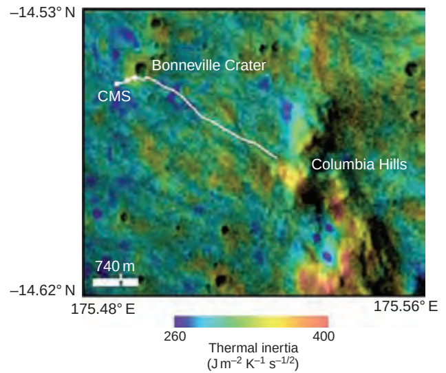
Figure 21.19. THEMIS thermal inertia image in color (100 m/pixel) overlaid on THEMIS visible mosaic (18 m/pixel) of the Gusev crater landing region. Spirit landed at Columbia Memorial Station (CMS) in a low albedo, low thermal inertia intercrater plains (southwestern-most white dot: Mission Success panorama location), traversed through the ejecta blanket (middle white dot: Legacy panorama location) to the rim of Bonneville crater about 300 m away (northeastern-most white dot), and then across the low and high thermal inertia plains to the Columbia Hills (with generally higher inertias) to the east and southeast. Thermal inertia (Ferguson and Christensen, 2006b) increases from 285 to 330 \text{ J m}^{-2} \text{ K}^{-1} \text{ s}^{-1/2} over the traverse to the rim of Bonneville crater. Rock size frequency distributions are reported at these three locations in Figure 21.12.
