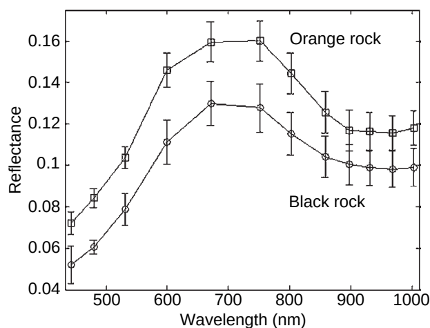
Figure 12.3. Orange and Black Rock spectra. Orange Rock spectrum from SuperPan octant S0188 referenced by Murchie et al. (2000). Black Rock spectrum from SuperPan octant S0184 (corresponds to Merényi et al. [2004] class O).
