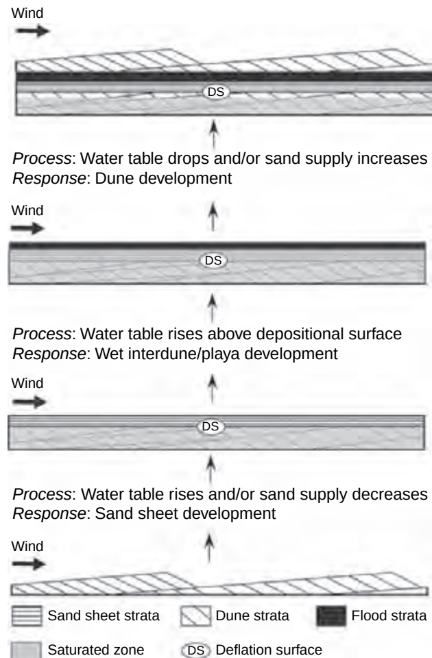
Figure 24.11. Depositional model for the Burns formation in the region of Eagle and Endurance craters (from Grotzinger et al. , 2005) documenting a “wetting upward” eolian system. The lower unit accumulates by migration of eolian dunes composed of sulfate-cemented altered basalt sand grains. Elevation of the water table (or decrease in sediment flux) results in the formation of a deflation surface (DS) down to the level of the capillary fringe of the water table. Sand sheet strata are deposited above the deflation surface. At some point, the groundwater table breaches the surface, resulting in deposition of subaqueous interdune sandstones (“Flood Strata”). To date, only one such cycle has been confirmed by Opportunity , but such a model predicts that the cycle would be repeated as the level of the groundwater table fluctuated.
