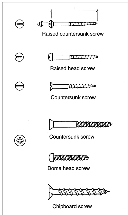
Figure 17.3: Standard wood screws.
