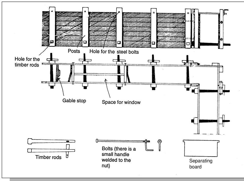
Figure 13.19: Swedish model for shuttering. Source: Lindberg 1950
