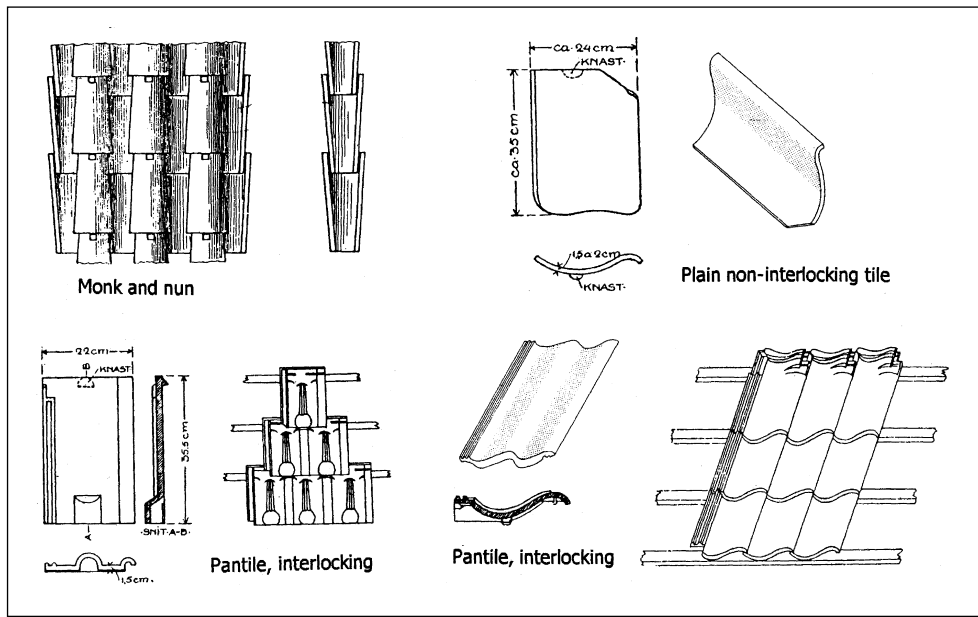
Figure 15.5: Types of roof tiling.
