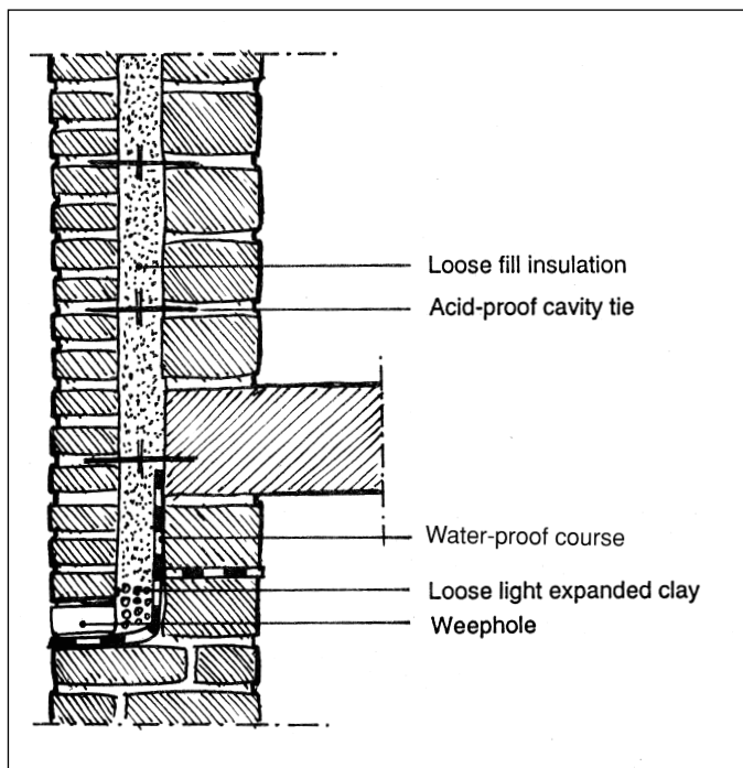
Figure 14.6: Principle for perlite insulation in cavity walls.
