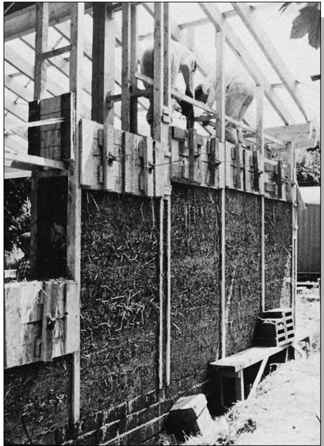
Figure 14.16: Wall construction in 'Leichtlehm'.
