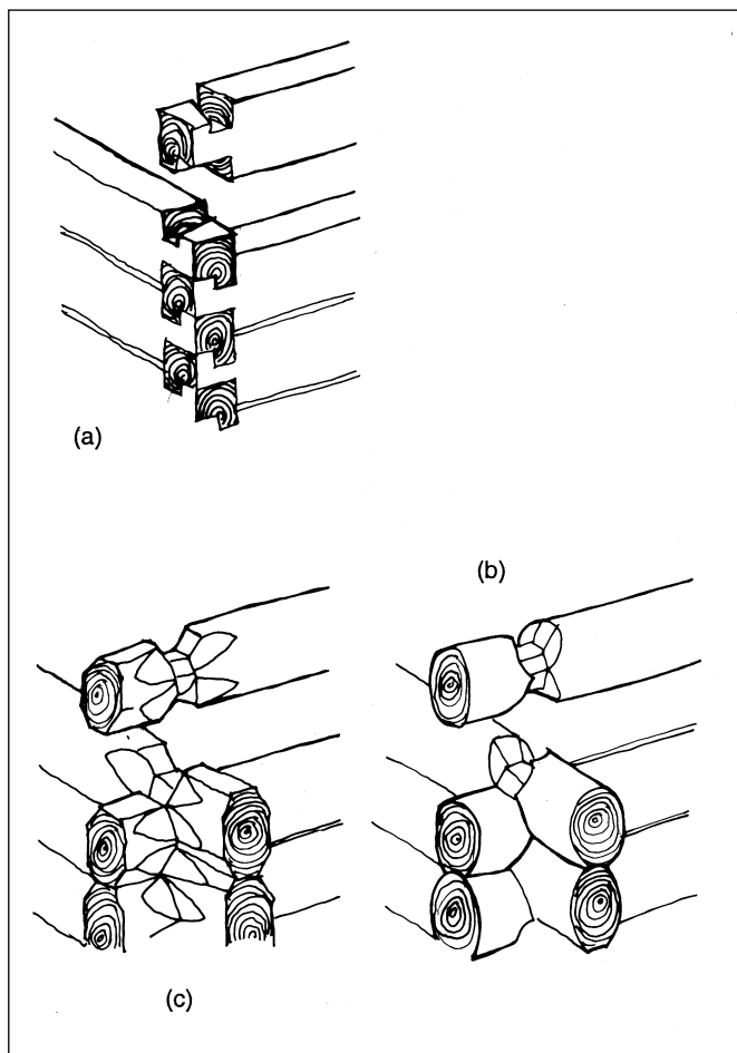
Figure 13.38: Some log joints.
