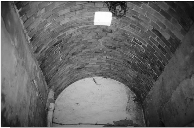
Figure 13.16: Structural vault in brick.
