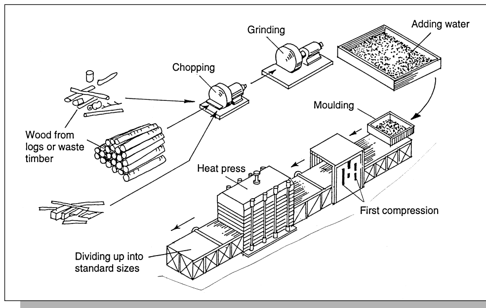
Figure 15.25: Production of hard and semi-hard wood fibreboards.
