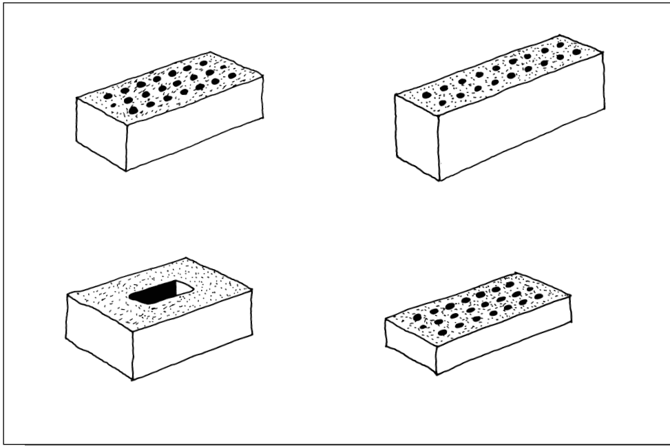
Figure 13.12: Examples of perforated bricks.
