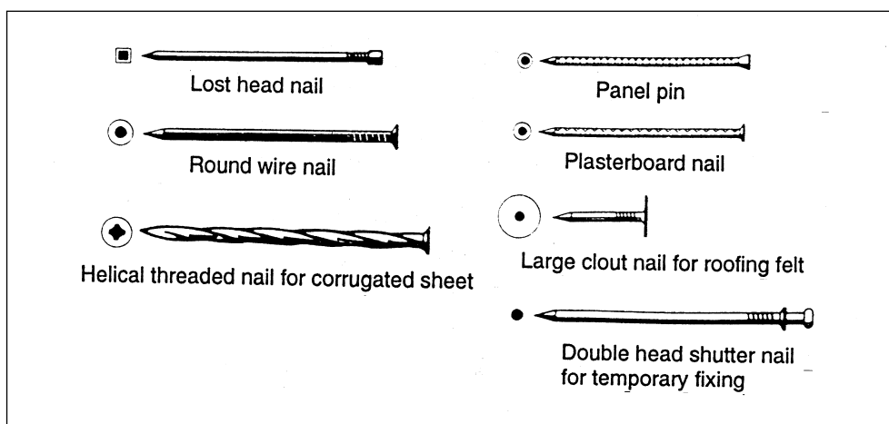
Figure 17.2: Standard nails.
