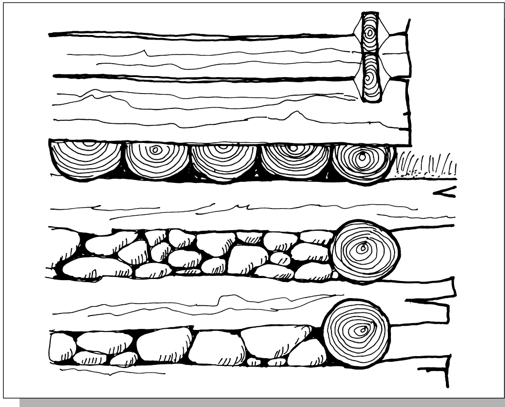
Figure 13.36: Bulwark method of foundation work. Source: Drange, 1980
