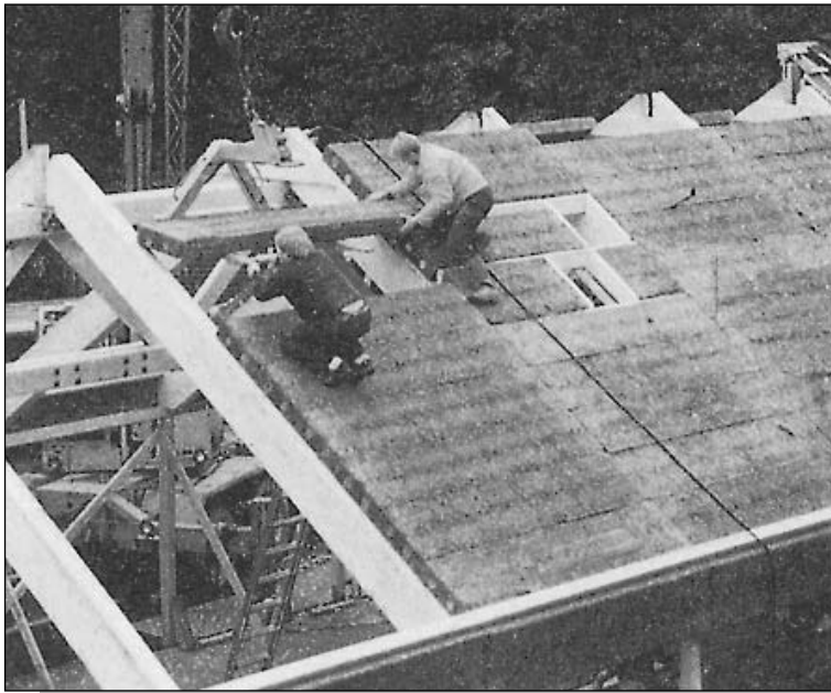
Figure 14.13: Woodwool slabs reinforced with round rods combine high thermal insulation values with structural integrity.
