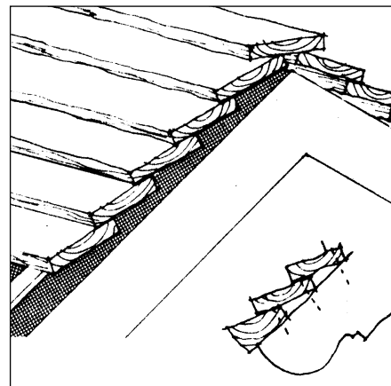
Figure 15.18: A Sutak roof. Source: Eriksen
