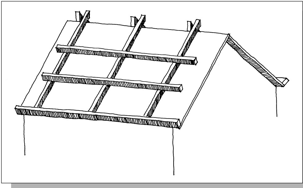
Figure 15.13: Battens for holding turf in place on steeper roofs.
