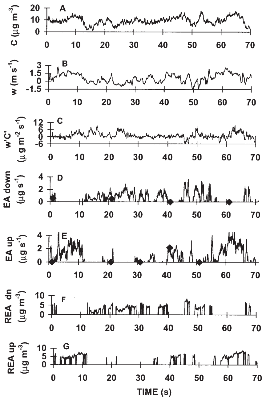
FIGURE 24.2 Fast-response measurements of trace gas concentration ( a ); vertical wind velocity ( b ); their application to eddy covariance ( c ); eddy accumulation ( d, e ); relaxed eddy accumulation ( f, g ); the points (filled diamonds) shown in d and e illustrate a periodic sampling strategy.
