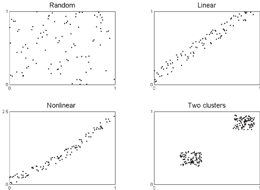
FIGURE 25.3 Scatter plots.
