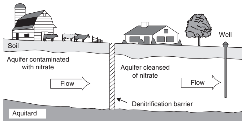
Figure 4. Hypothetical use of a denitrification barrier to remove nitrate from groundwater contaminated by farm animals.
