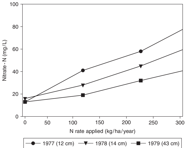
Figure 2. Nitrate-N concentration in tile drainage water as affected by N rate for continuous corn in Minnesota.
