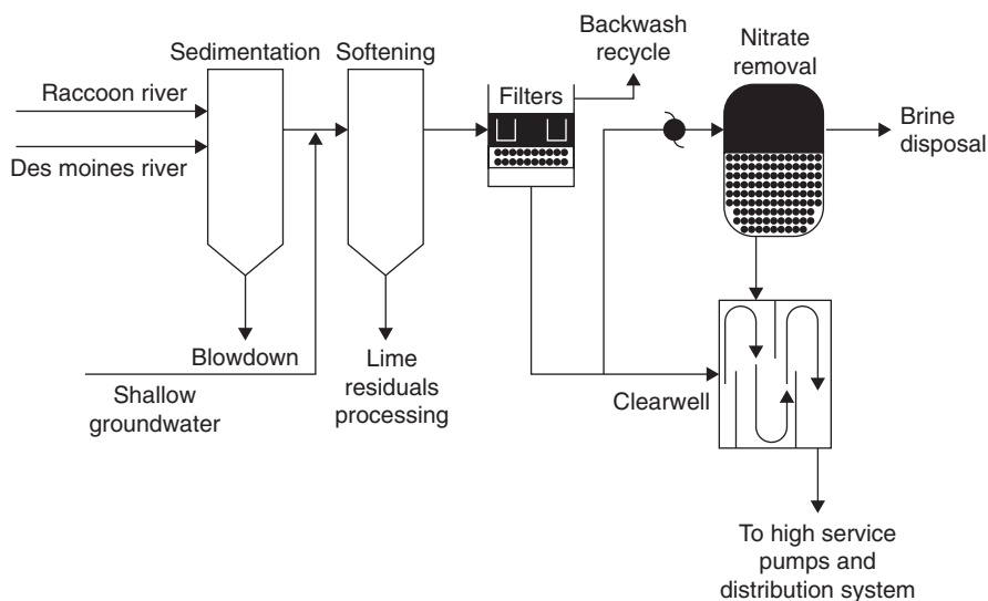
Figure 1. DMWW's treatment process.
