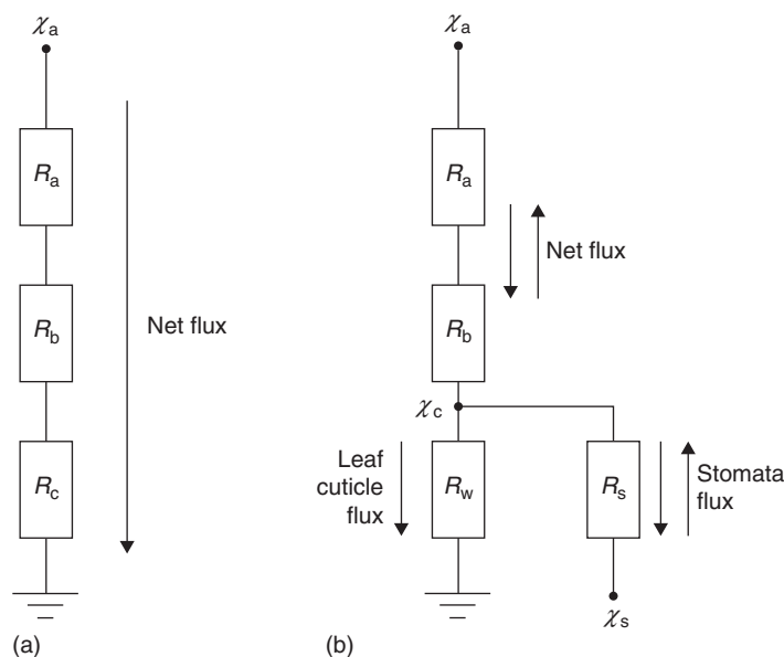
Figure 4. (a) Canopy resistance model; (b) the single-layer canopy compensation point model according to Sutton et al. (1995b). R, resistance; Subscripts: a = aerodynamic; b = boundary layer; w = leaf cuticle; and s = stomata. \chi_a , \text{NH}_3 concentration in air, \chi_s and \chi_c stomatal and canopy compensation points, respectively.
