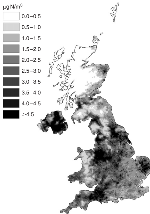
Figure 11. Surface concentration of \text{NH}_3 for the UK in 2002 (FRAME model version 5.9). Units are \mu\text{g N/m}^3 .
