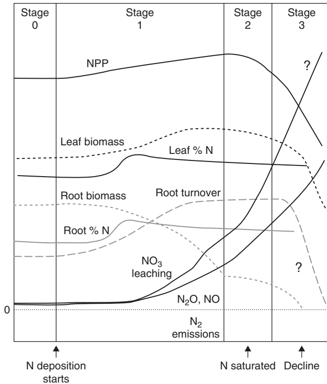
Figure 2. Conceptual model of forest biogeochemical responses to chronically elevated N deposition. Stage 0 represents pristine conditions. Stage 1 follows the onset of elevated N deposition, where N limits growth, increases in foliar and fine root N could lead to increased N concentrations and turnover rates in resource leaves and fine roots, and higher net primary production (NPP). These increases, however, might be difficult to detect, particularly at low rates of N input. Nitrate losses above background levels can occur, but they are not large. If forests advance to Stage 2, nitrate losses increase and biomass responses are more easily detected. If forest decline (Stage 3) occurs, tree mortality is high, NPP decreases, and exports of nitrate and oxidized N gases increase. Variations of lines along the y-axis indicate qualitative changes for the individual processes or properties as elevated N deposition progresses. Adapted from Aber et al. (1989, 1998) and Nadelhoffer, 2000.
