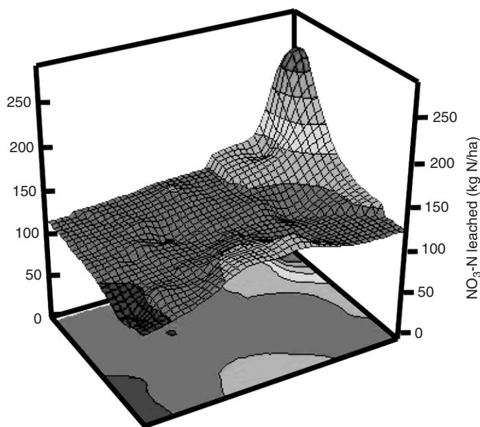
Figure 8. Spatial distribution of predicted NO 3 -N leaching from the root zone of corn (1.5 m depth) in study one across the different productivity zones during the 2000 growing season. (From Delgado and Bausch, 2005).
