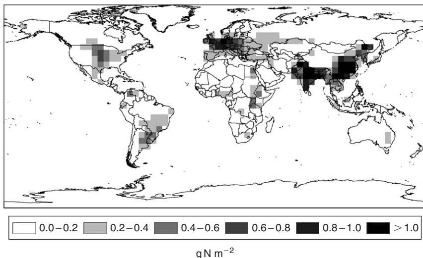
Figure 13. Global \text{NH}_3 dry deposition map for 2000, produced from output of the STOCHEM model (data courtesy of David Stevenson, Edinburgh University). Units are \text{g N/m}^2 .
