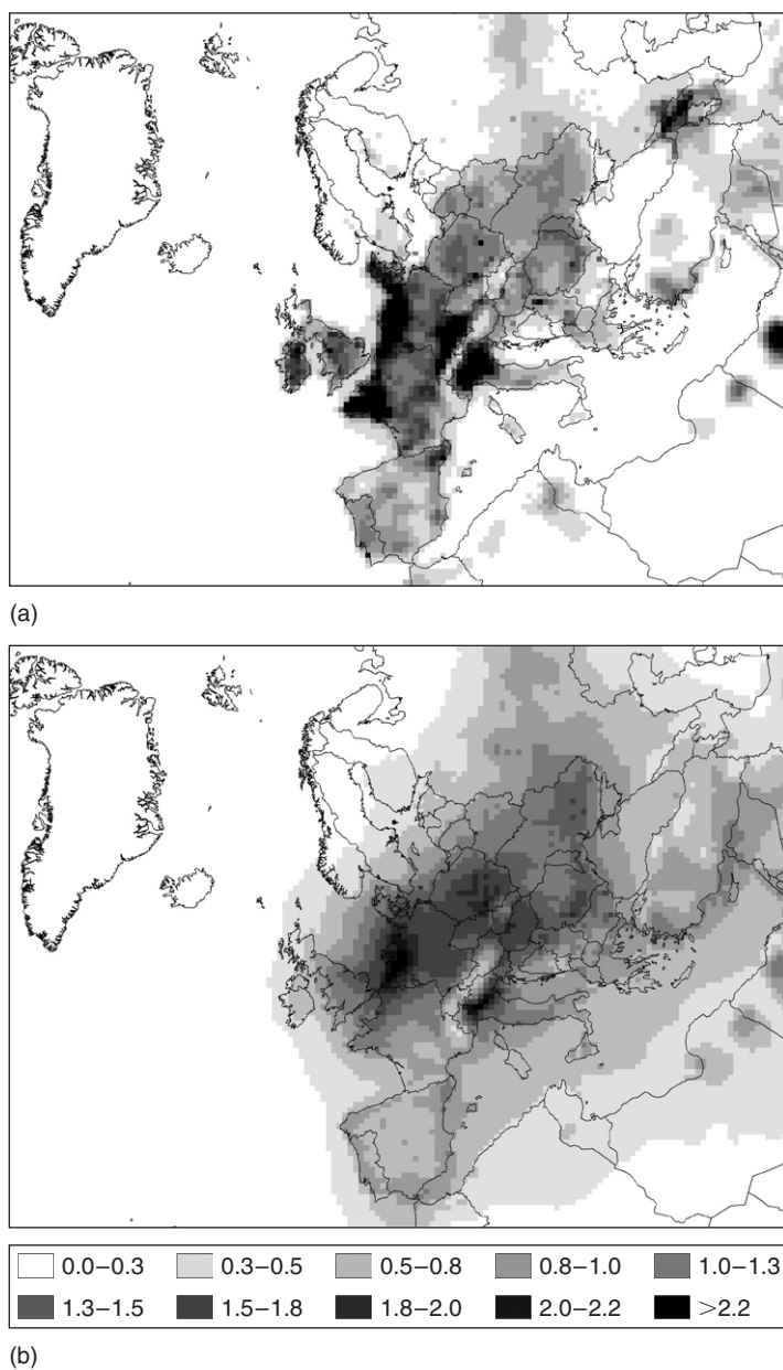
Figure 12. Predicted surface concentration for Europe in 2002: (a) Ammonia ( \text{NH}_3 ) and (b) Ammonium ( \text{NH}_4^+ ), calculated with the EMEP Unified model (data courtesy of David Simpson, Norwegian Meteorological Institute). Units are \mu\text{g N/m}^3 .
