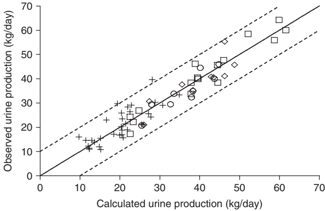
Figure 4. Comparison between measured and calculated urine production by lactating dairy cows. Calculated values were obtained from regression analysis, according to: urine production (kg/day) = 0.134 (0.010) \times urinary excreted sodium (g/day) + 0.061 (0.005) \times urinary excreted potassium (g/day) + 0.024 (0.007) \times urinary excreted N (g/day) ( R^2 = 0.898 , SE = 4.22 kg/day) (Bannink et al., 1999).
