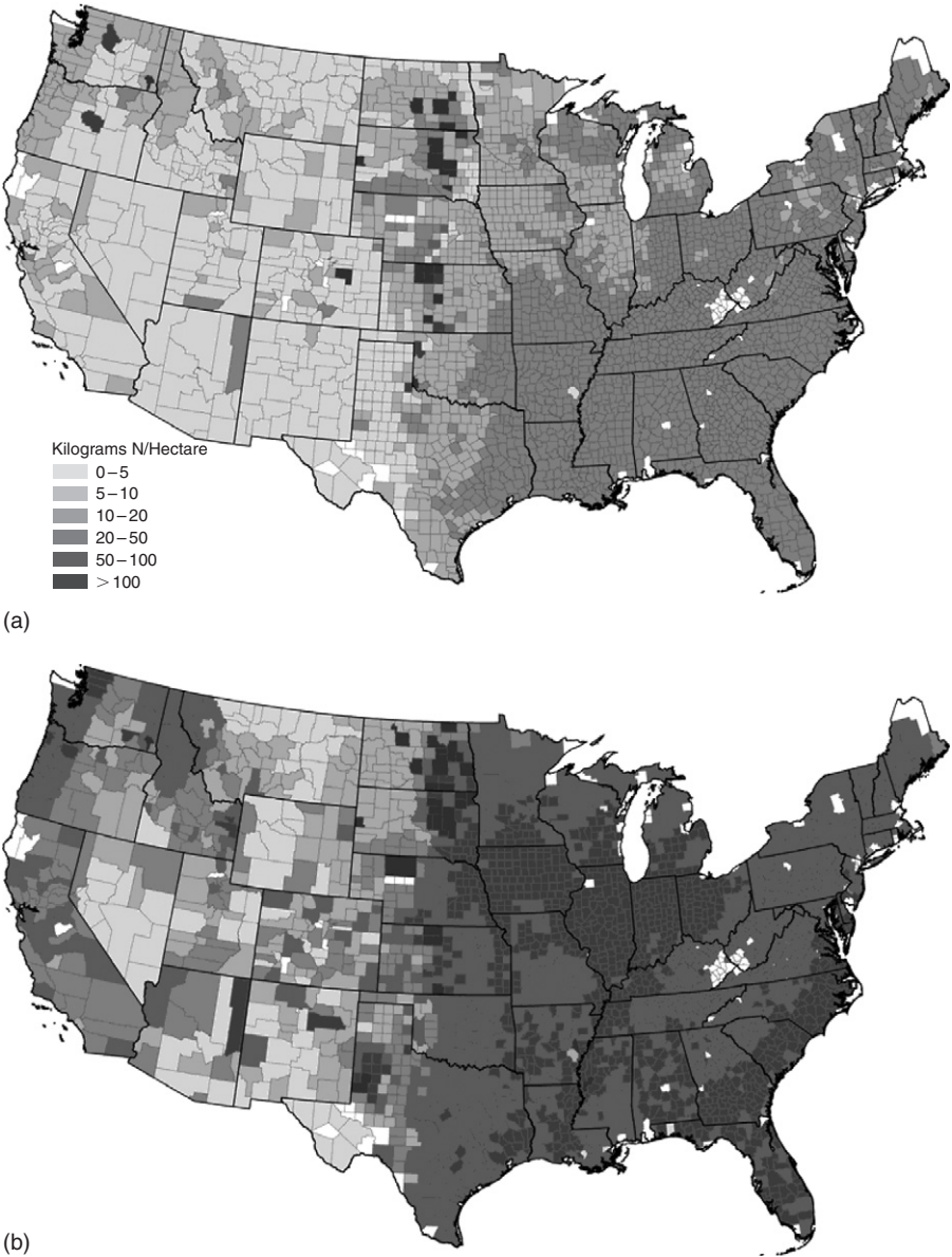
Figure 5. DAYCENT simulated county level mean N losses from \text{NO}_3 leaching and N gas emissions ( \text{NH}_3 , \text{NO}_x , \text{N}_2\text{O} , \text{N}_2 ) for (a) potential native vegetation and (b) croppeds/grazed land area weighted means. Values are annual means for 1990–2003.
