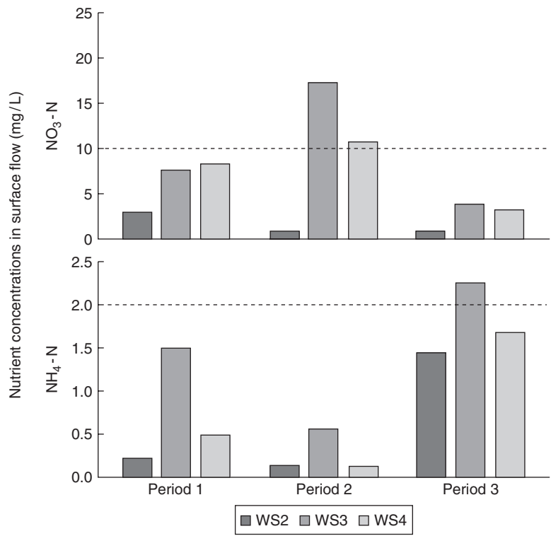
Figure 3. Runoff-weighted concentrations of \text{NO}_3^- -N and \text{NH}_4^+ -N in surface flow by seasonal period. Dashed lines represent current water quality standards. (From Alberts and Spomer, 1985).
