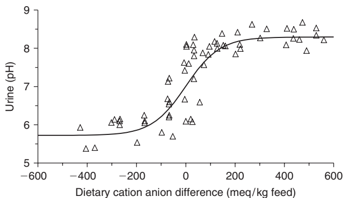
Figure 5. The relationship between dietary cation–anion balance ( \text{Na} + \text{K} - \text{Cl}^{-2} \times \text{S} in meq/kg feed dry matter) and the pH of urine excreted by dairy cows. The following relationship was derived by regression of a logistic equation to observed data: \text{Urine pH} = 5.72(0.17) + 2.57(0.29)/[1 + \exp(-0.015(0.004) \times (\text{cation–anion balance})] R^2 = 0.692 ; \text{SE} = 0.612 (Bannink and van Vuuren, 1998).
