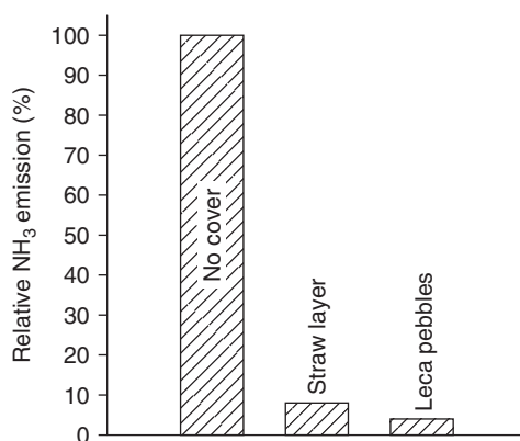
Figure 7. Decrease in \text{NH}_3 losses following the covering of slurry storage systems, in percent (after Sommer, 1997).
