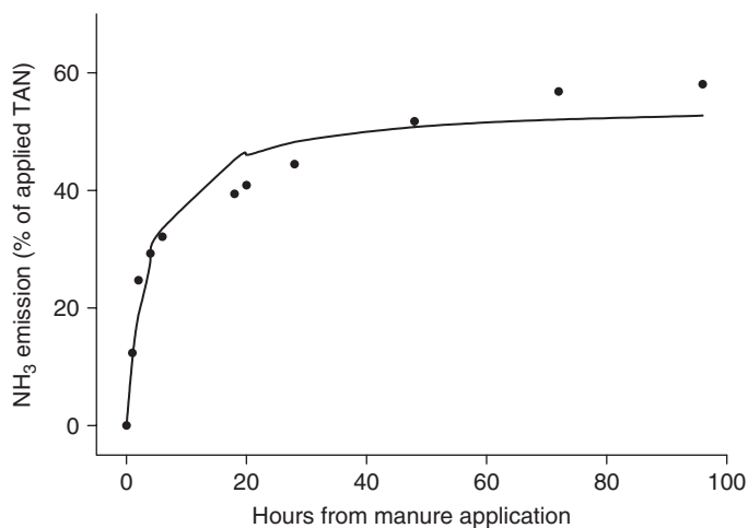
Figure 9. Pattern of \text{NH}_3 volatilization following surface application of pig slurry to arable land on top of stubble, in percent of the total amount of ammonium N (TAN) in the slurry (after Bless et al., 1991).
