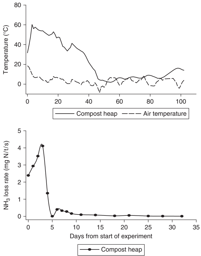
Figure 8. Air temperature and manure temperature (upper panel) and the NH 3 loss from the manure (lower panel). Note differences in scale of X-axes: upper panel 0–100 days and lower panel 0–35 days. The increase in NH 3 loss during the first four days (lower panel) coincides with the rise in temperature of the manure (upper panel).
