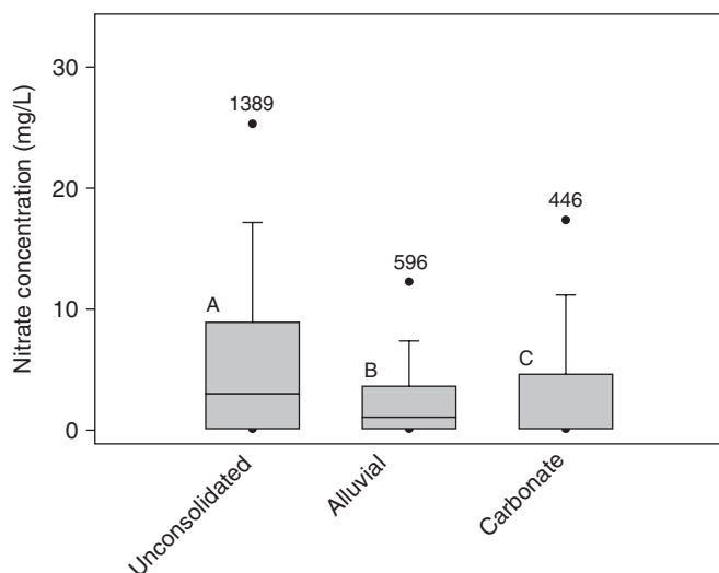
Figure 11. Nitrate concentrations grouped by shallow aquifer types.
