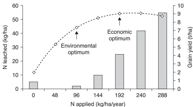
Figure 2. A nitrogen response curve and corresponding leaching losses from the 160-year-old Broadbalk Experiment at Rothamsted.
