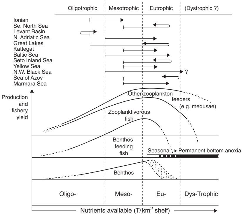
Figure 11. A speculative concept of fisheries change with nutrient enrichment. Redrawn from Caddy (1993). A qualitative progression was suggested from a review of patterns in different enclosed and semi-enclosed seas. The recent trajectory of different systems with respect to trophic status is indicated at the top. The bottom suggests a progression of change in the structure of food webs and composition of fisheries prior to a dramatic loss of yield with permanent bottom anoxia.
