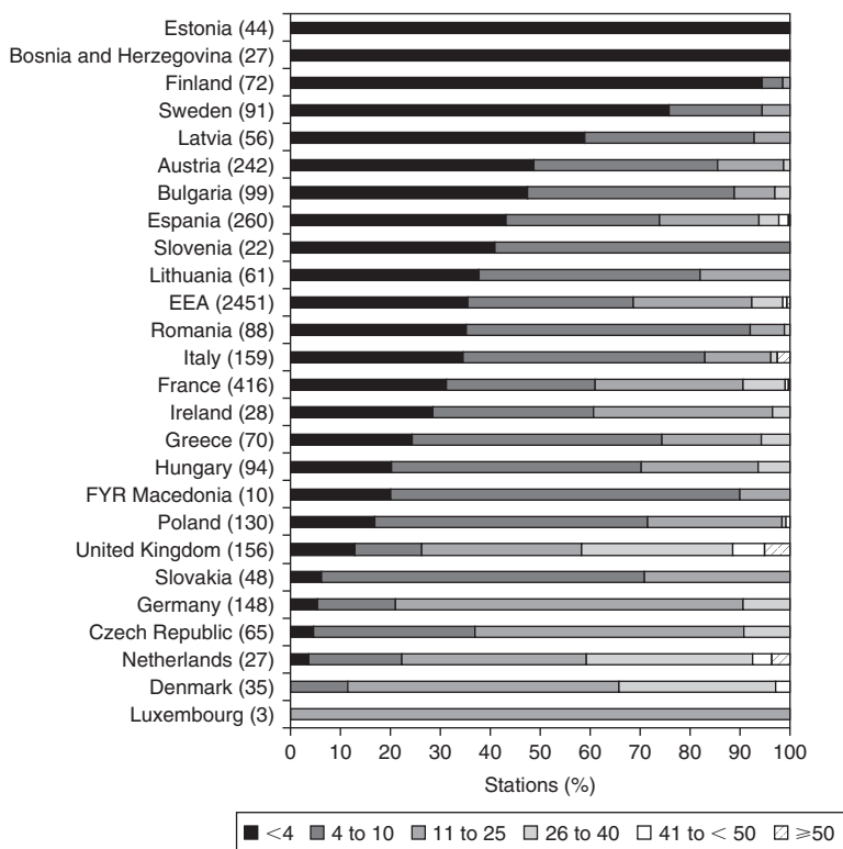
Figure 2. Concentrations of nitrate (mg nitrate per liter) at monitoring stations in European rivers shown in concentration classes. The number of monitoring stations within each country is given in the bracket following the country name. (Data from European Environment Agency, 2005b)
