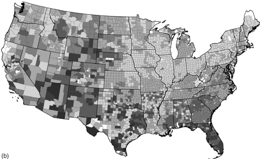
Figure 7. DAYCENT simulated county level mean \text{NO}_x/\text{N}_2\text{O} ratios for (a) potential native vegetation and (b) cropped/grazed land area weighted means. Values are annual means for 1990–2003.
