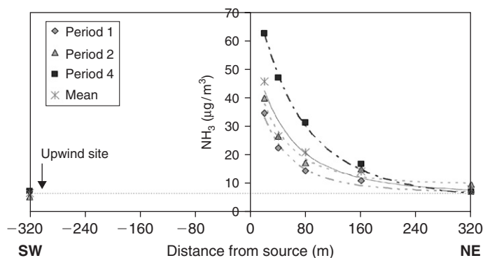
Figure 8. Monitored \text{NH}_3 concentrations along the SW-NE transect at a poultry farm with natural ventilation for three 6–8-week bird cycles. Data from Tang et al. (2005).
