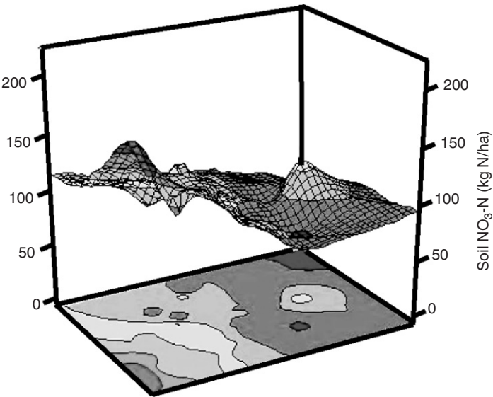
Figure 7. Spatial distribution of observed residual soil NO 3 -N in the top 1.5m of soil for study one across the different productivity zones during the 2000 growing season. (From Delgado and Bausch, 2005).
