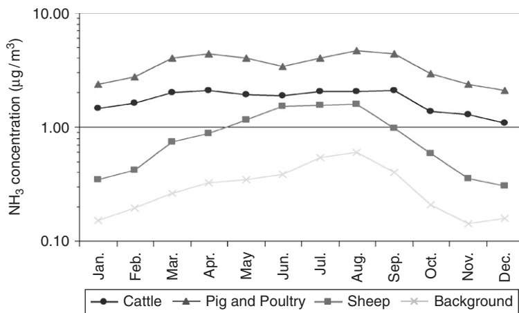
Figure 7. Seasonal profiles of NH 3 concentrations from the mean data (1996–2005) of sites in the NAMN classified by different dominant emission categories: cattle, sheep, pig and poultry and background.
