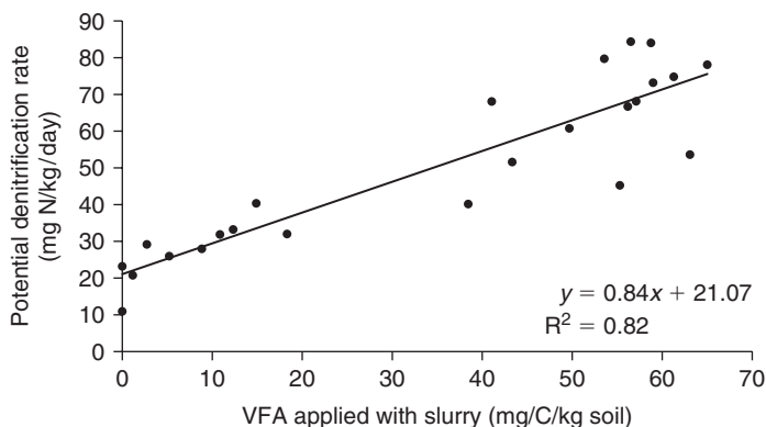
Figure 10. Relationship between the amount of volatile fatty acids (VFA) applied with pig slurry to a sandy soil and potential denitrification. Differences in contents of VFA between slurries were created by differences in diet offered to the pigs (Velthof et al., 2005) and by digestion (Velthof, unpublished results). The potential denitrification is defined as the maximum rate at which nitrate is reduced under anaerobic conditions at 20°C.
