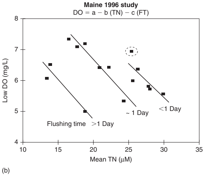
Figure 8b. Relationship observed among N concentrations, minimum DO concentrations, and flushing time for 15 small, short-residence time, tidally flushed estuaries and embayments. Adapted from Kelly, 1997c, in which stepwise multiple regression analyses selected TN and flushing as first-order explanatory variables accounting for >60% of the variability. One point (circled) did not fit the trend. Flushing time is based on replacement of estuarine volume by tidal volume input every 12.42h, and as such assumes complete mixing. Freshwater replacement time is much slower; these systems generally have low Fw/tidal volume ratios (see Figure 3a).
