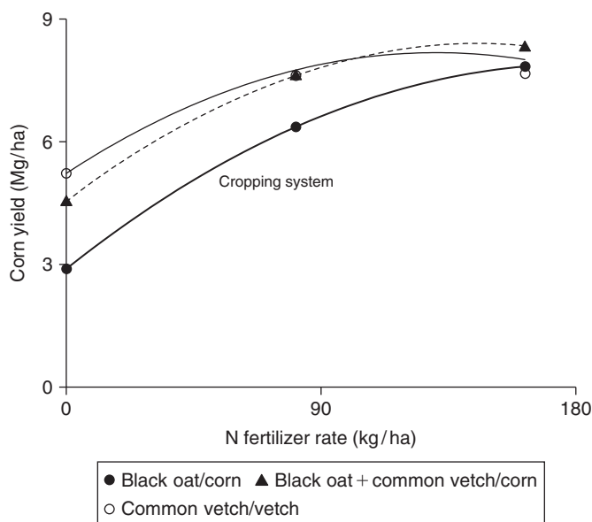
Figure 6. Nitrogen fertilizer (urea) effect on corn yield in different cropping systems in Rio Grande do Sul, state. (Amado et al., 1999).
