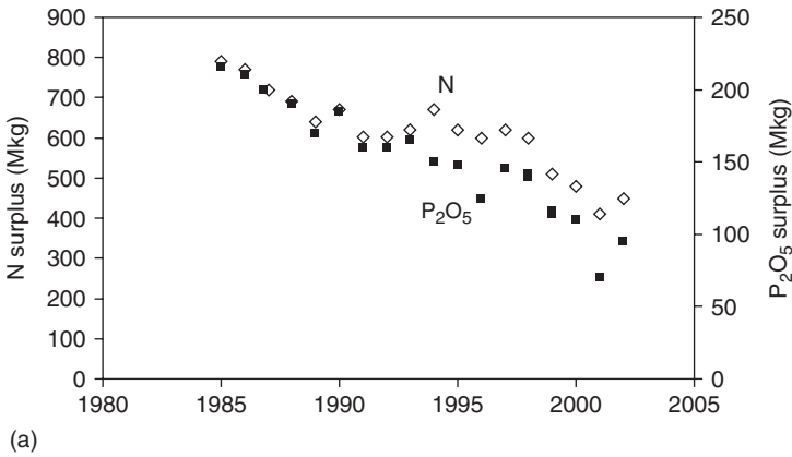
Figure 3a. Total nitrogen (N) and phosphorus (as P_2O_5 ) surpluses in the Netherlands from 1985 to 2002. In 2002 the average surpluses were 130kg N per hectare and 28kg P_2O_5 per hectare (Goulding et al., 2006).
