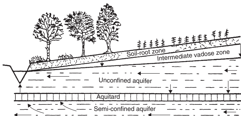
Figure 7. Schematic of the vadose zone, aquifers, and flow directions in a typical riparian zone subject to a humid climate. (From Pionke and Lowrance, 1991).
