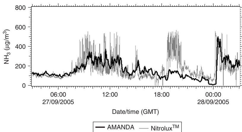
Figure 10. Comparison of field measurements of \text{NH}_3 close to an agricultural source, using a continuous wet ADS (AMANDA, ECN, NL) and a photo-acoustic monitor (NitroLux-100, Pranalytica Inc., CA, USA), both as 5-min averages (M. Twigg and E. Nemitz, unpublished data, CEH Edinburgh).
