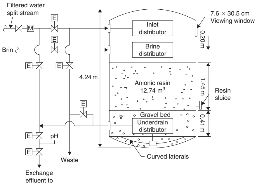
Figure 4. Detailed view of ion exchange vessel and header piping.
