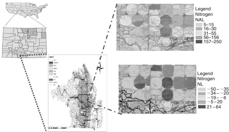
Figure 9. Mass balance for N available to leach and nitrate leaches in an area of a region.
