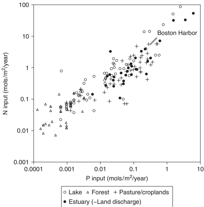
Figure 2. Nitrogen and phosphorus input to a variety of terrestrial and aquatic ecosystems. Modified from Kelly and Levin (1986). Estuarine systems show DIN or TN input from land and in some cases, atmosphere. Boston Harbor is from land-derived sources only (Kelly, 1997a), showing an example range for a system considering only DIN (lower end of bar) or TN (upper end of bar).
