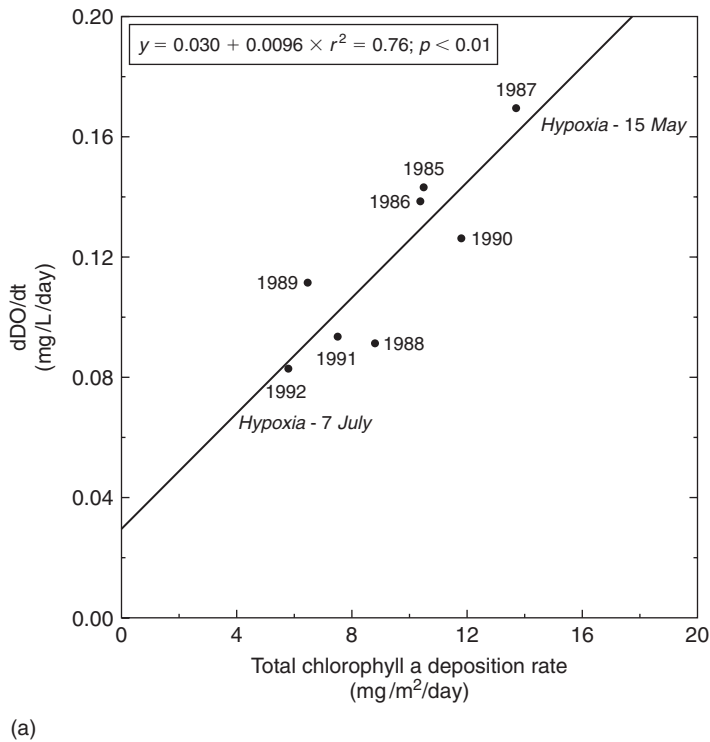
Figure 8a. Empirical relationship between spring organic matter input and summer seasonal DO decline rates in bottom-water at a site in the mainstem of Chesapeake Bay. Redrawn from Boynton and Kemp (2000). The date at which hypoxia (as DO <1 mg/L) was first encountered in years with highest and lowest organic matter is indicated.
