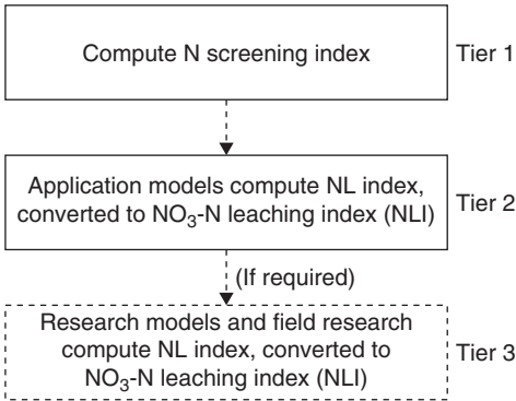
Figure 3. Tier structure of proposed \text{NO}_3^- -N leaching index (NLI). (From Shaffer and Delgado, 2002).
