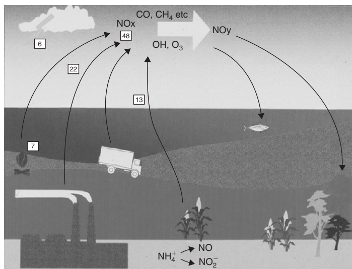
Figure 7. A cartoon depiction of the terrestrial-atmosphere exchange of NO_x and deposition of NO_y (adapted from Williams et al., 1992; Mosier, 1998).
