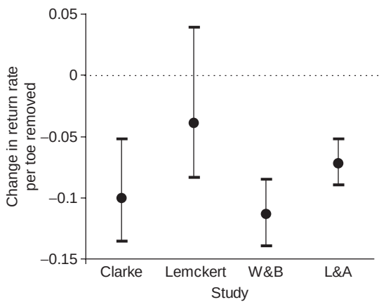
Fig. 7.5. Predicted change in return rate of frogs for each toe removed for four different studies (Clarke, 1972; Lemckert, 1996; Williamson and Bull, 1996; Lüddecke and Amézquita, 1999). The circle is the best estimate of the effect and the bars represent 95% confidence intervals. Negative values represent an adverse effect of toe clipping. Reproduced from McCarthy and Parris (2004).
