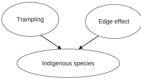
Fig. 31.1. A basic conceptual model of the anticipated effects of trampling and habitat edges on the indigenous biota in urban environments, as described in Grandchamp et al. (2000) and Lehv virta et al. (2006).
