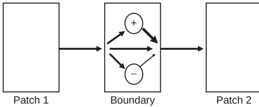
Fig. 3.2. A general template for models examining the structure and function of ecological boundaries. Any model of boundary function would minimally have to identify the contrasting areas or patches separated by the boundary, the kind of flux across the boundary, and the ability of the boundary to control the flow. Modified from Cadenasso et al. (2003b).
