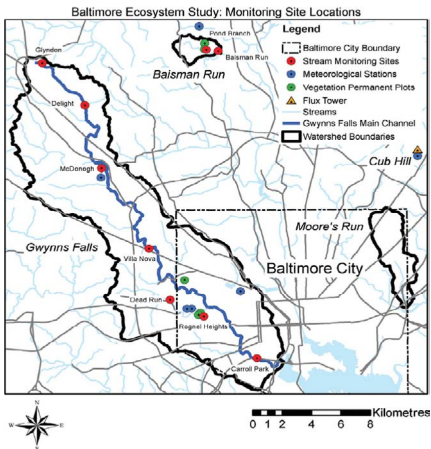
Plate 3.5. Sampling sites for the Baltimore Ecosystem Study, based on major watersheds. Watersheds are used as integrators, and reflect different degrees of urbanisation. The Baisman Run watershed contains Pond Branch, which serves as a forested reference for the project. Different kinds of sampling plots or facilities are identified across the urban landscape.
