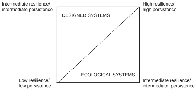
Fig. 28.2. The dual identity of urban riparian landscapes as designed and ecological systems.
