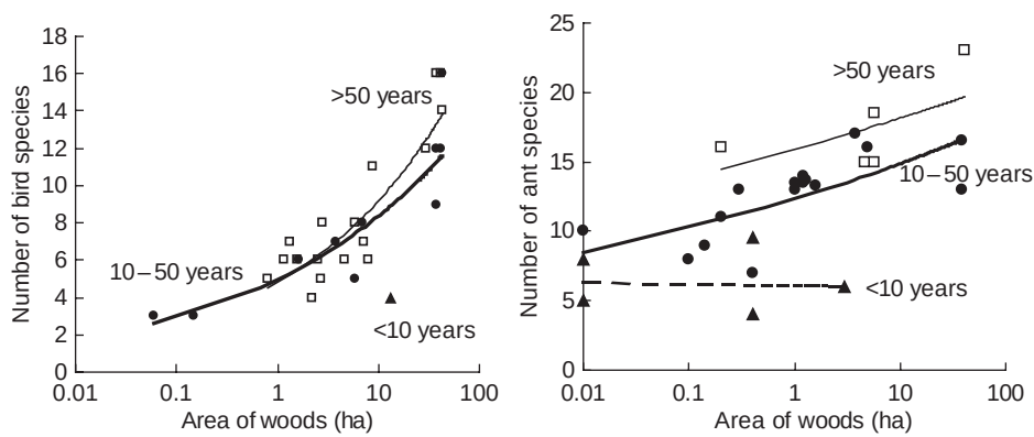
Figure 12.2. A comparison of species–area curves between birds and ants in Osaka, Japan. Symbols indicate years after plantation of forests: squares and thin lines, more than 50 years; circles and thick lines, 10–50 years; triangles and broken lines, less than 10 years.
