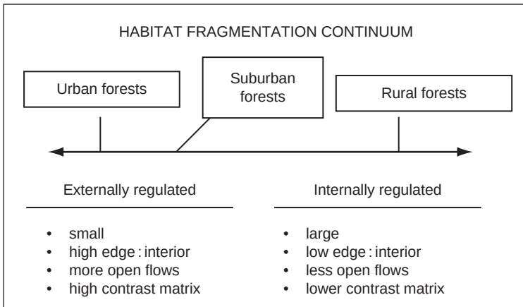
Fig. 19.1. Urban and suburban forest remnants are smaller than rural forest counterparts resulting in their having higher edge-to-interior ratios. For urban forests, proportionately greater edge length would therefore be in contact with the matrix, permitting more open and frequent exchanges of species, matter and energy between forest and matrix. Since urban matrix conditions differ markedly from most rural matrix types and forests in species composition, atmospheric chemistry and thermal regime, the intensity and type of flows is accentuated. Both higher edge-to-interior ratios and the high contrast matrix increase the potential for surrounding conditions to regulate ecological processes inside small, urban forests. Ecological processes, such as decomposition, primary production and population dynamics, in larger forests with less edge in contact with their surroundings are more likely to be regulated by internal factors.
