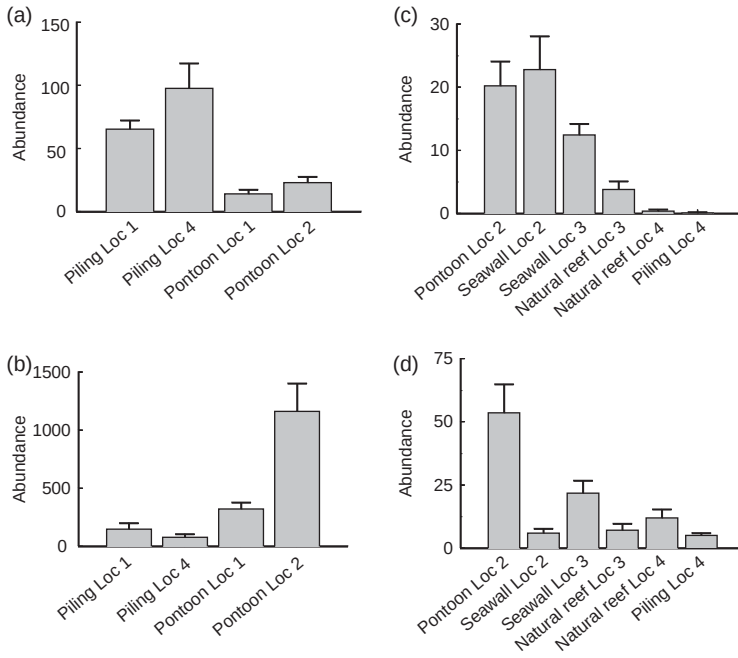
Fig. 9.3. Mean abundances (S.E.) of (a) isopods; (b) amphipods; (c) nemerteans and (d) syllid polychaetes from mussel-beds on different types of urban structures in different locations in Sydney Harbour. For all comparisons n = 10 except for natural reefs in Location 3 where n = 9 .
