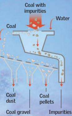
WASHING AND CLASSIFICATION BUILDING
