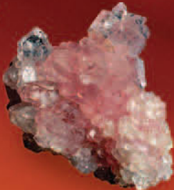
ROSE The presence of manganese results in a pink color.
