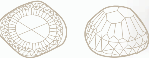
ORIGINAL CUT It formerly weighed 186 carats with 30 facets that merged into six facets, which, in turn, became one. This explains its name: Mountain of Light.
