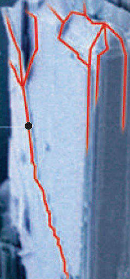
COLOR Some tourmaline crystals can have two or more colors.
