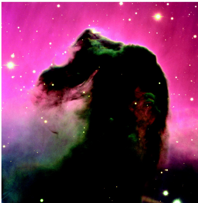
The Horsehead Nebula , imaged by the 8.2-m KUEYEN Telescope of the European Southern Observatory.
