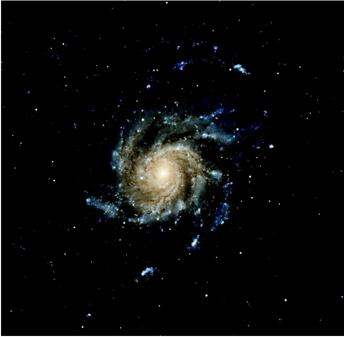
The Pinwheel Galaxy .
