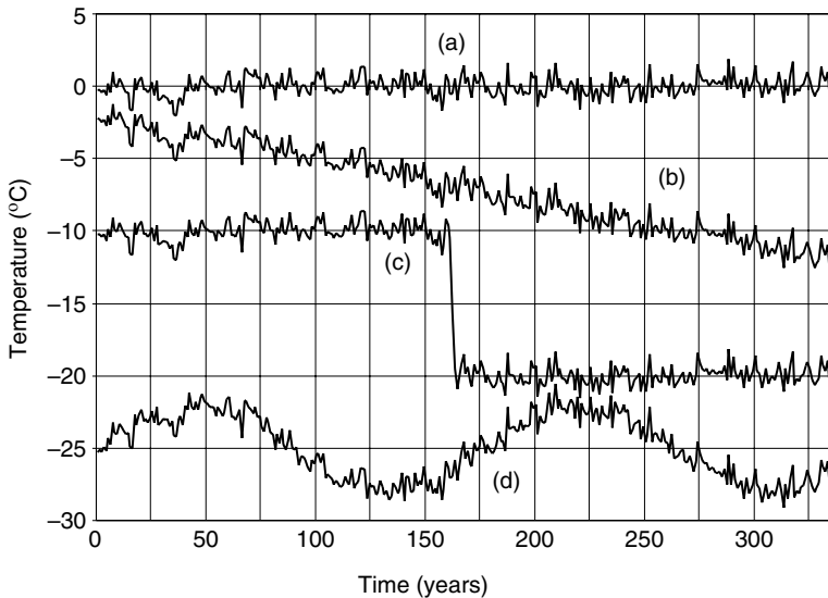
FIGURE 2.1 The definition of climate variability and climate change is most easily presented by considering a typical set of temperature observations which show (a) climate variability without any underlying change in the climate; (b) the combination of the same climate variability with a linear decline in temperature of 10^{\circ}\text{C} over the period of the observations; (c) the combination of climate variability with a sudden drop in temperature of 10^{\circ}\text{C} during the record, with the average temperature otherwise remaining constant before and after the shift; and (d) the combination of climate variability with a periodic variation in temperature of 6^{\circ}\text{C} . Successive records are displaced by an appropriate amount to enable a comparison to be made more easily.
