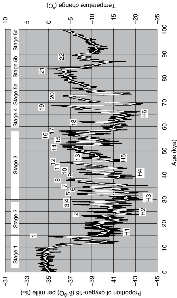
FIGURE 2.6 The record of the proportion of oxygen-18 ( \delta^{18}\text{O} ) per thousand (‰) in the GISP2 ice core (the black line is the data average values for every 50 years and the white line is the 41-term binomial smoothing of these data). These curves show the 20 Dansgaard/Oeschger warming events (labelled 1 to 20), six of which combined with Heinrich events (labelled H1 to H6). The temperature range covered by these changes is reckoned to be about 20^\circ\text{C} between the coldest periods and the warmth of the last 10 kyr. The various Oxygen Isotope Stages identified in the ocean-sediment core analysis are shown at the top of the diagram. [Data archived at the World Data Center for Paleoclimatology, Boulder, Colorado, USA.]
