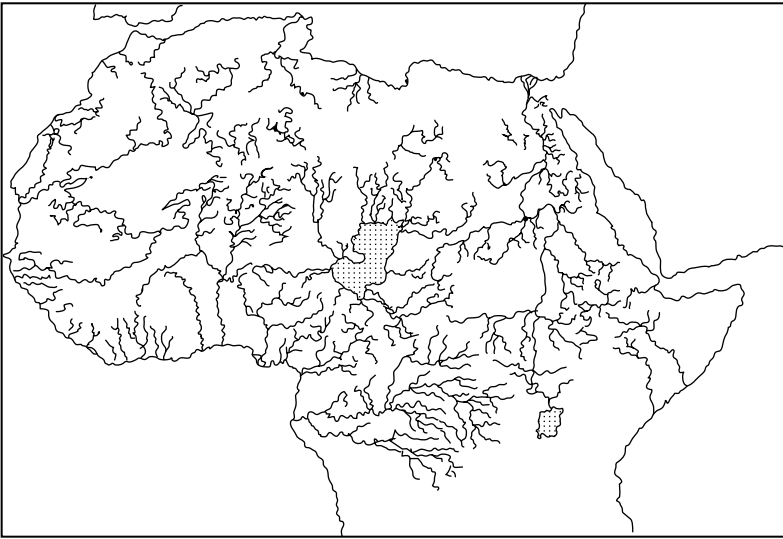
FIGURE 5.5. Map of northern Africa showing the more extensive river systems around the Sahara and greatly expanded Lake Chad.
