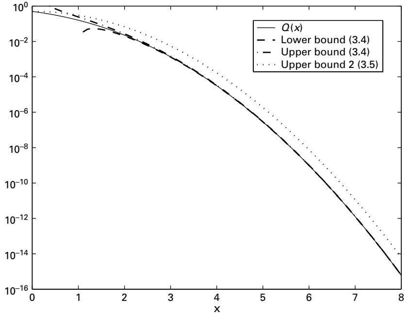
Figure 3.4 The Q function and bounds.
