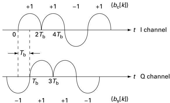
Figure 8.14 MSK interpreted as offset QPSK using a sinusoidal pulse. The I and Q channel symbols are offset by T_b , as shown.
