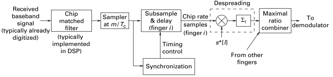
Figure 8.8 Digital-signal-processing-centric implementation of the rake receiver. The output of the chip matched filter is sampled faster than the chip rate. The synchronization circuit provides the timing control required to select a chip rate substream of samples, together with an appropriate delay, before despreading.
