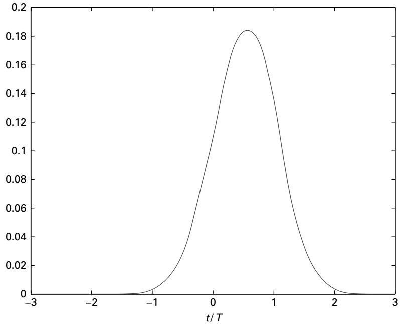
Figure 8.18 The frequency pulse g_{\text{GMSK}}(t) for Gaussian MSK with \beta = 0.3 as in the GSM system.
