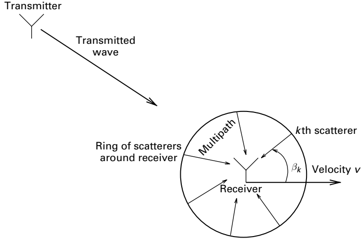
Figure 8.2 Clarke's model for time variations for a narrowband Rayleigh fading channel. The waves arriving from the ring of scatterers superimpose to result in a gain modeled as a complex Gaussian random process with PSD given by (8.11).
