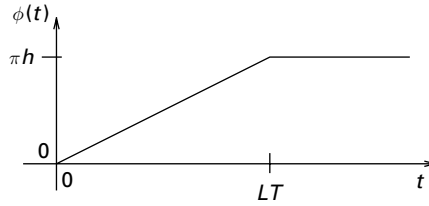
Figure 8.17 Phase pulse for CPFSK has a linear increase. Partial response CPFSK corresponds to L > 1 , and h is the modulation index.
