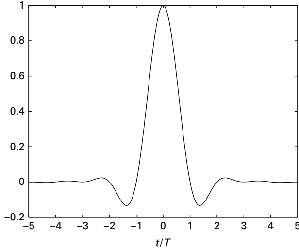
(b) Time domain pulse (excess bandwidth a = 0.5 )
