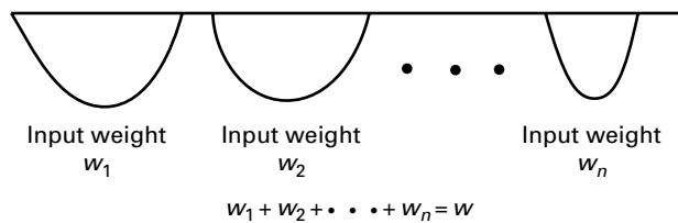
Figure 7.17 Nonzero convolutional codeword consisting of n error events, with total input weight w .
