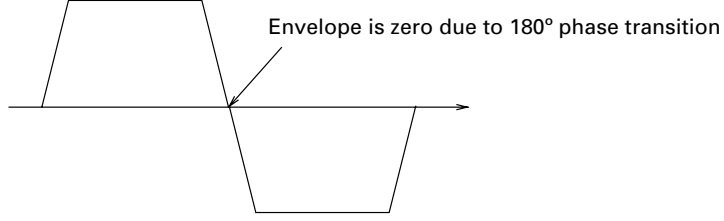
Figure 8.13 The envelope of a PSK signal passes through zero during a 180^\circ phase transition, and gets distorted over a nonlinear channel.
