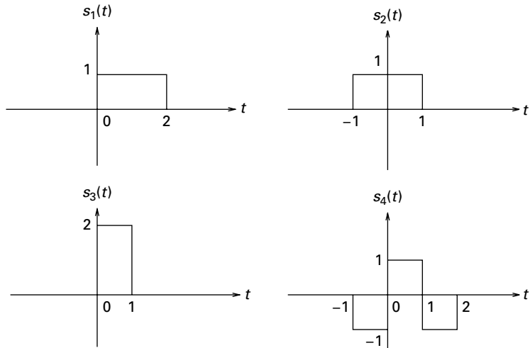
Figure 3.7 Four signals spanning a three-dimensional signal space.
