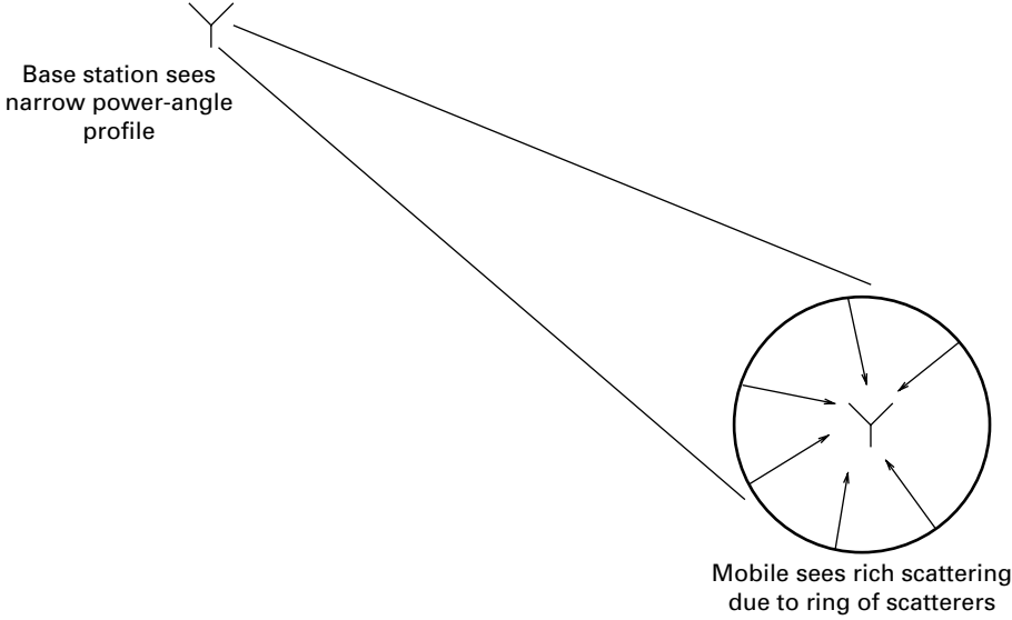
Figure 8.22 An elevated base station sees a narrow power-angle profile to a given mobile, but the mobile sees a rich scattering environment locally. The nodes may have multiple antenna elements (not shown in figure).
