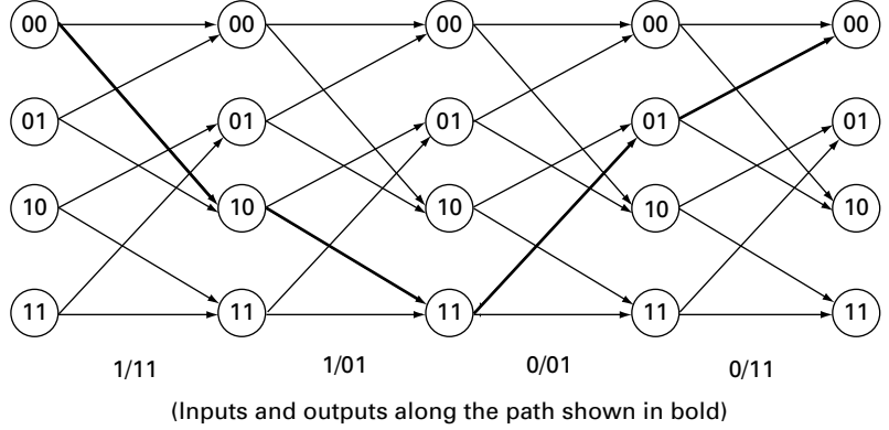
Figure 7.7 An error event for our running example of a nonrecursive, nonsystematic rate 1/2 code with generator [7, 5].
