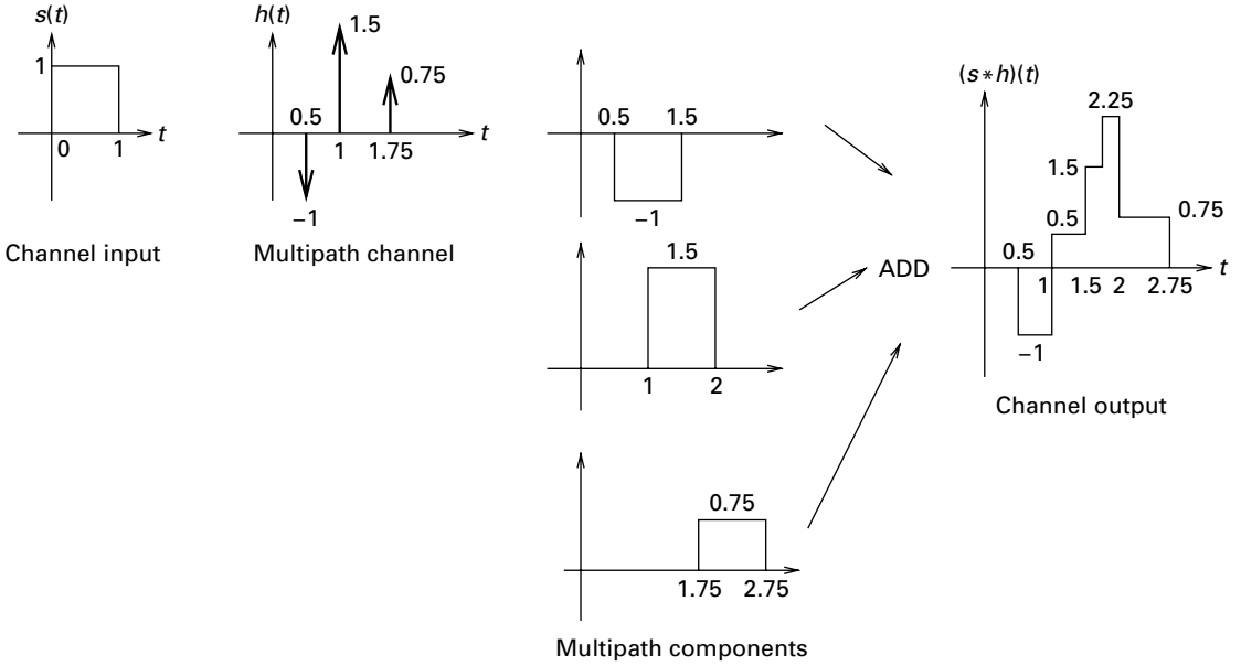
Figure 2.3 A signal going through a multipath channel.
