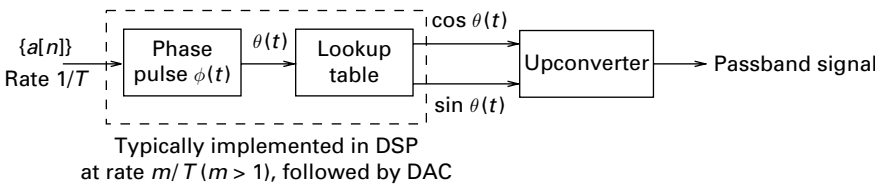
Figure 8.16 Digital signal processing-centric realization of a CPM modulator. The linear modulation of the phase \theta(t) , followed by look-up of the sine and cosine, is often implemented in DSP at an integer multiple of the symbol rate, followed by digital-to-analog conversion prior to upconversion.
