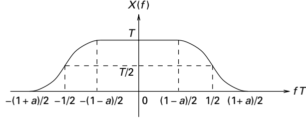
(a) Frequency domain raised cosine
