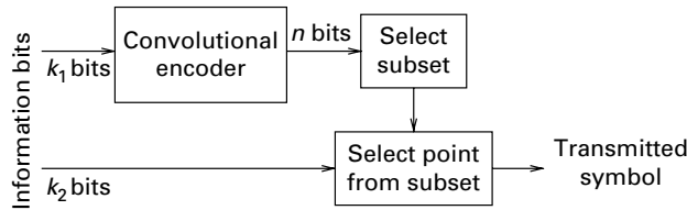
Figure 7.24 A TCM encoder uses convolutionally coded bits to select a subset of points, and uncoded bits to select points within the subset. In the figure, the constellation has 2^{n+k_2} points, divided into 2^n subsets, each with 2^{k_2} points. The convolutional code has rate k_1/n .
