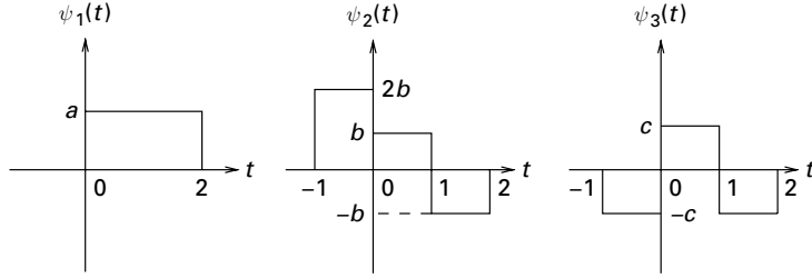
Figure 3.9 An orthonormal basis for the signal set in Figure 3.7, obtained by applying the Gramm–Schmidt procedure. The unknowns a , b , and c are to be determined in Exercise 3.3.1.
