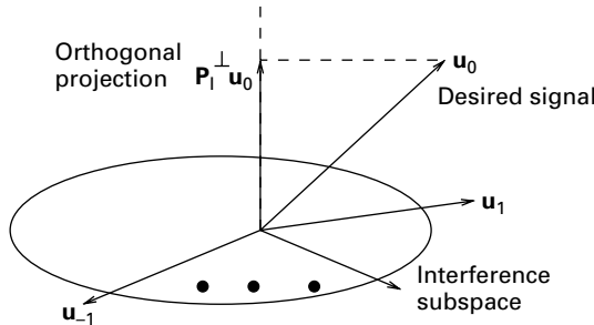
Figure 5.9 The geometry of zero-forcing equalization.
