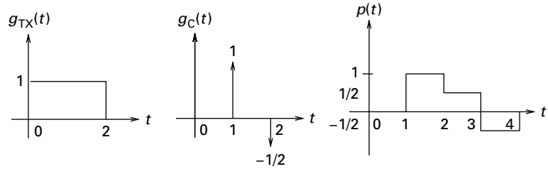
Figure 5.2 Transmit pulse g_{\text{TX}}(t) , channel impulse response g_{\text{C}}(t) , and overall pulse p(t) for the running example. The symbol rate is 1/2 symbol per unit time.
