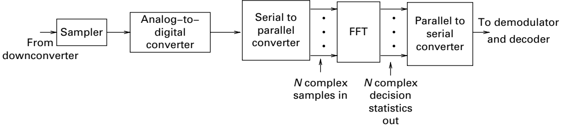
Figure 8.5 DSP-centric implementation of an OFDM receiver. Carrier and timing synchronization blocks are not shown.
