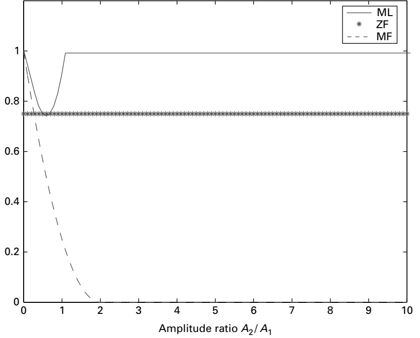
Figure 8.11 Asymptotic efficiency for User 1 as a function of the ratio of amplitudes A_2/A_1 for normalized correlation \rho = \pm 0.5 . The ML and ZF detectors are near-far resistant, while the near-far resistance for the MF goes to zero once A_2 \geq 2A_1 .
