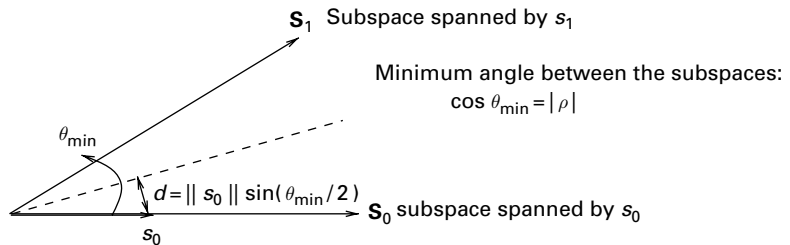
Figure 4.7 Geometric view of noncoherent demodulation.
