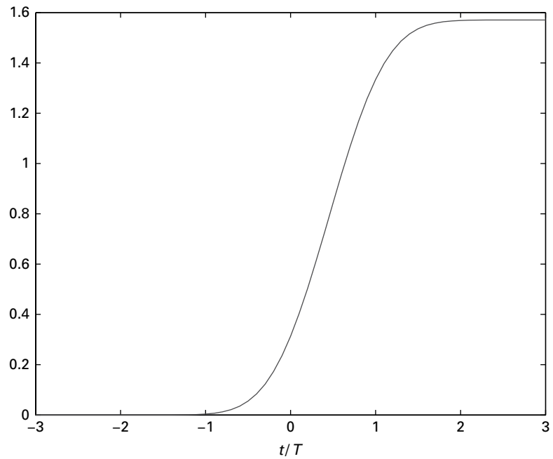
Figure 8.20 The phase pulse \phi_{\text{GMSK}}(t) for Gaussian MSK with \beta = 0.3 . Note that the variation of the phase can be captured in an interval of length L = 4 .
