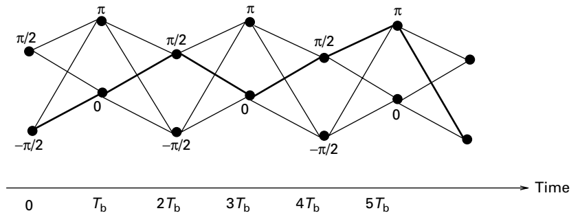
Figure 8.15 A trellis representation for the phase evolution of MSK. The path in bold corresponds to the realization shown in Figure 8.14.
