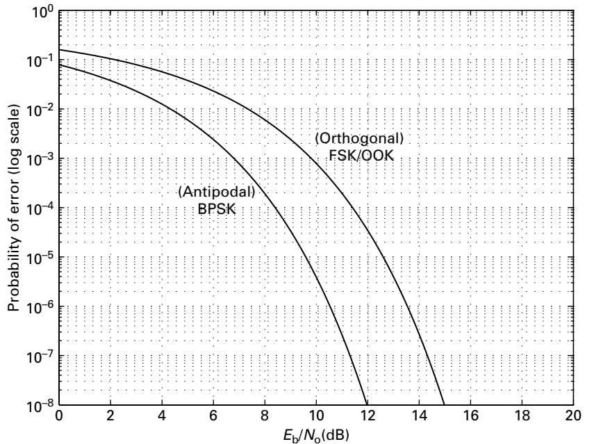
Figure 3.15 Bit error rate versus E_b/N_0 (dB) for antipodal and orthogonal signaling.
