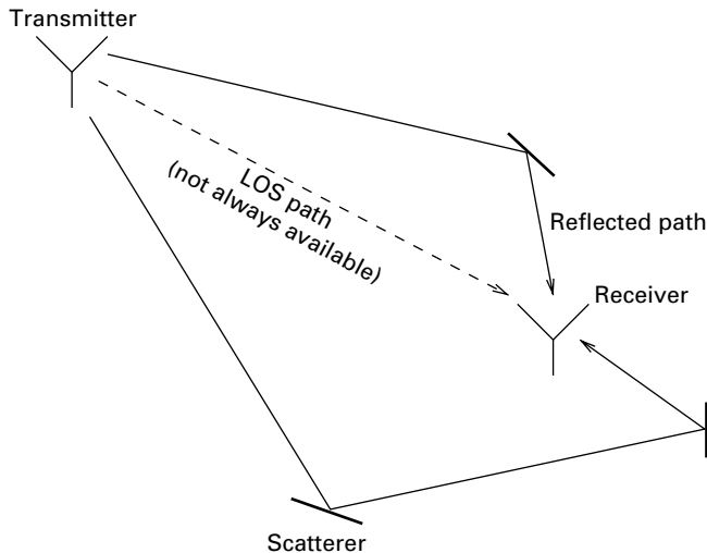
Figure 8.1 The signal from transmitter to receiver in a wireless system may undergo reflections from multiple scatterers, creating a multipath channel. The line of sight (LOS) path may or may not be available, depending on the propagation environment.
