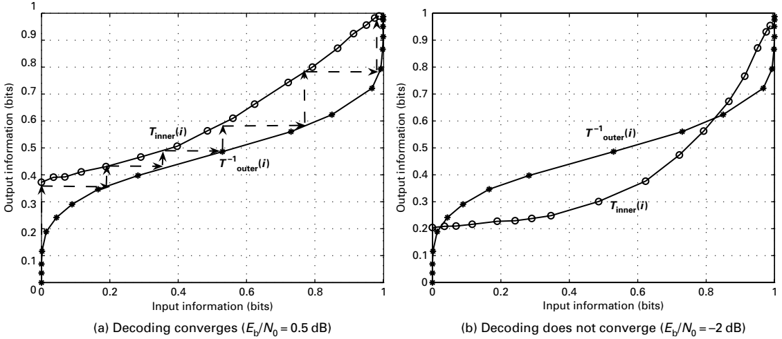
Figure 7.16 The EXIT charts for a rate 1/4 serial concatenated turbo code. Inner and outer codes are identical recursive systematic rate 1/2 [7, 5] convolutional codes.
