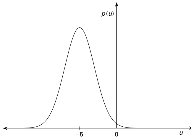
Figure 3.1 The shape of an N(-5, 4) density.
