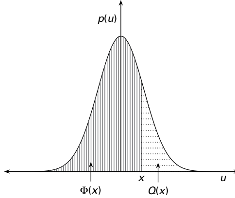
Figure 3.2 The \Phi and Q functions are obtained by integrating the N(0, 1) density over appropriate intervals.
