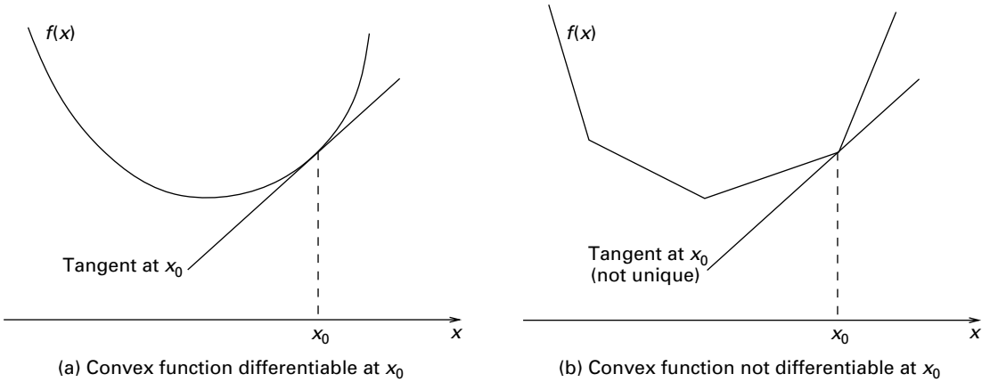
Figure C.1 Tangents for convex functions lie below it.
