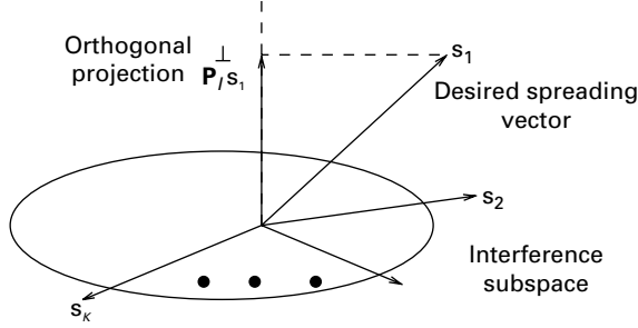
Figure 8.10 The ZF correlator is a scalar multiple of the projection of the desired spreading vector orthogonal to the interference subspace.
