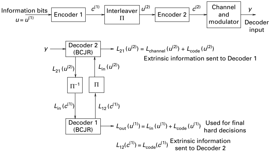
Figure 7.11 Encoder and decoder for a serial concatenated turbo code.
