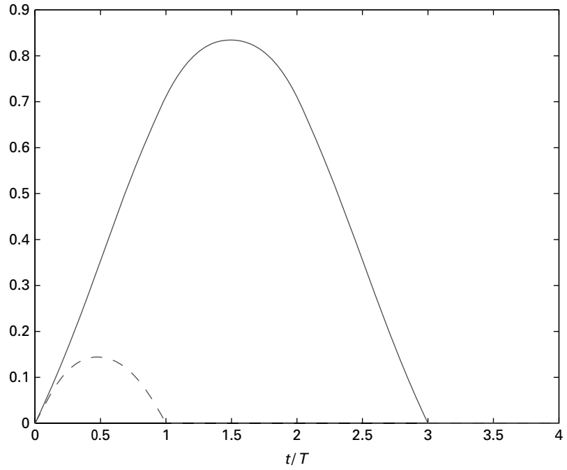
Figure 8.19 Laurent pulses s_0 and s_1 for CPFSK with L = 2 , computed as described in Example 8.6.1. Note that the dominant pulse s_0(t) , shown using an unbroken line, is much larger than the pulse s_1(t) , shown using a dashed line.
