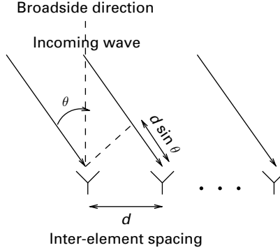
Figure 8.21 Geometry of a linear antenna array.
