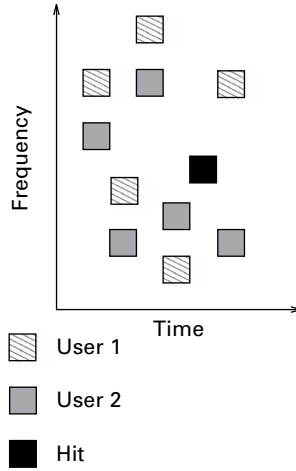
Figure 8.12 Frequency hop users employ hopping patterns that collide occasionally.
