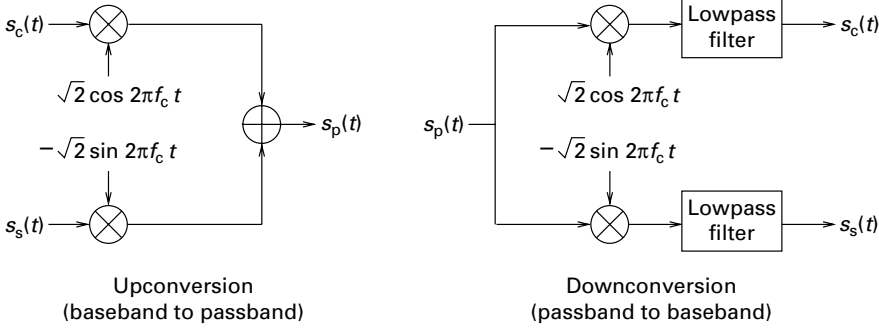
Figure 2.9 Upconversion from baseband to passband and downconversion from passband to baseband.
