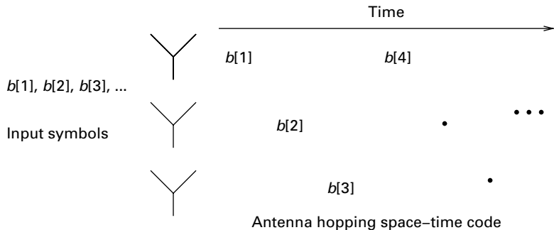
Figure 8.23 Antenna hopping space–time code.
