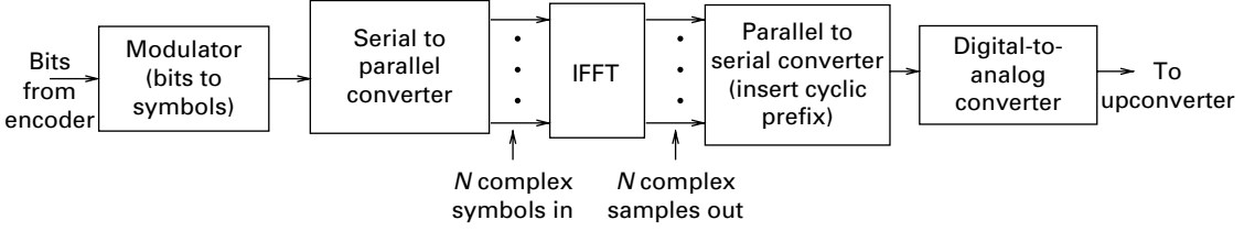
Figure 8.4 DSP-centric implementation of an OFDM transmitter.
