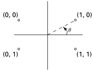
Figure 3.29 Signal constellation with unequal error protection (Problem 3.19).
