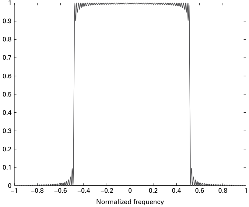
Figure 8.6 The PSD of OFDM with N = 64 subcarriers as a function of normalized frequency fT/N .
