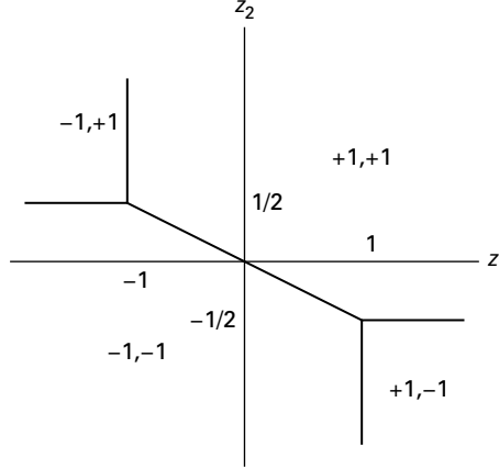
Figure 8.9 Decision regions for ML reception with two users: A_1 = 1 , A_2 = 2 and \rho = -1/2 in Example 8.4.2.
