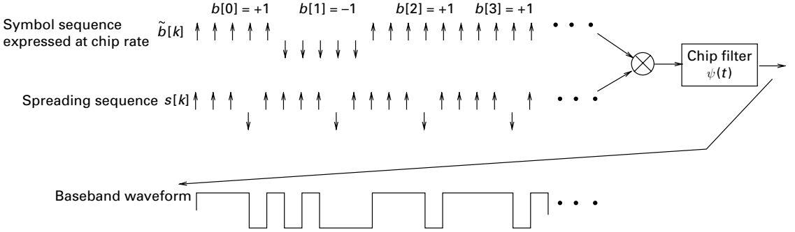
Figure 8.7 Example of DS modulation, with processing gain N = 5 and a short spreading sequence. In this chip rate implementation, the data sequence is converted to the chip rate and is multiplied chip-by-chip with the spreading sequence before modulating the chip waveform. These discrete-time chip rate sequences are indicated by delta functions in the figure. These are then passed through a chip filter (which may itself be implemented in DSP at a multiple of the chip rate, followed by digital-to-analog conversion) to obtain the baseband analog waveform to be upconverted.
