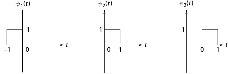
Figure 3.8 An orthonormal basis for the signal set in Figure 3.7, obtained by inspection.
