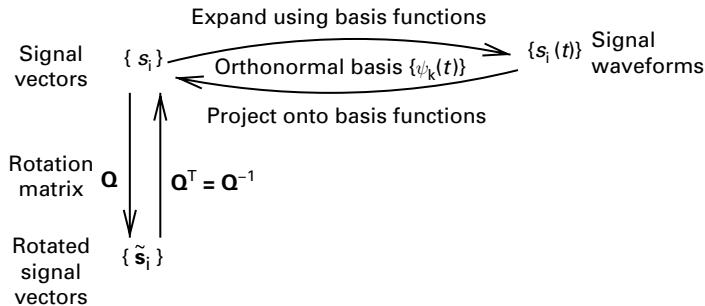
Figure 3.16 Transformations of the signal constellation that leave performance over the AWGN channel unchanged.
