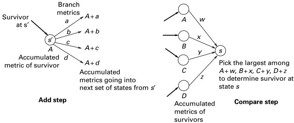
Figure 5.7 The add and compare steps in the Viterbi algorithm.
