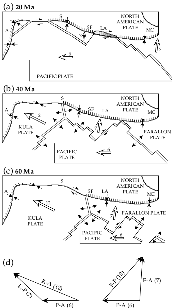
Fig. 1.23 (a)–(c) Extrapolated plate relationships in the northeast Pacific at different times in the Cenozoic (after Atwater, 1970). Letters on the American plate give approximate locations of some modern cities for reference: MC, Mexico City; LA, Los Angeles; SF, San Francisco; S, Seattle; A, Anchorage. The shaded area in (a) is an unacceptable overlap. (d) Vector diagrams of the relative plate velocities at the Kula–Pacific–American and Farallon–Pacific–American triple junctions (numbers are velocities in \text{cm yr}^{-1} relative to the American plate).
