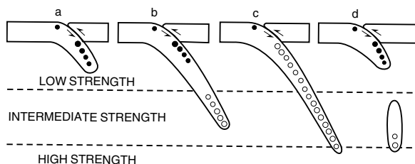
Fig. 1.18 Stresses acting on a subducting lithospheric plate. Arrows indicate shear where the underriding plate is bent downward. Solid and open circles within the descending slab denote extension and compression, respectively; the size of the circle represents qualitatively the seismic activity. In (a), (b) and (d) extensional stress in the upper part of the plate is due to the slab being pulled into low-strength asthenosphere. In (b) resistance of the more rigid layer under the asthenosphere causes compression within the lower part of the slab; if the plate sinks far enough, (c), the stress becomes compressional throughout; in some cases, (d), the deep part of the lower slab may break off (after Isacks and Molnar, 1969).
