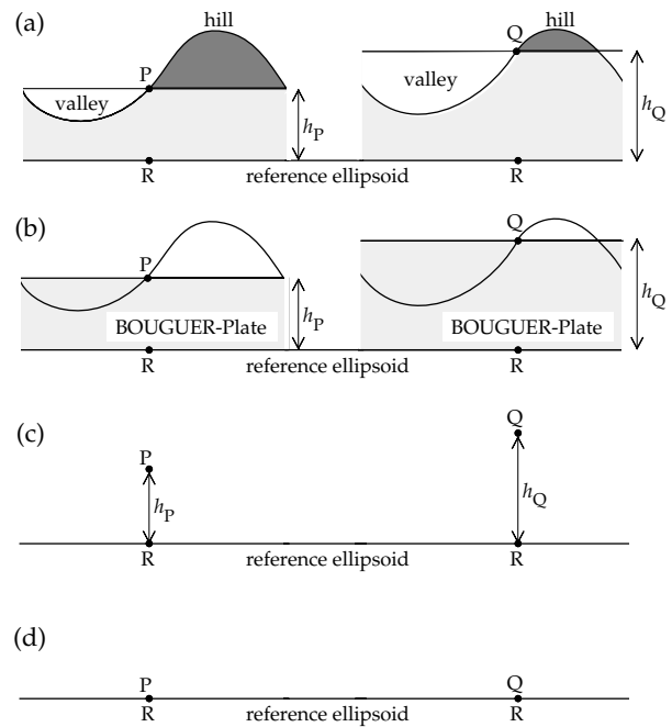
Fig. 2.37 After (a) terrain corrections, (b) the Bouguer plate correction, and (c) the free-air correction, the gravity measurements at stations P and Q can be compared to (d) the theoretical gravity at R on the reference ellipsoid.
