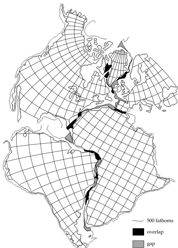
Fig. 1.6 Computer-assisted fit of the Atlantic-bounding continents at the 500 fathom (900 m) depth (after Bullard et al. , 1965).
