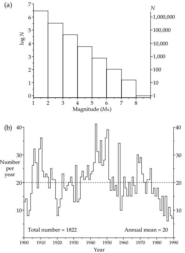
Fig. 3.49 Histograms of (a) the logarithm of the number ( N ) of earthquakes per year with magnitude M_s , and (b) the annual number of earthquakes with magnitudes M_s \geq 7 since 1900 (based on data from the US Geological Survey National Earthquake Information Center).
