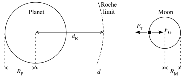
Fig. B2.1.2 Parameters for computation of the Roche limit.
