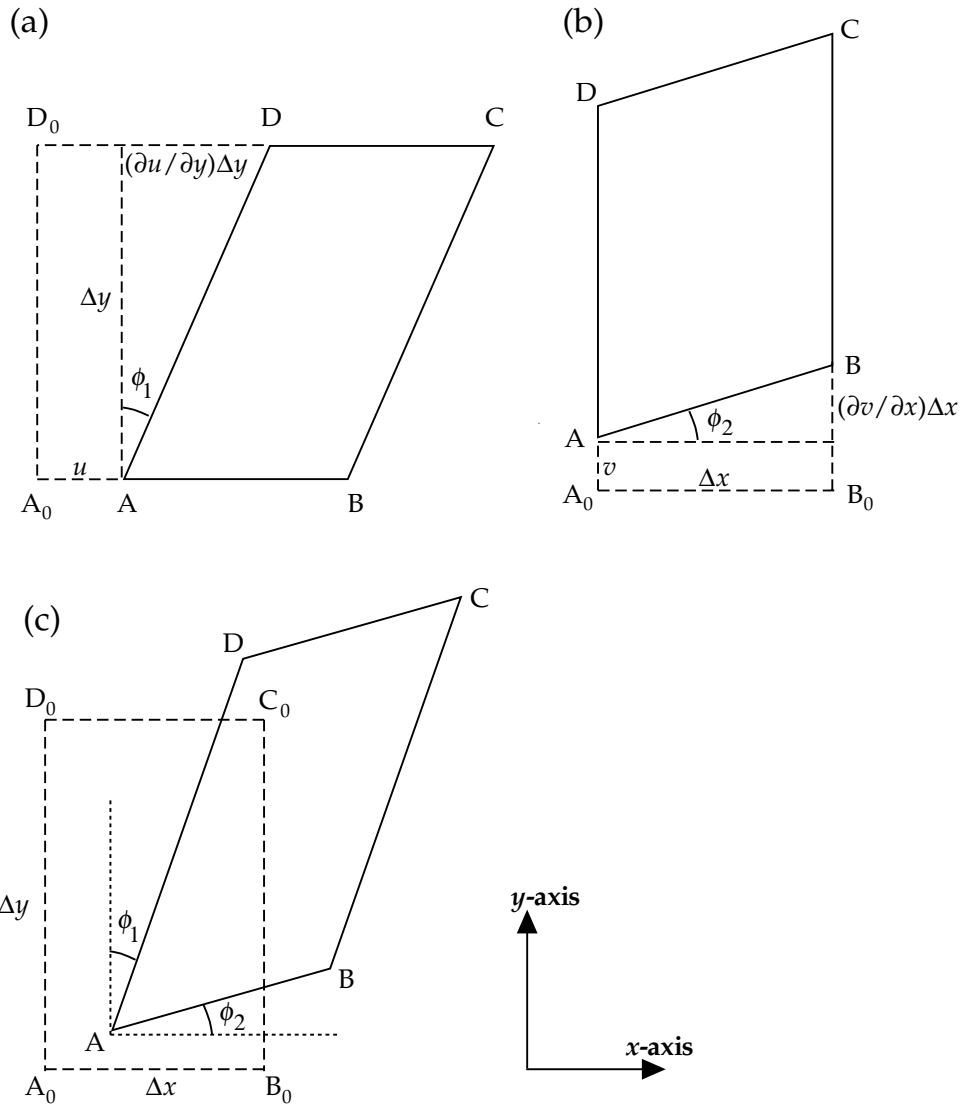
Fig. 3.6 (a) When a square is sheared parallel to the x -axis, side AD parallel to the y -axis rotates through a small angle \phi_1 ; (b) when it is sheared parallel to the y -axis, side AB parallel to the x -axis rotates through a small angle \phi_2 . In general, shear causes both sides to rotate, giving a total angular deformation (\phi_1 + \phi_2) . In each case the diagonal AC is extended.
