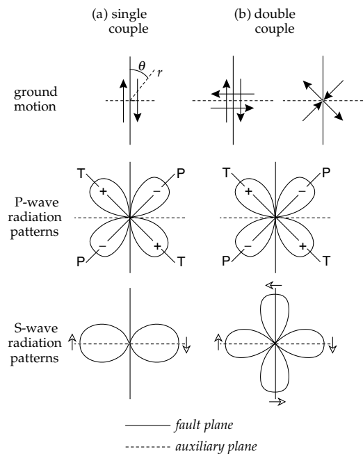
Fig. 3.35 Azimuthal patterns of amplitude variation for (a) single-couple and (b) double-couple earthquake source models are the same for P-waves but differ for S-waves. The radius of each pattern at azimuth \theta from the fault-plane is proportional to the amplitude of the seismic wave in this direction. For P-waves the fault plane and auxiliary plane are nodal planes of zero displacement. The maximum compressional amplitude is along the T-axis at an angle of 45^\circ to the fault plane. The dilatational amplitude is maximum along the P-axis, also at 45^\circ to the fault plane.
