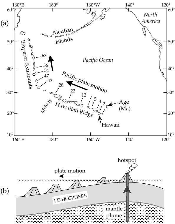
Fig. 1.26 (a) The Hawaiian Ridge and Emperor Seamount volcanic chains trace the motion of the Pacific plate over the Hawaiian hot spot; numbers give the approximate age of volcanism; note the change in direction about 43 Ma ago (after Van Andel, 1992). (b) Sketch illustrating the formation of volcanic islands and seamounts as a lithospheric plate moves over a hot spot (based on Wilson, 1963).
