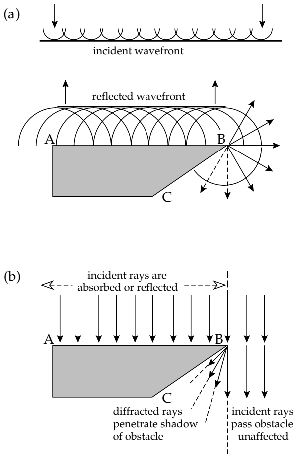
Fig. 3.55 Explanation of diffraction at an edge with the aid of Huygens' principle. (a) The incident and reflected plane wavefronts are the envelopes to Huygens wavelets, which are able to carry the incident disturbance around a sharp corner. (b) The incident rays are absorbed, reflected or pass by the obstacle, but some rays related to the wavelets generated at the point of the obstruction are diffracted into its shadow.
