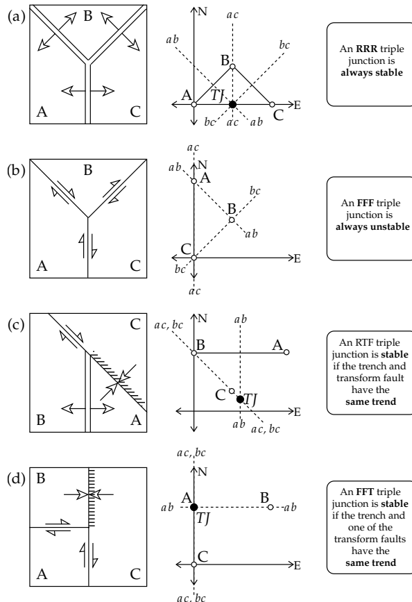
Fig. 1.22 Triple junction configuration (left), velocity lines of each margin in velocity space (center), and stability criteria (right) for selected triple junctions, TJ (after Cox and Hart, 1986).
