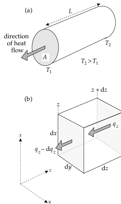
Fig. 4.15 (a) Conduction of heat Q through a bar of length L and cross-sectional area A , with its ends kept at temperatures T_1 and T_2 ( T_2 > T_1 ). (b) Heat flux entering ( q_z ) and leaving ( q_z - dq_z ) a short bar of length dz .
