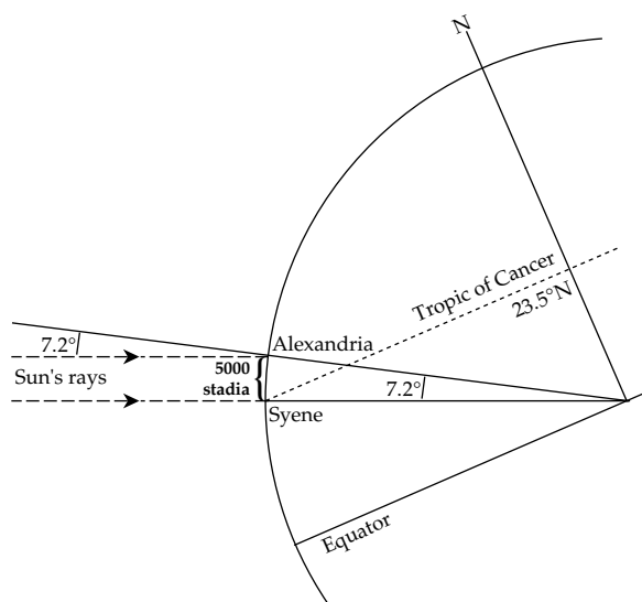
Fig. 2.1 The method used by Eratosthenes (275–195 BC) to estimate the Earth's circumference used the 7.2^\circ difference in altitude of the Sun's rays at Alexandria and Syene, which are 5000 stadia apart (after Strahler, 1963).
