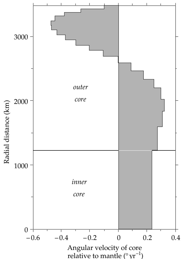
Fig. 5.38 Interpreted velocity distribution (relative to the mantle) for a multi-layered core model in which the change of angular momentum of each layer due to convective fluid motion is balanced by electromagnetic forces (after Watanabe and Yukutake, 1975).
