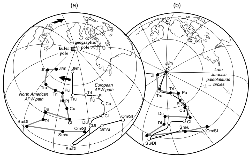
Fig. 5.67 (a) The Ordovician to Jurassic segments of the North American and European APW paths. (b) The same APW paths after rotating Europe by 38^\circ clockwise about the Euler rotation pole at 88.5^\circ\text{N} 27.7^\circ\text{E} , marked by the square symbol in (a) (after Van der Voo, 1990).
