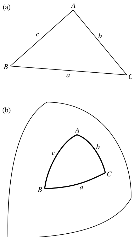
Fig. B1.4 The sides and angles of (a) a plane triangle, (b) a spherical triangle.
