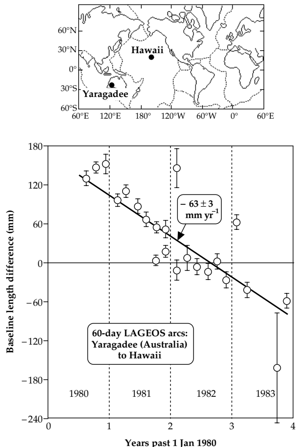
Fig. 2.27 Changes in the arc distance between satellite laser-ranging (SLR) stations in Australia and Hawaii determined from LAGEOS observations over a period of four years. The mean rate of convergence, 63 \pm 3 \text{ mm yr}^{-1} , agrees well with the rate of 67 \text{ mm yr}^{-1} deduced from plate tectonics (after Tapley et al. , 1985).
