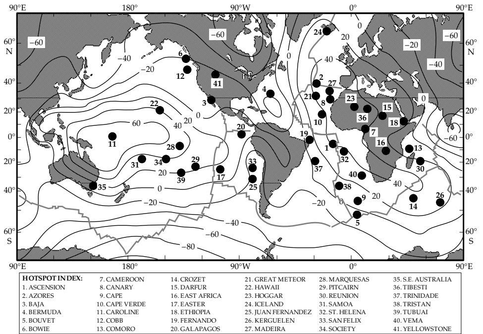
Fig. 1.25 The global distribution of 41 hotspots and their relationship to the residual geoid obtained by correcting geoid heights (shown in meters above the reference ellipsoid) for the effects of cold subducting slabs (after Crough and Jurdy, 1980).
