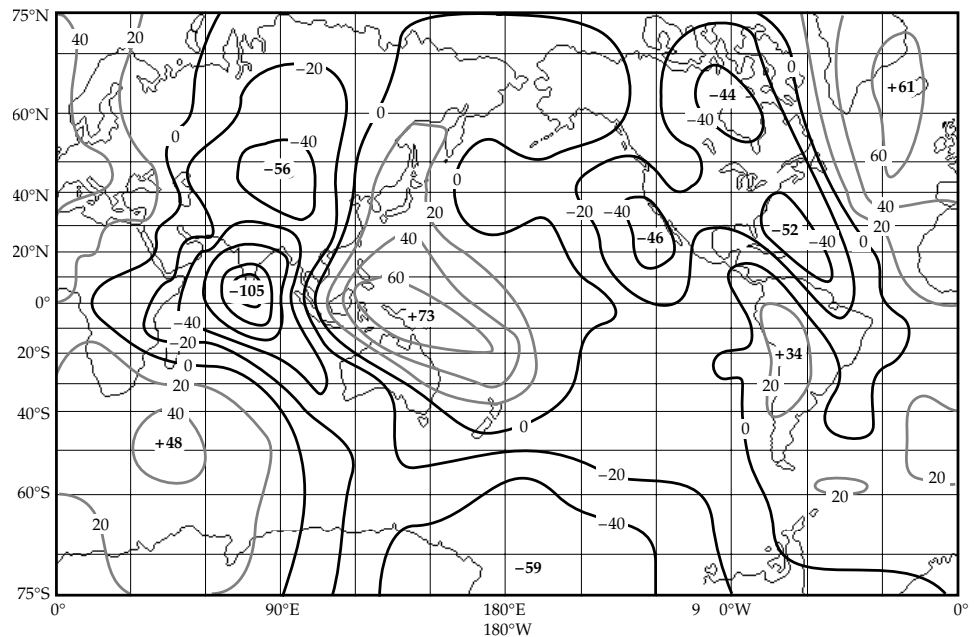
Fig. 2.25 World map of geoid undulations relative to a reference ellipsoid of flattening f = 1/298.257 (after Lerch et al. , 1979).
