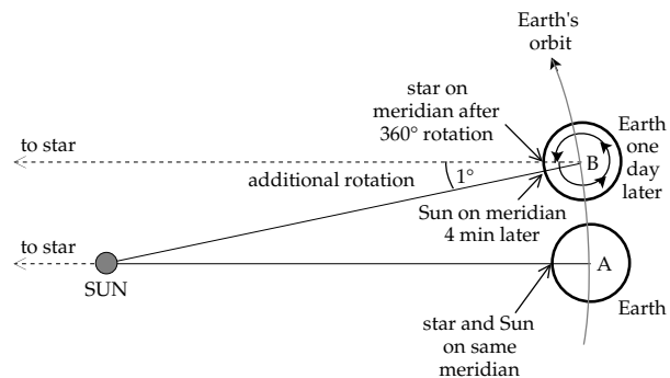
Fig. 4.1 The sidereal day is the time taken for the Earth to rotate through 360^\circ relative to a fixed star; the solar day is the time taken for a rotation between meridians relative to the Sun. This is slightly more than 360^\circ relative to the stars, because the Earth is also orbiting the Sun.
