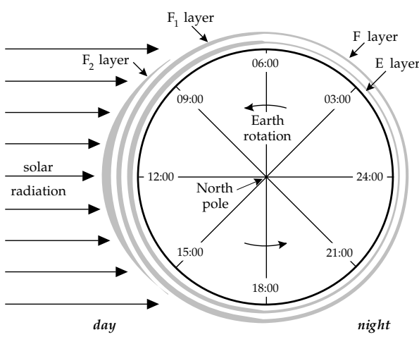
Fig. 5.31 Cross-section through the Earth showing the layered structure of the ionosphere (after Strahler, 1963).
