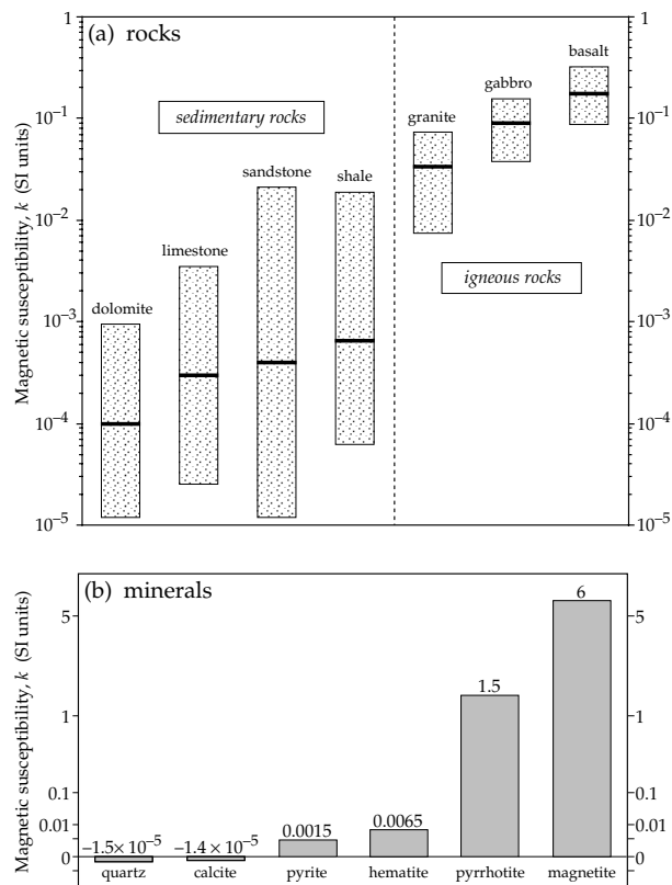
Fig. 5.13 (a) Median values and ranges of the magnetic susceptibility of some common rock types, and (b) the susceptibilities of some important minerals.
