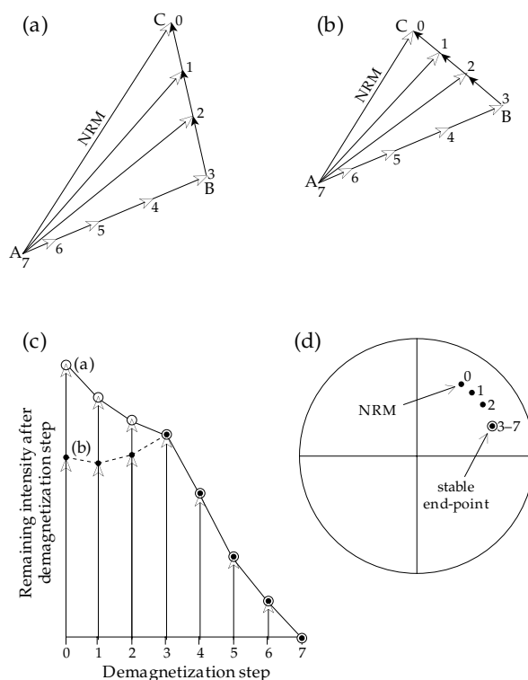
Fig. 5.56 Stepwise demagnetization of a remanent magnetization consisting of two components with different ranges of stability: (a) low stability vector BC demagnetizes before stable vector AB; (b) same situation with different angle between AB and BC; (c) variation of intensity for cases (a) and (b); and (d) directional changes on a stereogram. Numbers on points indicate successive demagnetization temperatures in ^\circ\text{C} .
