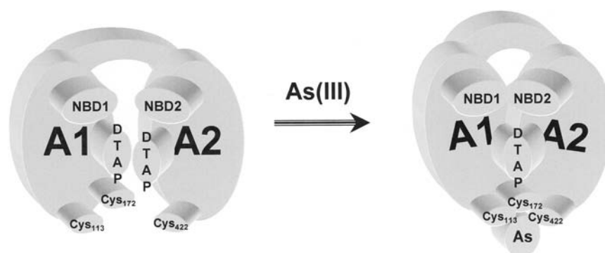
FIGURE 5 Model of ArsA catalysis. In the absence of metalloid activator, the A1 and A2 halves of ArsA are independent of each other, with only the A1 NBD exhibiting a basal rate of ATP hydrolysis (48). Binding of Sb(III) or As(III) to Cys113, Cys172, and Cys422 brings the halves together. This results in interaction of the A1 and A2 NBDs to interact and promotion of catalysis. Conformational changes in the conserved DTAP domains report binding and hydrolysis of nucleotides (51,52).
