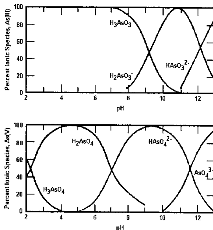
FIGURE 2 Acidic dissociation diagram for H 3 As III O 3 and H 3 As V O 4 . (Adapted from ref. 271.)
