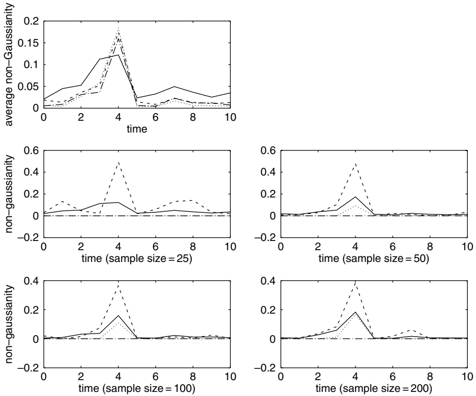
Figure 15.1 Fourier mode: \mathbf{k} = 0 . Top panel: shows the average non-Gaussianity, over 20 ensembles, with sample sizes 25 (solid), 50 (dashed), 100 (dot-dashed), and 200 (dotted). Panels 2–4: The solid curve shows the average non-Gaussianity for the indicated sample size. The dashed curve shows the ensemble with the largest non-Gaussianity at time t = 4 . The dot-dashed curve shows the adjusted moment technique applied to this ensemble. The dotted curve shows the central limit technique applied to this ensemble.
