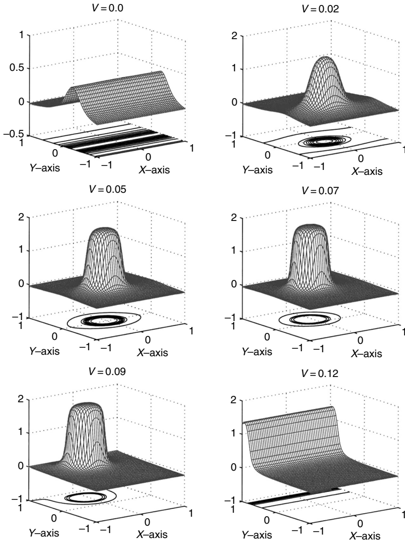
Figure 11.5 Plot of potential vorticity of maximum entropy solutions in Langevin theory, with “energy” \tilde{E} = 0.03 , circulation \Gamma = 1.0 , \beta = 0.3 , \bar{Q} = 0.9 and Q = 1.0 , a variable mean flow ranging from V = 0.0 to V = 0.12 .
