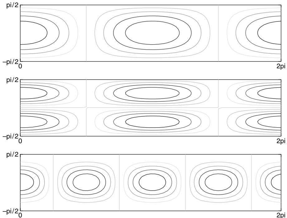
Figure 16.2 Surface spherical harmonics corresponding to spherical Rossby waves in moving frames. Top: \cos \theta \cos \phi , n = m = 1 ; middle: \cos \theta \sin \theta \cos \phi , n = 2, m = 1 ; bottom: \cos^2 \theta \cos(2\phi) , n = m = 2 .
