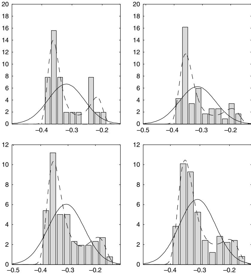
Figure 15.4 Fourier mode: \mathbf{k} = 3 . Each graph shows a histogram of the data from panels 2–4 in Fig. 15.3 at time t = 3 . The Gaussian and four-moment fits are overlaid.
