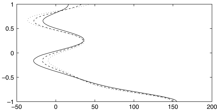
Figure 13.6 The Limate profile (solid) in the northern hemisphere band, and the zonal velocity profiles for the equilibrium states with \varepsilon = -0.02 (dashed) and \varepsilon = -0.032 (dotted) and the same energy and circulation as the Limate zonal flow; each of these computed solutions is purely zonal.
