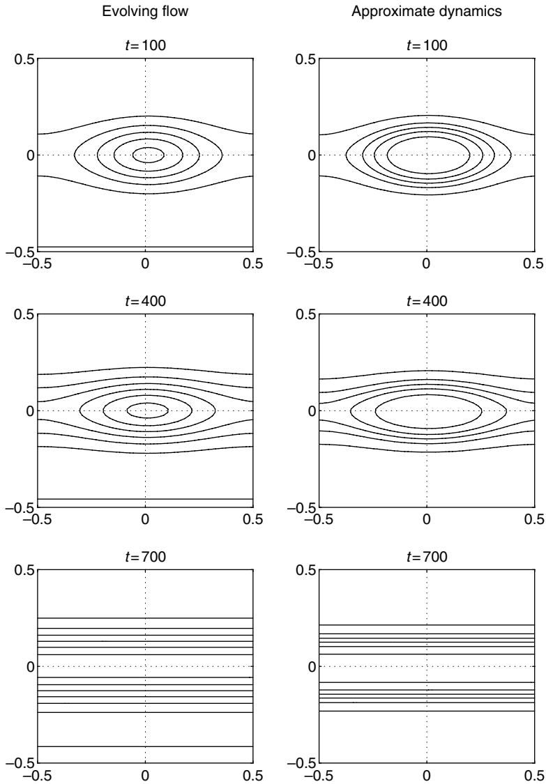
Figure 12.3 Contour lines of the potential vorticity fields at times t = 100, 400 , and 700 for the numerical experiment described in Figure 12.2. Left-hand column: snapshots of the evolving flow, right-hand column: most probable states of the statistical theory.
