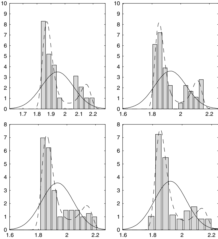
Figure 15.2 Fourier mode: k = 0 . Each graph shows a histogram of the data from panels 2–4 in Figure 15.1 at time t = 4 . The Gaussian and four-moment fits are overlaid.
