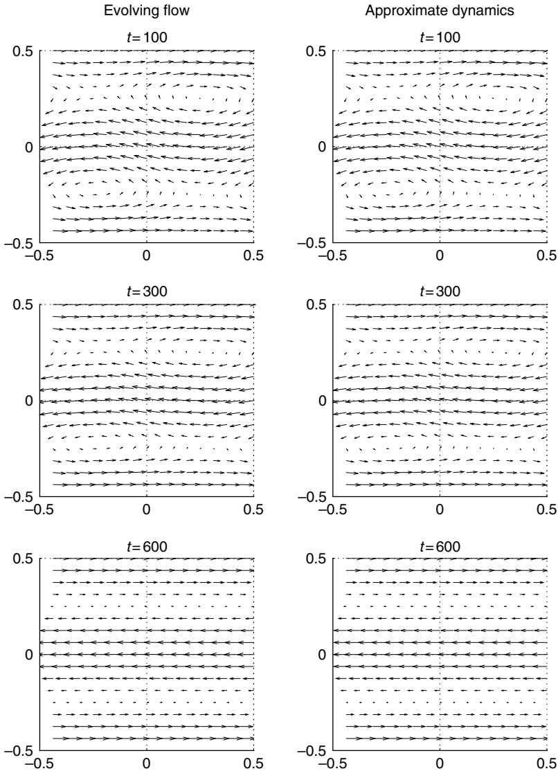
Figure 12.5 Velocity field at times t = 100 , 300 , and 600 for the numerical experiment described in Figure 12.4. Left-hand column: snapshots of the evolving flow, right-hand column: most probable states of the statistical theory.
