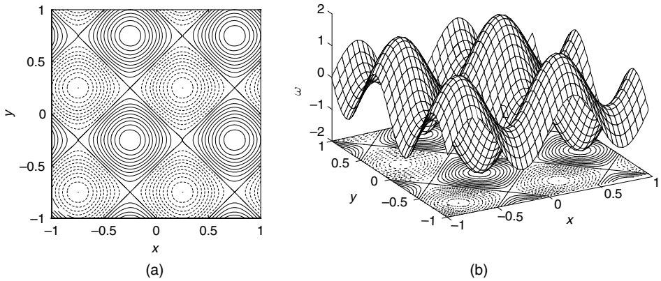
Figure 1.2 2-D array of swirling eddies with stream function \psi(x, y) = \sin(x) + \sin(y) ( x and y both normalized by 2\pi ). (a) Plot of the streamlines: counter-clockwise rotation (—); clockwise rotation (- -). (b) Plot of the vorticity \omega .
