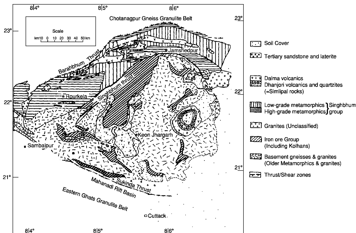
Figure 5 Geological map of the Singhbhum Craton (adapted with permission from Mahadevan TM, 1994; © Geological Society of India, Bangalore).
