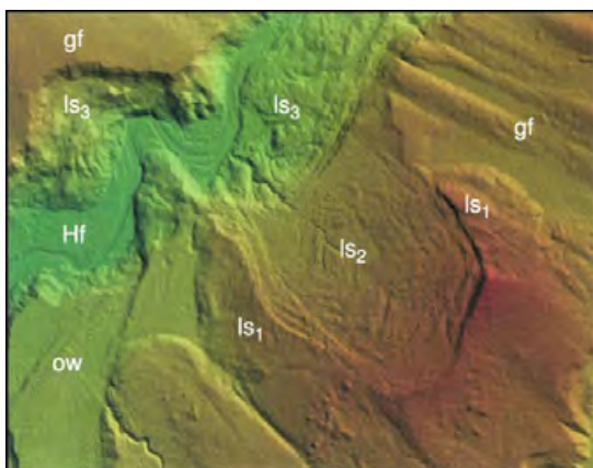
Figure 5 Lidar topography showing landslides near Seattle, Washington. The view is 3.5 km wide. Symbols: ow, outwash; ls, landslides (1 = youngest, 3 = oldest); Hf, Holocene flood plain; gf, glacially fluted surface. Courtesy of the Geological Society of America (see GSA Today , November 2003, pp. 4–10).
