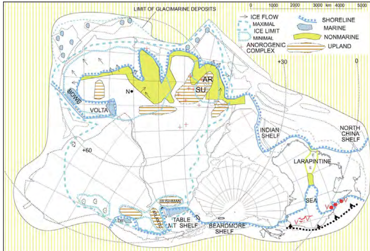
Figure 6 Late Ordovician (458–443 Ma) palaeogeography: DB, the glaciomarine Don Braulio Formation; AR, Arabian upland; SU, Sudan upland; E, area of evaporite deposition; += anorogenic complex. Reproduced with permission from Veevers JJ (2004) Gondwanaland from 650–500 Ma assembly through 320 Ma merger in Pangaea to 185–100 Ma breakup: supercontinental tectonics via stratigraphy and radiometric dating. Earth Science Reviews
