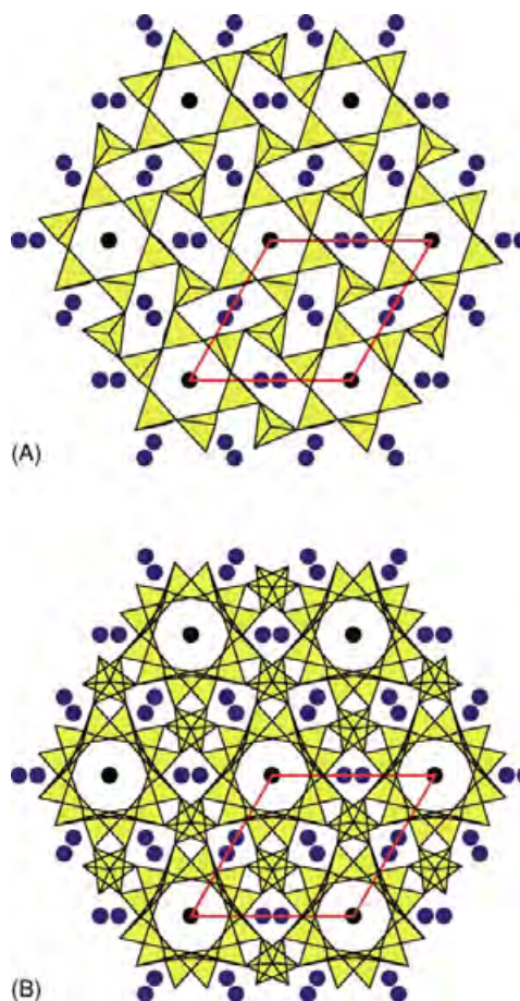
Figure 3 (A) The characteristic sheet of distorted and undistorted six-membered rings of \text{AlO}_4 and \text{SiO}_4 tetrahedra in the nepheline-type structure. Blue circles are sodium ions occupying smaller channel sites above and below the sheet, and black circles are potassium ions occupying the larger regular channels. The projection of the unit cell is shown in red. (B) A complete double sheet of the nepheline-type structure, showing the two kinds of channel.
