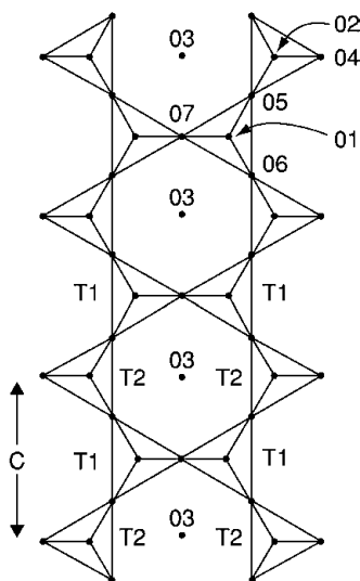
Figure 1 Double chain of linked (Si,Al) \text{O}_4 tetrahedra characteristic of all amphiboles.
