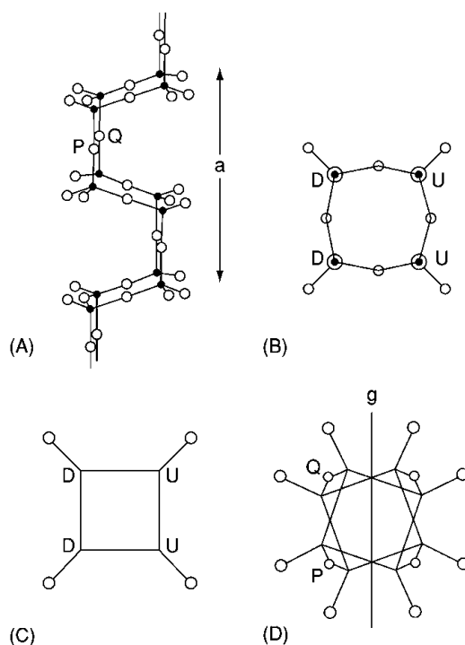
Figure 2 Idealized illustrations of the feldspar 'chain'. In (B) and (C) U and D indicate tetrahedra pointing up and down, respectively.
