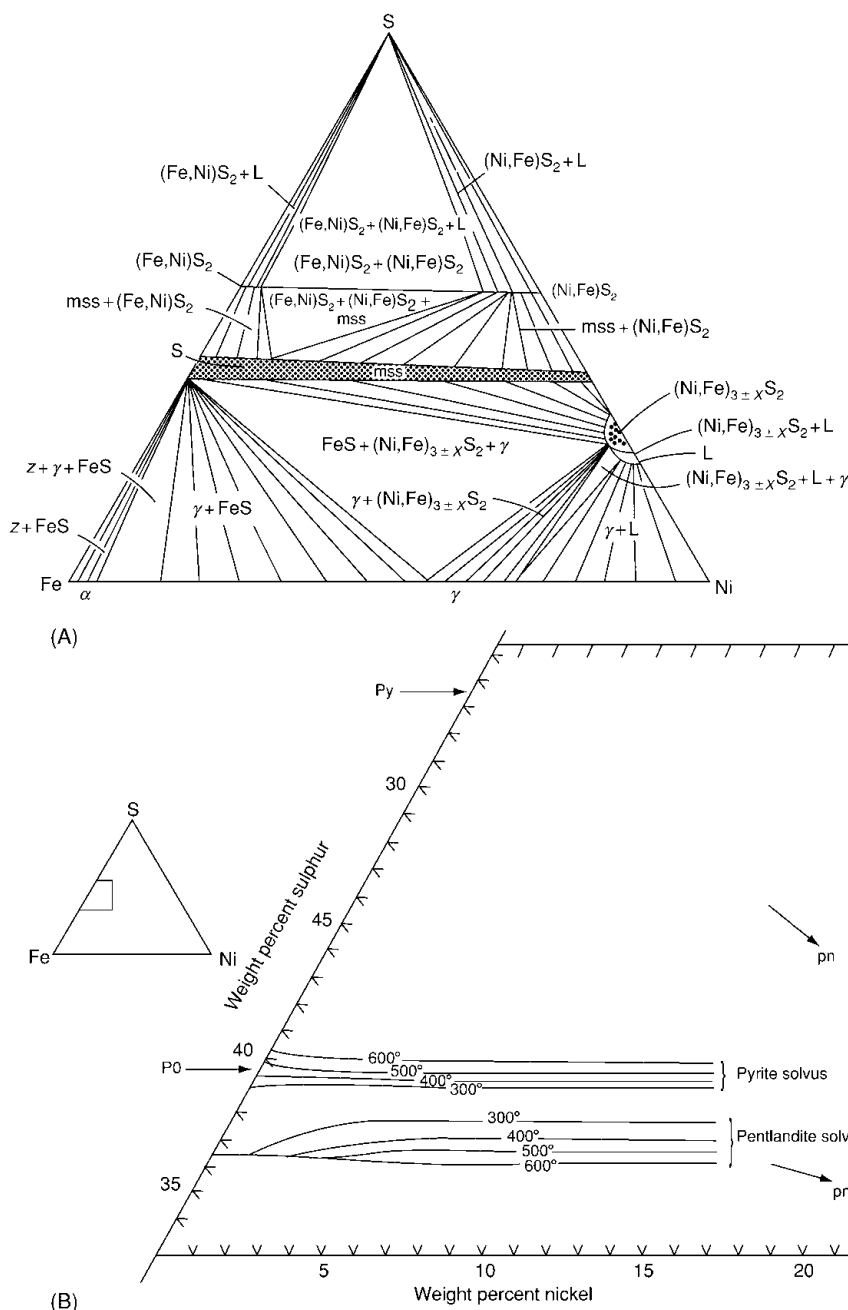
Figure 6 (A) The condensed phase relations in the Fe–Ni–S system at 650°C. Note the absence of pentlandite and the area of monosulphide solid solution ( mss ) that spans the system from \text{Fe}_{1-x}\text{S} to \text{Ni}_{1-x}\text{S} . (B) A portion of the Fe–Ni–S system, showing the compositional limits of the monosulphide solid solution in (A) at 600°C, 500°C, 400°C, and 300°C. Pentlandite flames exsolve from the mss as the sulphur-poor boundary retreats during cooling. Reproduced with permission from Geochemistry of Hydrothermal Ore Deposits , ed. H. L. Barnes, 1997, John Wiley and Sons.
