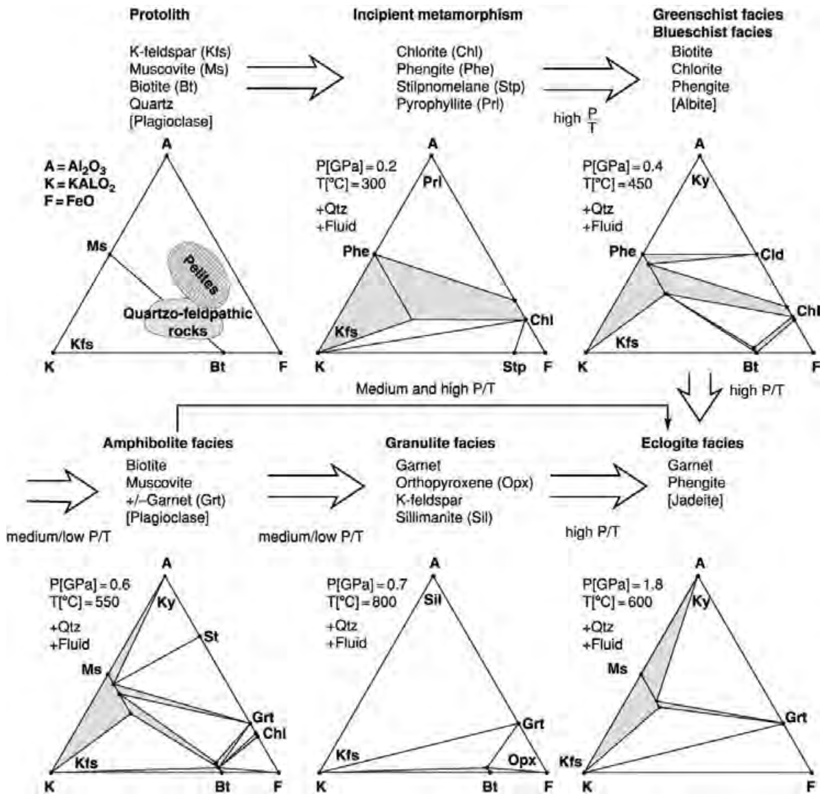
Figure 9 For the chemographic presentation of quartzzo-feldspathic rocks, the AKF-system is applied. The difference to the ACF-projection is the consideration of K instead of Ca. Again feldspar, quartz, and H 2 O are used as projection phases. K-feldspar, muscovite, biotite, and stilpnomelane are the only four important potassium-bearing minerals, besides the K-free Fe-Mg-Al-phases plotting at the AF-line. The chemical composition of quartzzo-feldspathic rocks plot in the lower Al-poor part of the triangle and therefore these lithologies contain only few and not diagnostic assemblages. The AKF chemographic projections show the significant mineral assemblages at different metamorphic grades.
