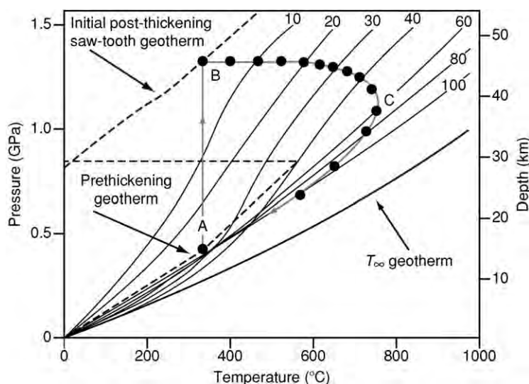
Figure 5 Schematic PTt path for crustal thickening by instantaneous overthrusting as typical for one-dimensional modelling. Point A on the prethrusting geotherm undergoes an isothermal pressure increase to B followed by isobaric heating for 20 Ma before erosion is initiated.
