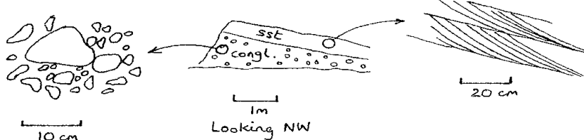
Figure 3 Field notebook. (a) The daily heading gives the date, weather conditions, general aim, and route. (b) Number the localities consecutively. Do not restart each day. An eight-figure grid reference (eastings then northings) locates the position to 10 m. (c) Describe the nature of the exposure, particularly its size. A 1 m exposure of sandstone might be part of a shale formation, whereas a
