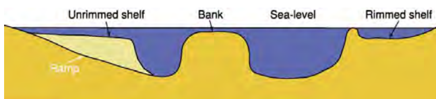
Figure 6 Schematic diagram showing differences between rimmed and unrimmed shelves, a ramp, and a bank.
