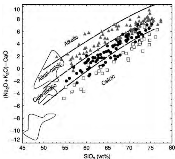
Figure 2 Subdivision of granitic rocks according to the modified alkali lime index of Frost BR, Barnes CG, Collins WJ, et al. (2001), as given by a plot of (Na 2 O + K 2 O) – CaO versus SiO 2 . Note that the trends defined by the three granitic suites – the subduction-related Peninsula Ranges (mostly calcic; open squares) and Sierra Nevada (mostly calc-alkalic; filled circles) batholiths (western USA) and the syn- to post-collisional Caledonian plutons of the UK (mostly alkali-calcic; grey triangles) – project at low silica towards coeval mantle-derived rocks in the three areas (circled fields).
