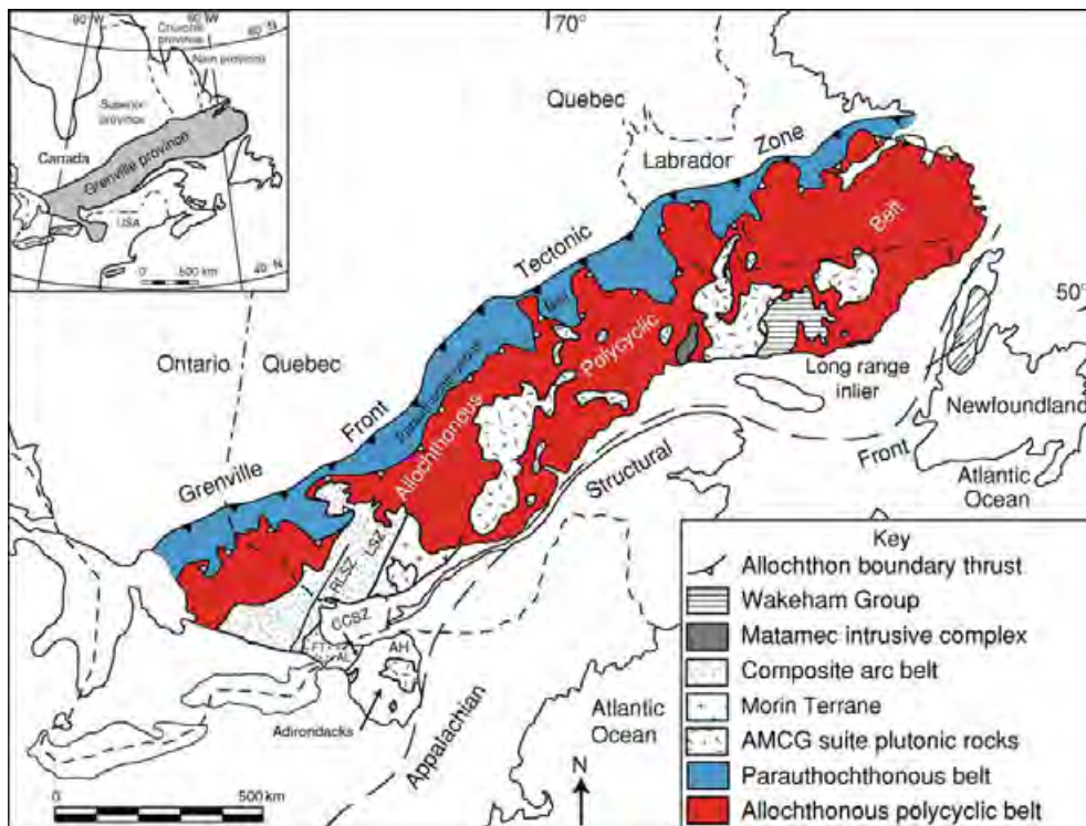
Figure 4 Map of the Grenville Province in Canada. Abbreviations: RLSZ, Robertson Lake shear zone; LSZ, Labelle shear zone; CCSZ, Carthage–Colton shear zone; FT, Frontenac Terrane; AL, Adirondack Lowlands; AH, Adirondack Highlands; AMCG, anorthosite–mangerite–charnockite–granite. Nomenclature for principal lithotectonic belts of the Canadian Grenville Province adopted from the work of the Carr group and Rivers and co-workers. Modified with permission from Davidson A (1998) An overview of Grenville Province geology, Canadian Shield. In: Lucas SB and St-Onge MR (coordinators) Geology of the Precambrian Superior and Grenville Provinces and Precambrian Fossils in North America: Geological Survey of Canada, Geology of Canada, No. 7, chapt. 3, pp. 205–270 . Dartmouth, NS: Geological Survey of Canada.
