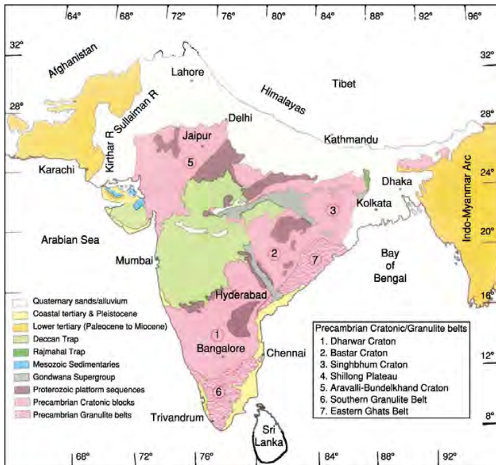
Figure 2 Generalised geological map of the Indian Sub-Continent.
