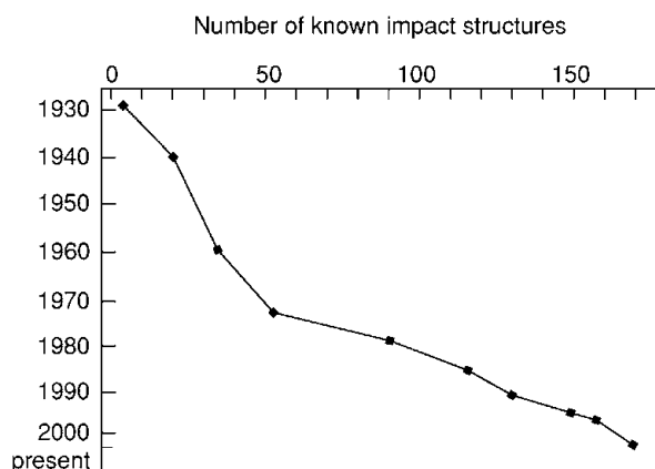
Figure 1 Number of known terrestrial impact structures recognized with time. Note the increase in the rate of discovery after the 1970s, due to the establishment of shock metamorphism (see text for details) as a reliable criterion for identifying the impact origin of specific structures.
