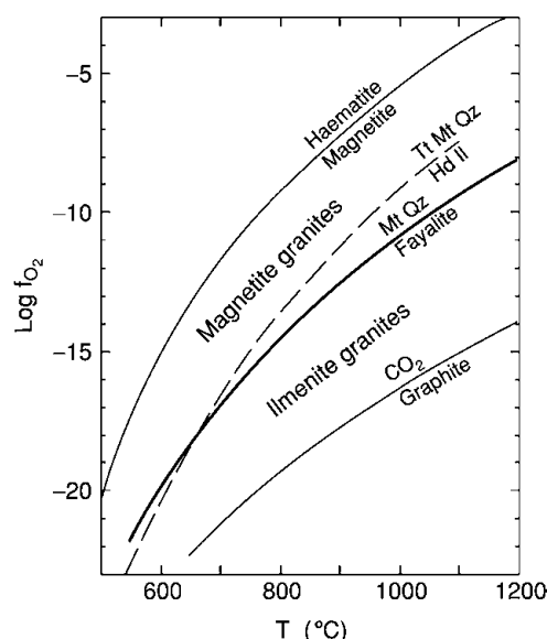
Figure 3 Plot of log f_{O_2} (oxygen fugacity) against temperature, showing the locations of commonly used buffer curves and the crystallization fields of ilmenite- and magnetite-bearing granitic rocks. Hd, hedenbergite; Il, ilmenite; Mt, magnetite; Qz, quartz, Tt, titanite.
