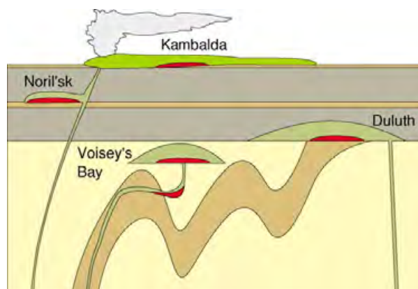
Figure 6 Cartoon of principal mechanisms for the generation and segregation of magmatic base-metal sulphides. The image shows a cross-section of the upper crust, with brown areas representing sulphur-rich crustal rocks which act as sources of sulphur for dykes and plutons of mantle-derived magma (darker green) or lava flows (lighter green). Sulphide liquid collects where it formed (Duluth), in traps within conduits or where conduits enter magma chambers (Voisey's Bay), in subvolcanic sills (Noril'sk), or in lava channels cutting through sulphidic sediments (Kambalda).
