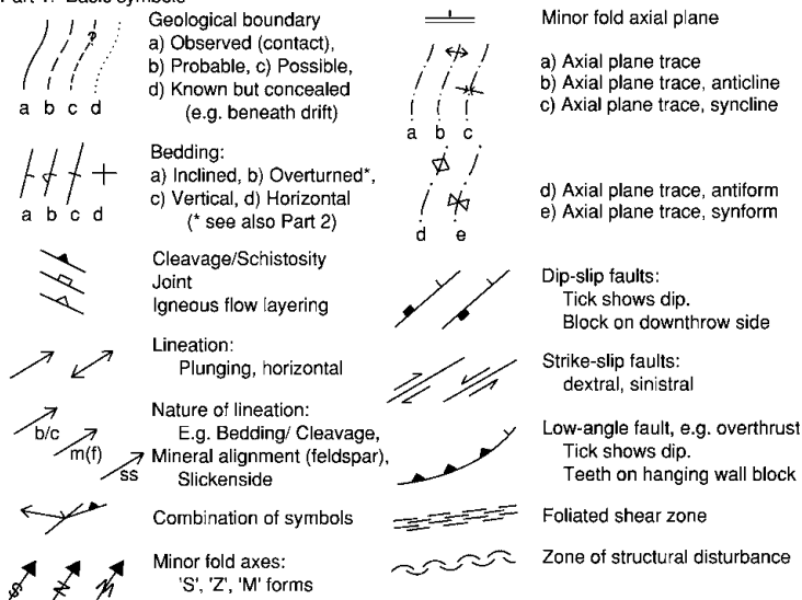
Figure 2 Geological mapping symbols.
