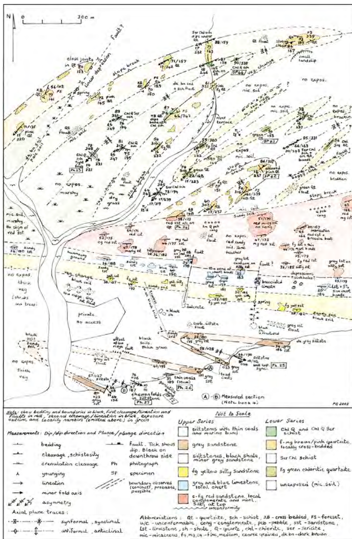
Figure 4 Example of field map entries. Map grid, contours, and locality numbers have been omitted for clarity. The map symbols would be in coloured ink. Exposures would be outlined in a continuous, not dotted, green line.
