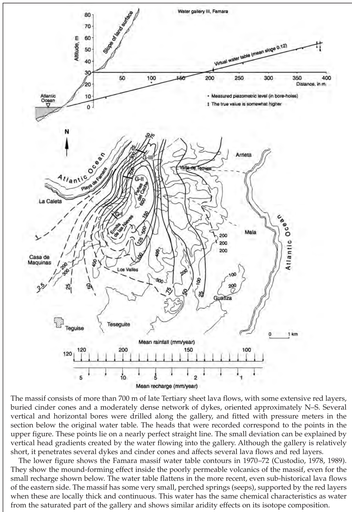
Figure 16.8 Experimental water gallery in the Famara massif, Northern Lanzarote, Canary Islands, Spain
