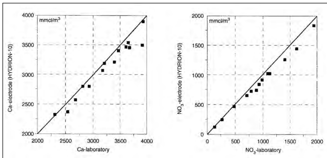
Figure 3.14 Comparison of some measured ion concentrations with conventional analytical techniques and a with set of integrated ion-selective electrodes HYDRION-10
