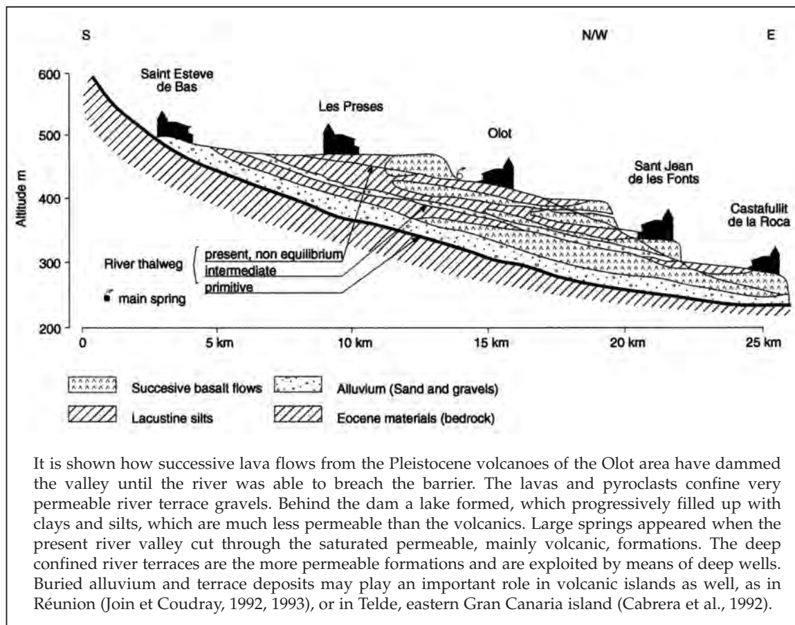
Figure 16.5 Cross section along the Fluvià river valley, Catalonia, Spain (modified from Fayas and Doménech, 1974)
