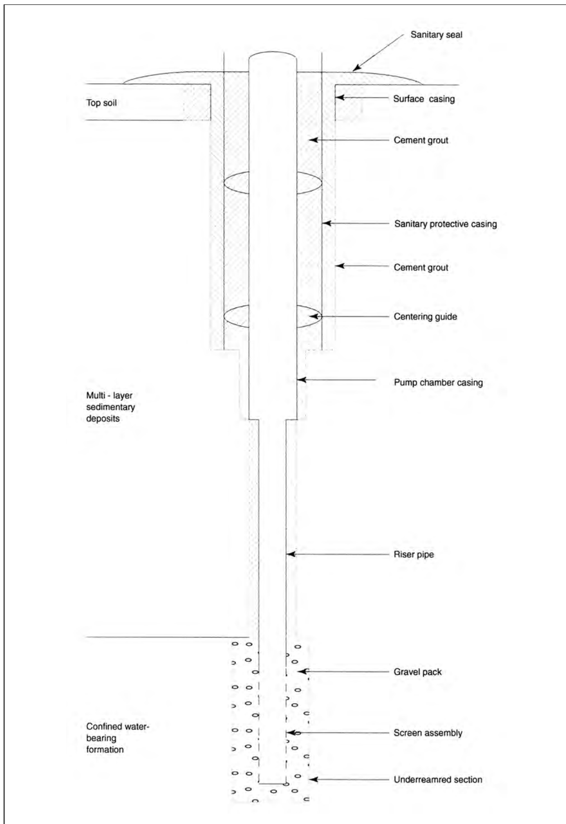
Figure 7.10 Diagram showing the main parts of a deep water well design
