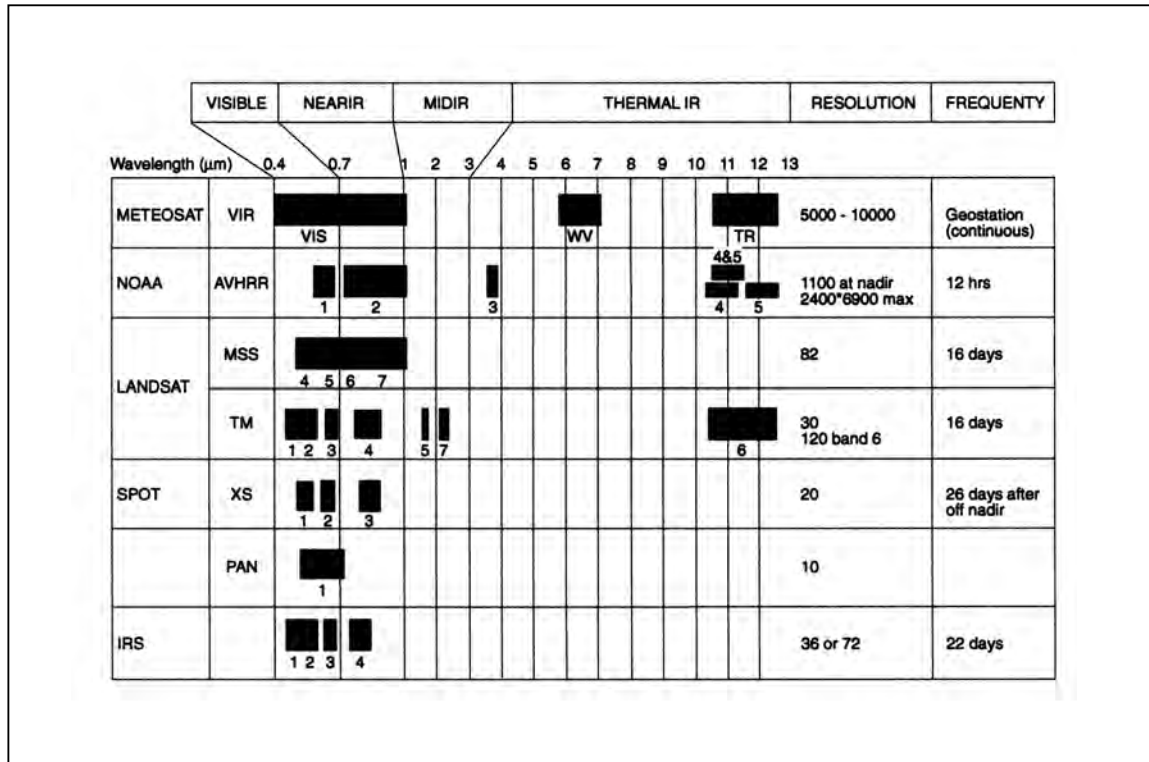
Figure 5.4 Satellite characteristics
