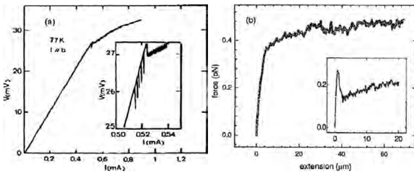
Fig. 18. (a) A plot of dc voltage-current that shows a sharp threshold for the onset of non-Ohmic regime (after [80]). (b) Force – extension curve for membrane tubulation. The inset shows another plot which is very similar to a sharp yield point followed by serrations (after [87])
