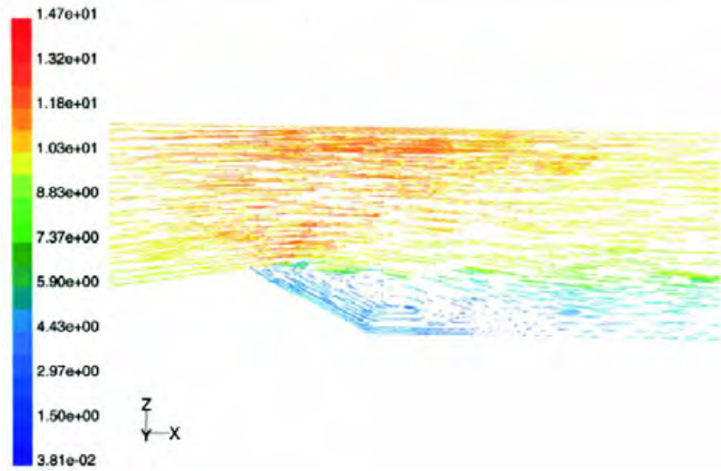
Fig. 4. Velocity field in a longitudinal cut along the central slice of a Barchan dune. One clearly sees the flow separation and a large eddy that forms in the wake of the dune
