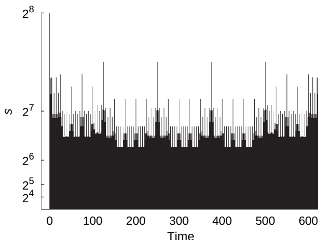
Fig. 11. For two ( regular ) Cantor sets, one moving uniformly over the other (with periodic boundary condition), the total measure of the ( shaded region in Fig. 8(b) contributing to the) overlap s has the time variation as shown here (for n = 4 )
