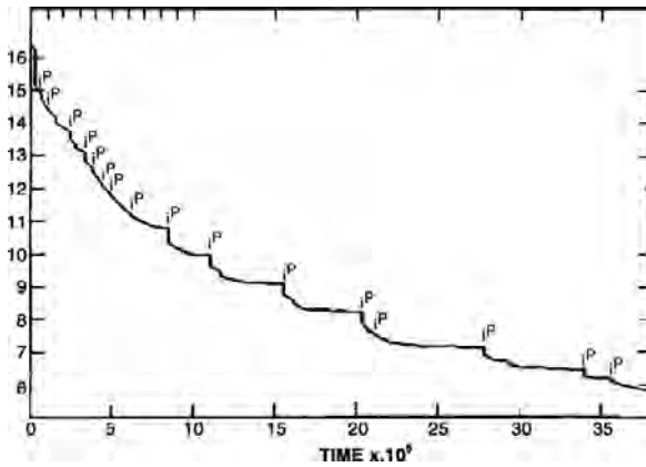
Fig. 13. Potential energy as a function of time for the aftershock sequence following a main shock. Shocks occurring on the principal segment of the fault are identified by the symbol P
