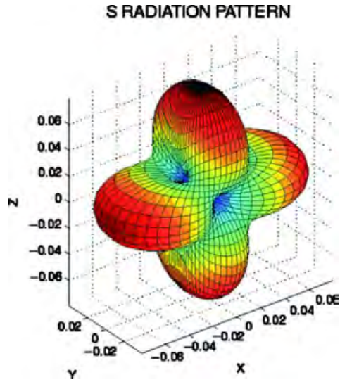
Fig. 3. This is the S radiation pattern, which is a ( spherical ) polar plot of the S amplitude A_S(\omega) radiated in direction \omega as a function of \omega , i.e. the surface r = |A_P(\omega)| . The shaded also represents the amplitude, on a scale of dark red = 1 to dark blue = 0. Compare the scales on the axes with those of Fig. 1 to see how much more energetic the S wave is than the P
