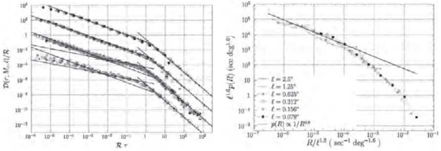
Fig. 9. ( Left ) Mixed recurrence-time densities (defined in the way of Bak et al.) and rescaled by R , for several values of \ell and M_c . The different sets of curves correspond, from top to bottom, to (i) Southern California, 1984–2001; (ii) Northern California, 1985–2003; (iii) Stationary seismicity: Southern California, 1988–1991; worldwide, 1973–2002; Japan, 1995–1998; and Spain, 1993–1997; (iv) Stationary seismicity: New Zealand, 1996–2001, and New Madrid, 1975–2002; A total of 84 distributions are shown, \ell ranging from 0.039^\circ to 45^\circ , and 1.5 \leq M_c \leq 6 . The distributions are shifted to the bottom for clarity sake. All the left tails are fit by a (decreasing) power-law with exponent 2.2, the right part of the distributions are fit by a power law with exponent 0.95 or 0.9, see [39]. ( Right ) Distribution of mean rates of occurrence for events with M \geq 2 in Southern-California, 1984–2001 (averaging 1984–1992 and 1993–2001), using diverse values of \ell . The distributions are rescaled by L^{1.6} and the straight line is a power law fit which turns out to be \propto 1/R^{0.8}
