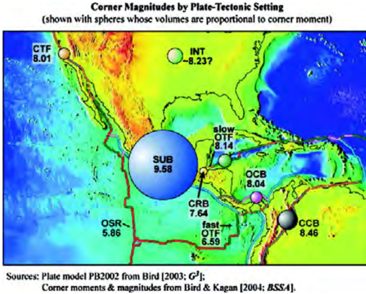
Fig. 7. Corner moment ( M_c ) distribution for eight tectonic provinces [13]. In this figure the moment magnitude is calculated using C = 6.05 in (2). For plate boundary names and abbreviations see Fig. 6
