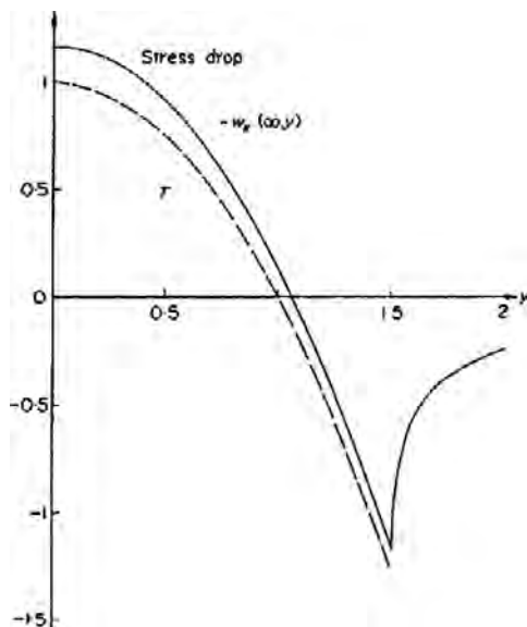
Fig. 36. Here are plotted as functions of y the dynamic stress drop T = 1 - y^2 ( dashed line ) which acts before stopping and the final static stress drop -w_x(\infty, y) , which is about 16% greater at y = 0
