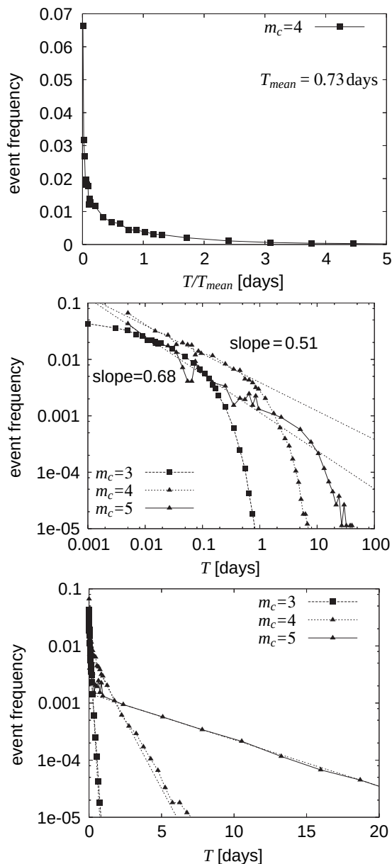
Fig. 8. The global recurrence-time distribution of large earthquakes in entire Japan generated from the JUNEC catalog. The distribution is given on a bare scale for large earthquakes with m_c = 4 [upper figure], on a double-logarithmic scale with varying m_c = 3, 4 and 5 [middle figure], and on a semi-logarithmic scale with varying m_c = 3, 4 and 5 [lower figure]
