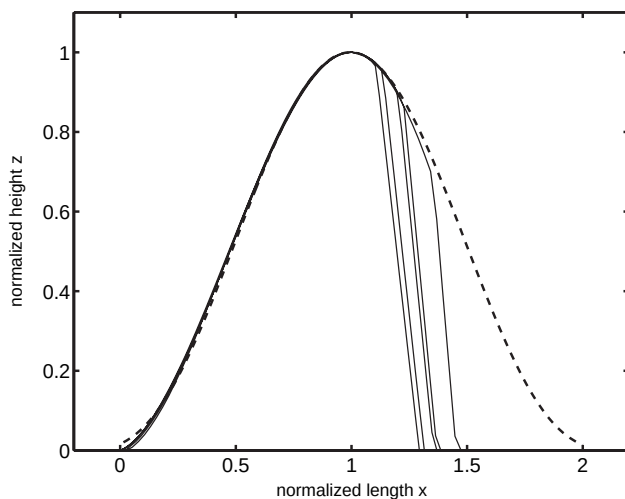
Fig. 17. Numerical calculation of the normalized longitudinal profiles of the dunes. A fit with \cosh^4(x) ( dashed line ) reproduces quite well the windward side. The shear velocity is u_* = 0.5 \text{ ms}^{-1} (from [40])
