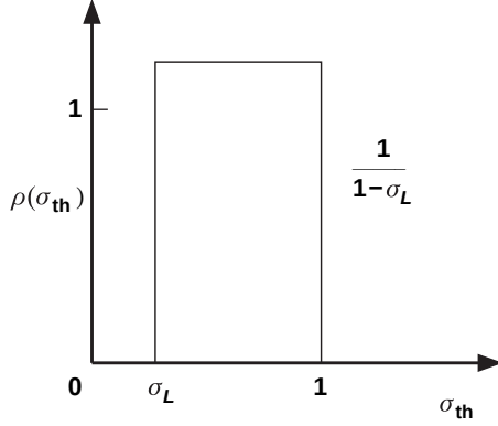
Fig. 5. The fibre breaking strength distribution \rho(\sigma_{\text{th}}) considered for studying elastic-plastic-type non-linear deformation behaviour of the equal-load-sharing model
