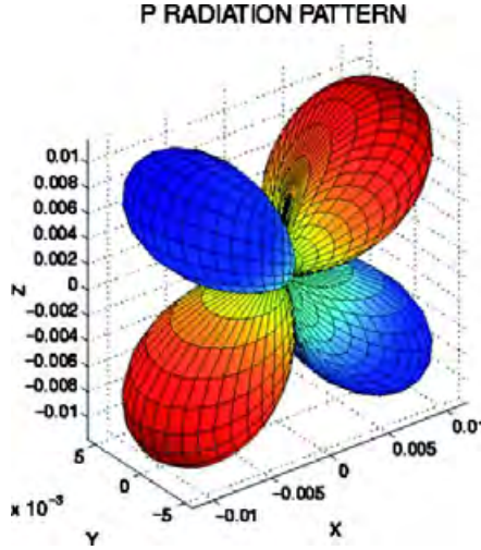
Fig. 1. This is the P radiation pattern, which is a ( spherical ) polar plot of the P amplitude A_P(\omega) radiated in direction \omega as a function of \omega , i.e. the surface r = |A_P(\omega)| . The shaded also represents the signed amplitude, on a scale of dark red = 1 to dark blue = -1
