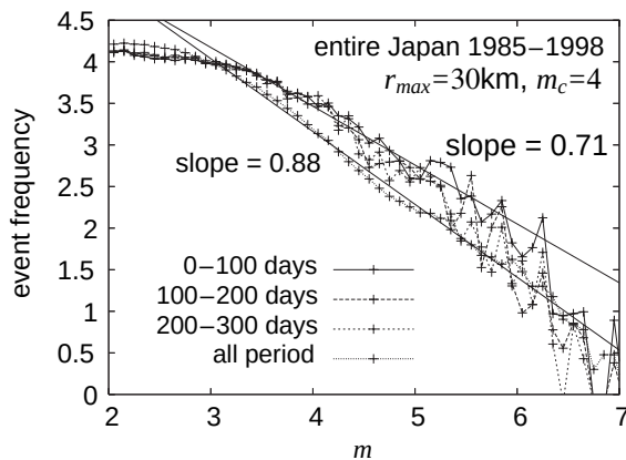
Fig. 23. The time-resolved local magnitude distribution of earthquakes in Japan after the mainshock of m > m_c = 4 , generated from the JUNE C catalog
