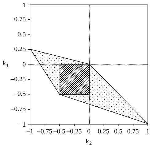
Figure 4.2 Acceptable domains for numerical values of the specified elements k_1(= s_{12}) and k_2(= s_{23}) (after Gandin and Murphy 1992)
