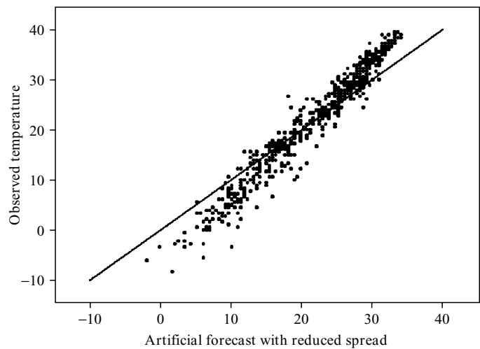
Figure 2.9 Scatterplot of observed high temperatures (°C) for Oklahoma City against artificial forecasts that have less spread than the observations
