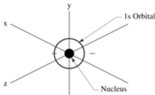
Figure 2-3(a) 1s orbital.
