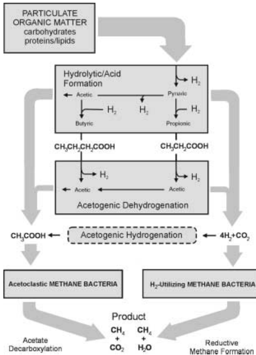
Figure 8-50 The groups of bacteria and the principal transformations performed in converting organic particulates to methane and carbon dioxide during anaerobic digestion. (After Mosey and McInerny and Bryant. Each rectangle represents a bacterial group).
