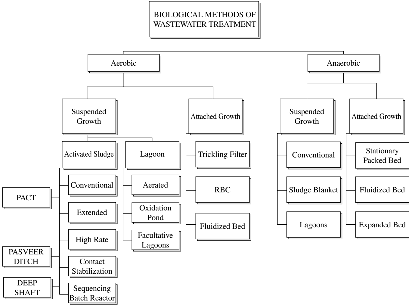
Figure 8-21 Aerobic and anaerobic methods of wastewater treatment.
