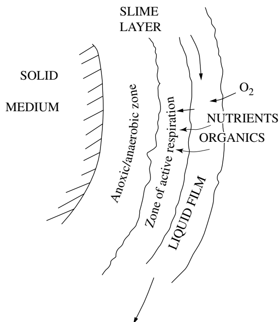
Figure 8-44 Characteristics of attached growth slime layer.
