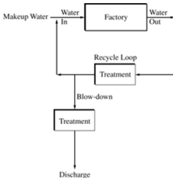
Figure 7-1 Example of a water recycle loop with treatment and blow-down.
