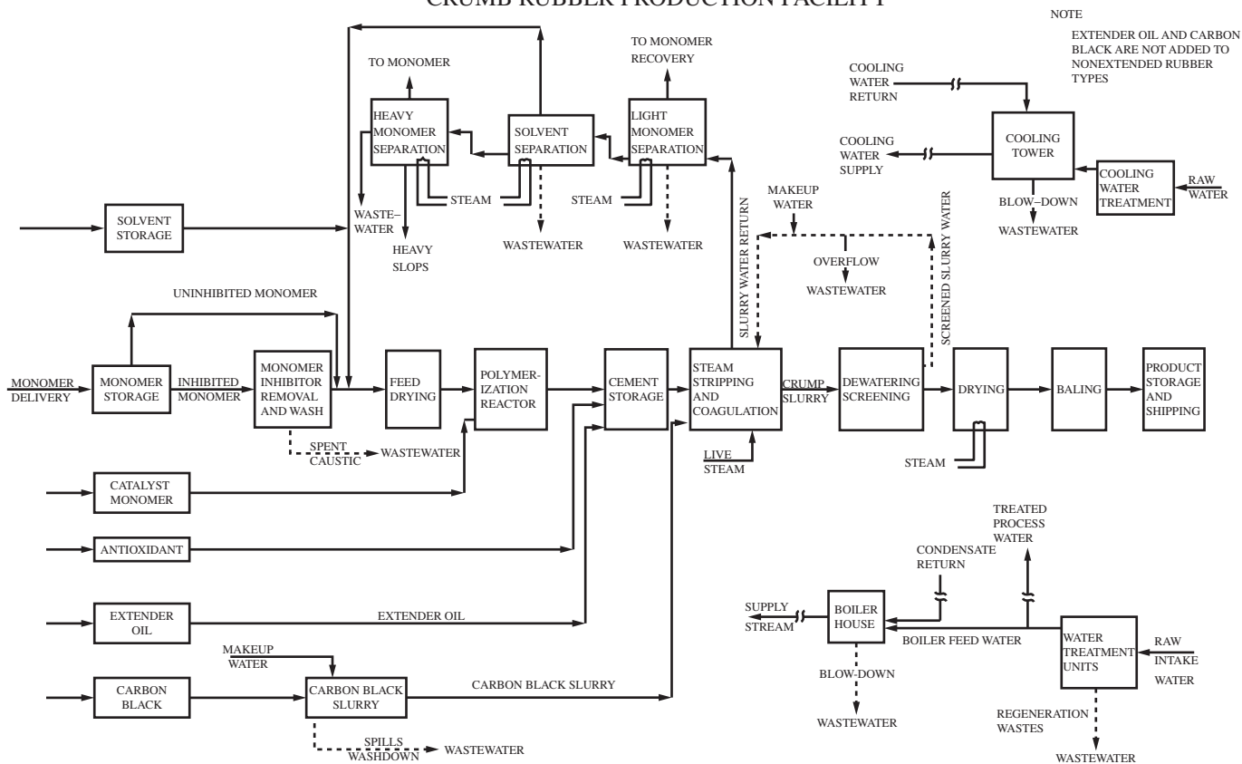
GENERAL WATER FLOW DIAGRAM FOR A SOLUTION POLYMERIZED CRUMB RUBBER PRODUCTION FACILITY
