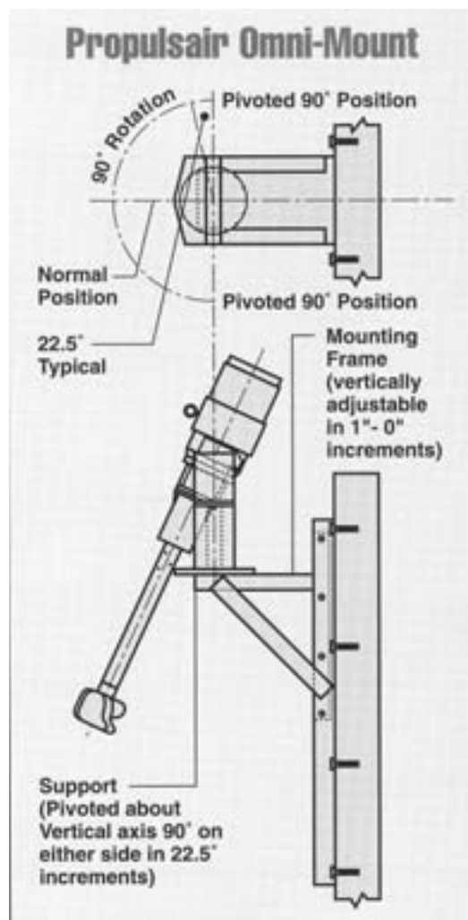
Figure 8-38(m) Alternative device for aeration. (Drawing courtesy of Eimco Process Equipment, a Baker Hughes Company.)
