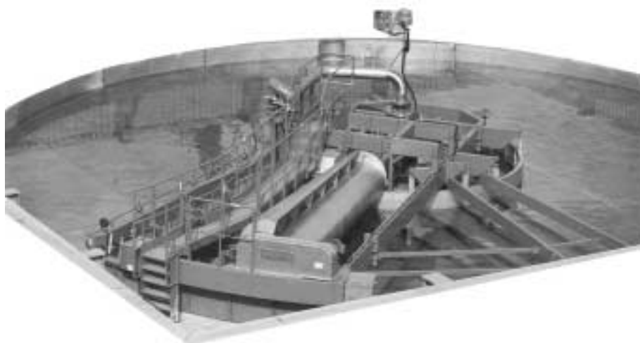
Figure 8-98(c) Gravity flotation and harvesting equipment. (Courtesy of KWI.)
