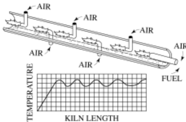
Figure 9-7(f) Elements of a rotary kiln incinerator—axial-burner concept. (From Freeman, © 1989. Reprinted by permission of McGraw-Hill, Inc.)
