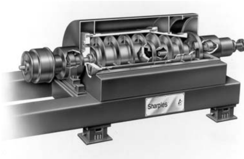
Figure 8-95 Diagram of a solid bowl centrifuge. (Courtesy of Alfa Laval, Inc.)
