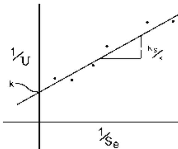
Figure 8-20 Plot of 1/U versus 1/S_e
