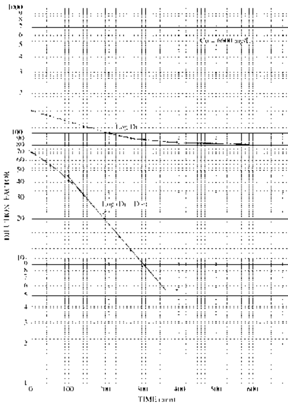
Figure 8-88(b) Dilution factor vs. time.
