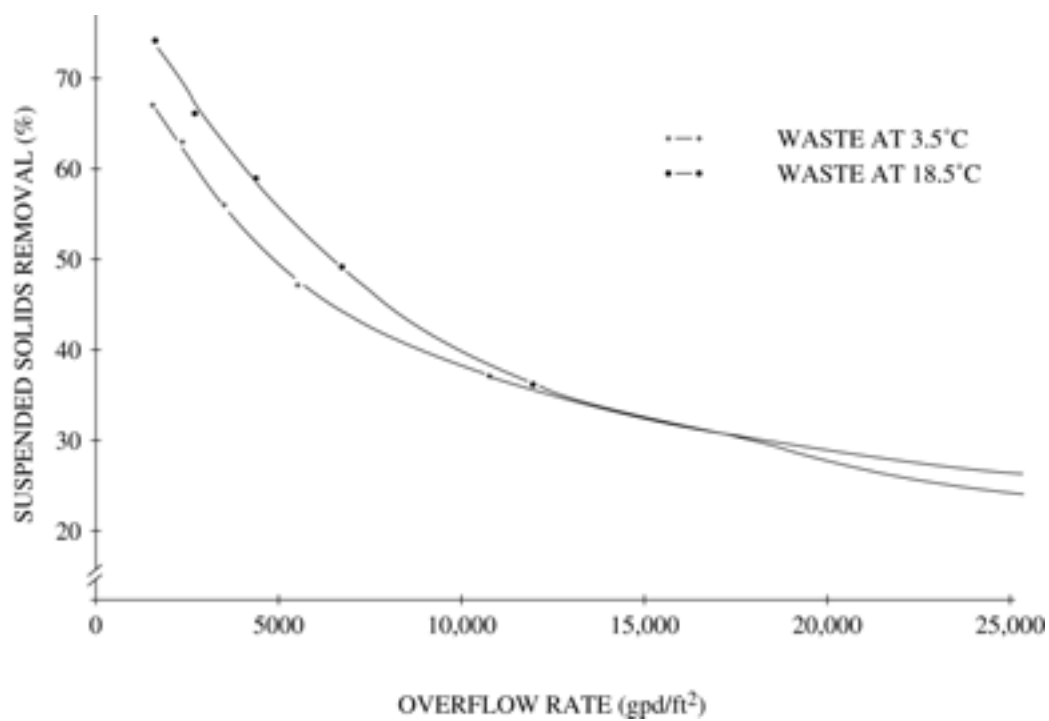
Figure 8-82 Suspended solids removal vs. overflow rate.
