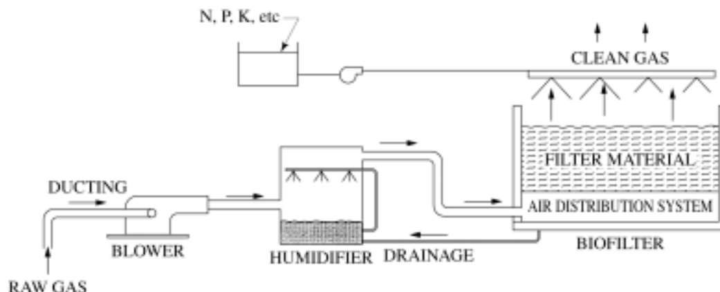
Figure 10-16 Schematic of a typical biofilter system.
