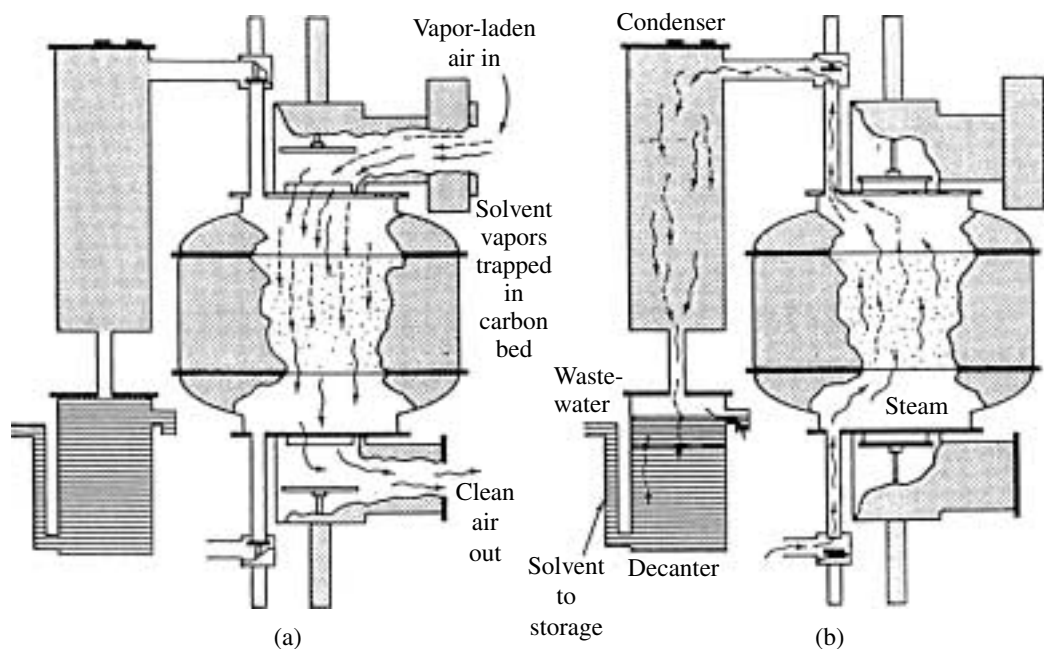
Figure 10-9 Activated carbon adsorption system for removal of gaseous pollutants and other chemicals from gas streams. (From Buonicor and Davis, © 1992. Reprinted by permission of John Wiley and Sons, Inc.)
