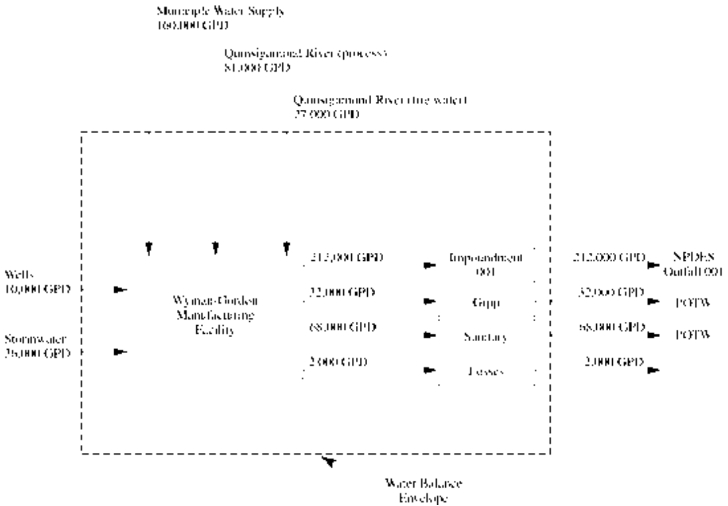
Figure S-2 Water balance before recycle.
