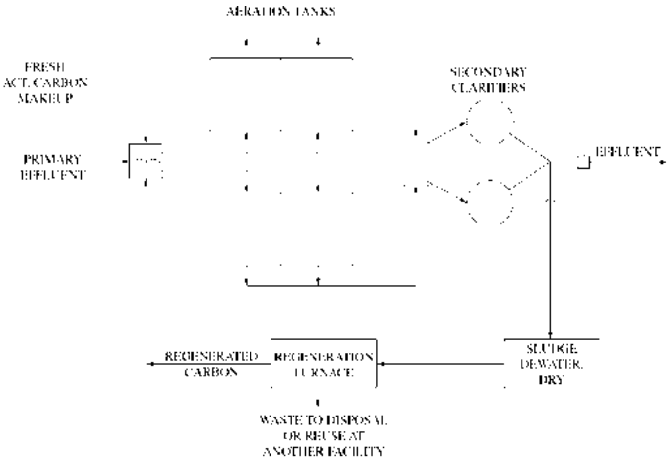
Figure 8-32 PACT modification of the activated sludge process, complete-mix configuration.
