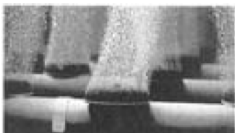
Figure 8-38(c) Alternative device for diffusion: Dome diffuser. (Photo courtesy of Parkson Corporation.)
