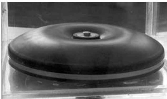
Figure 8-38(e) Alternative device for diffusion: Fine-bubble membrane diffuser. (Photo courtesy of Eimco Process Equipment, a Baker Hughes Company.)
