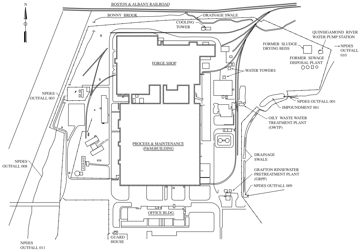
Figure 5-1 Site plan.
