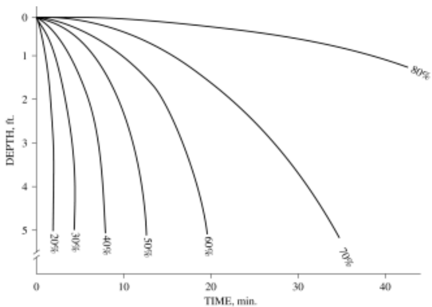
Figure 8-80 Solids removal for depth vs. time (18.5°C).
