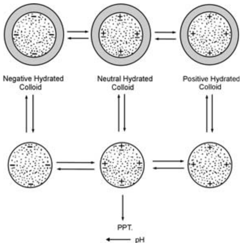
Figure 8-15 Diagrammatic representation of the various types of colloids. The colloids in the upper row are lyophillic; those below are lyophobic. pH increases from right to left.
