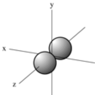
Figure 2-4(c) 2p_z orbital.
