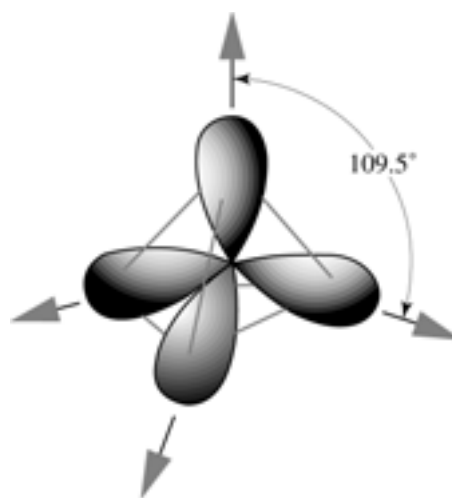
Figure 2-8 The four \text{sp}^3 orbitals of an atom of carbon.
