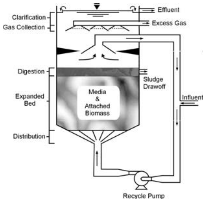
Figure 8-54 Anaerobic attached film expanded bed reactor (AAFEB).
