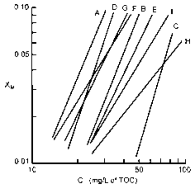
Figure 8-106 Composite plot of isotherms of three different carbon products.
