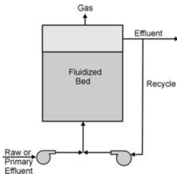
Figure 8-55 Anaerobic fluidized bed reactor.
