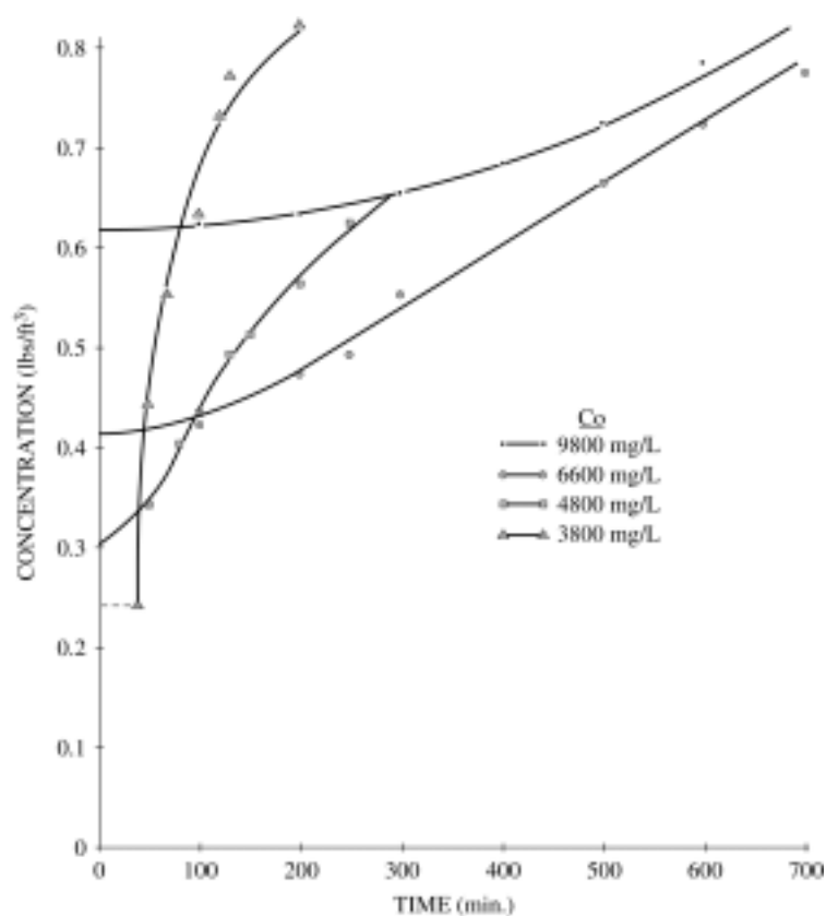
Figure 8-85 Sludge concentration vs. time.
