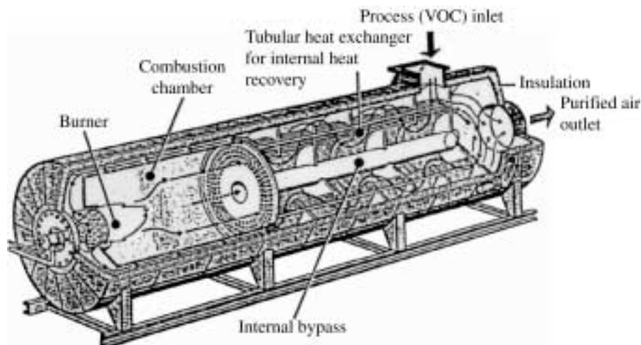
Figure 10-13 Basic components of a thermal oxidizer for air pollution control. (From Freeman, © 1989. Reprinted by permission of McGraw-Hill, Inc.)
