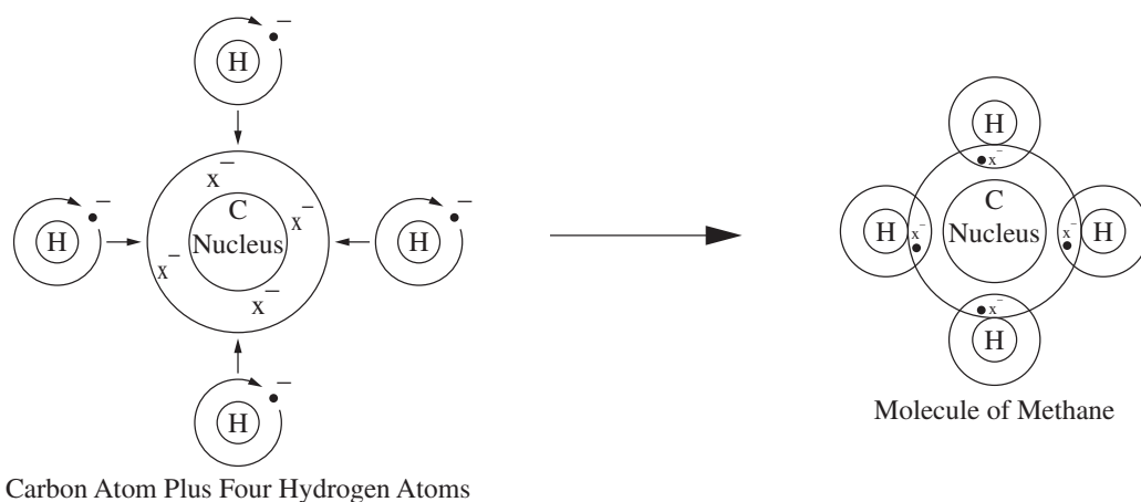
Figure 2-10 A carbon atom forms covalent bonds with each of four hydrogen atoms to produce a molecule of methane.
