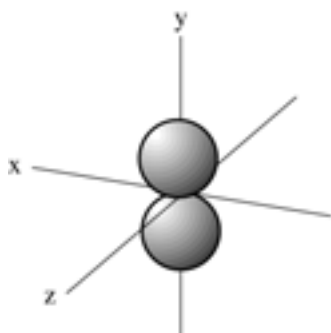
Figure 2-4(b) 2p_y orbital.
