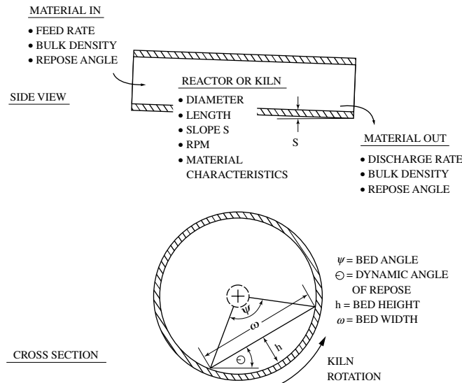
Figure 9-7(a) Elements of a rotary kiln incinerator—axial movement through the reactor. (From Freeman, © 1989. Reprinted by permission of McGraw-Hill, Inc.)
