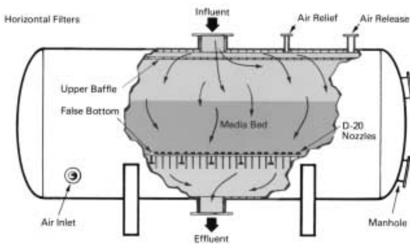
Figures 8-73(c) Pressure and vacuum filters. (Courtesy of IDI/Infilco Degremont, Inc.)
