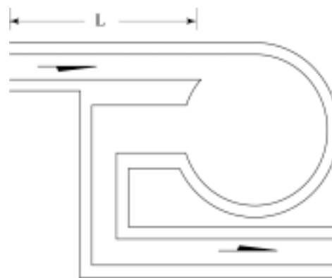
Figure 8-93(b) Swirl separator. (Courtesy of Smith & Loveless.)
