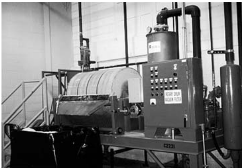
Figures 8-73(f) Pressure and vacuum filters. (Courtesy of Waterlink Separators, Inc.)
