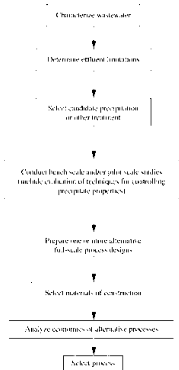
Figure 8-10 Suggested procedure for developing a treatment system.
