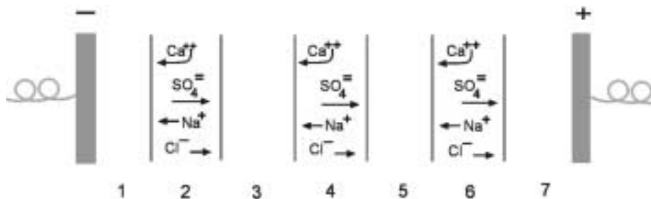
Figure 8-66 Schematic diagram of an electro dialysis cell.
