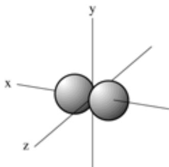
Figure 2-4(a) 2p_x orbital.
