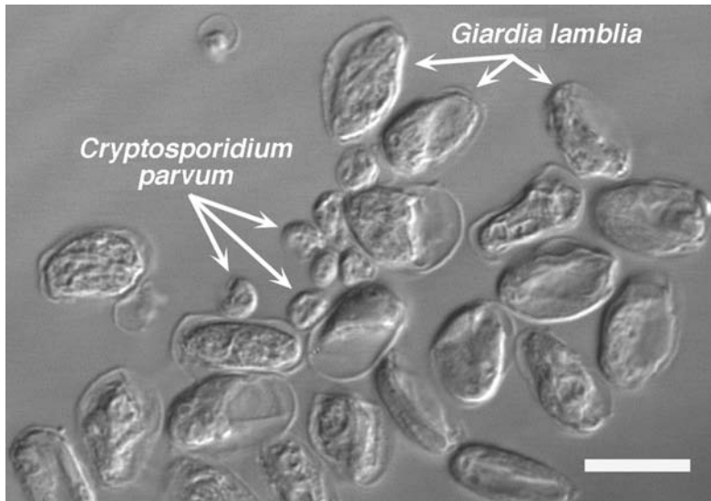
Figure 9.3 Two parasites in drinking water ( Cryptosporidium parvum and Giardia lamblia from animal feces). Photo credit: H. D. A. Lindquist, US EPA (Scale bar, 10 \mu m). Source: US EPA Microbiology
