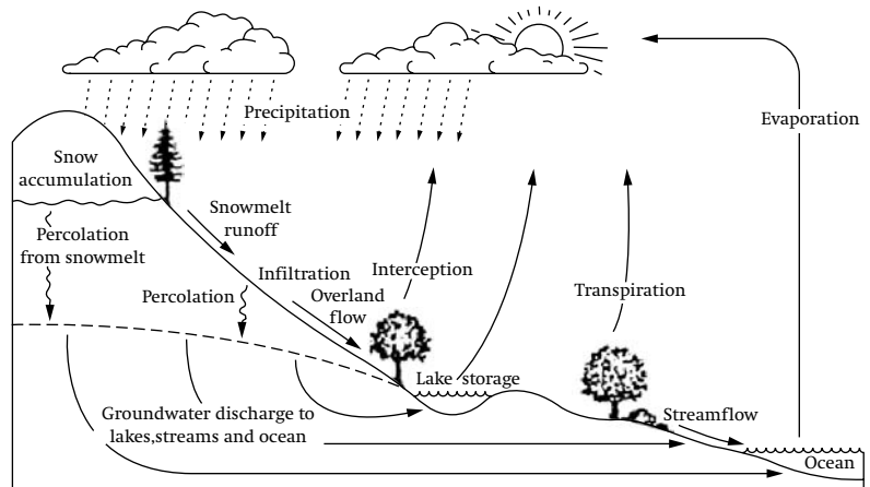
Figure 9.1 Movement of water in the environment. Source: New South Wales Environmental Protection Authority, Australia
