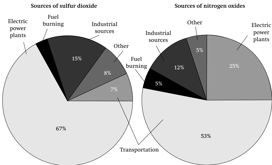
Figure 6.1 Sources of pollutants that form acid deposition
