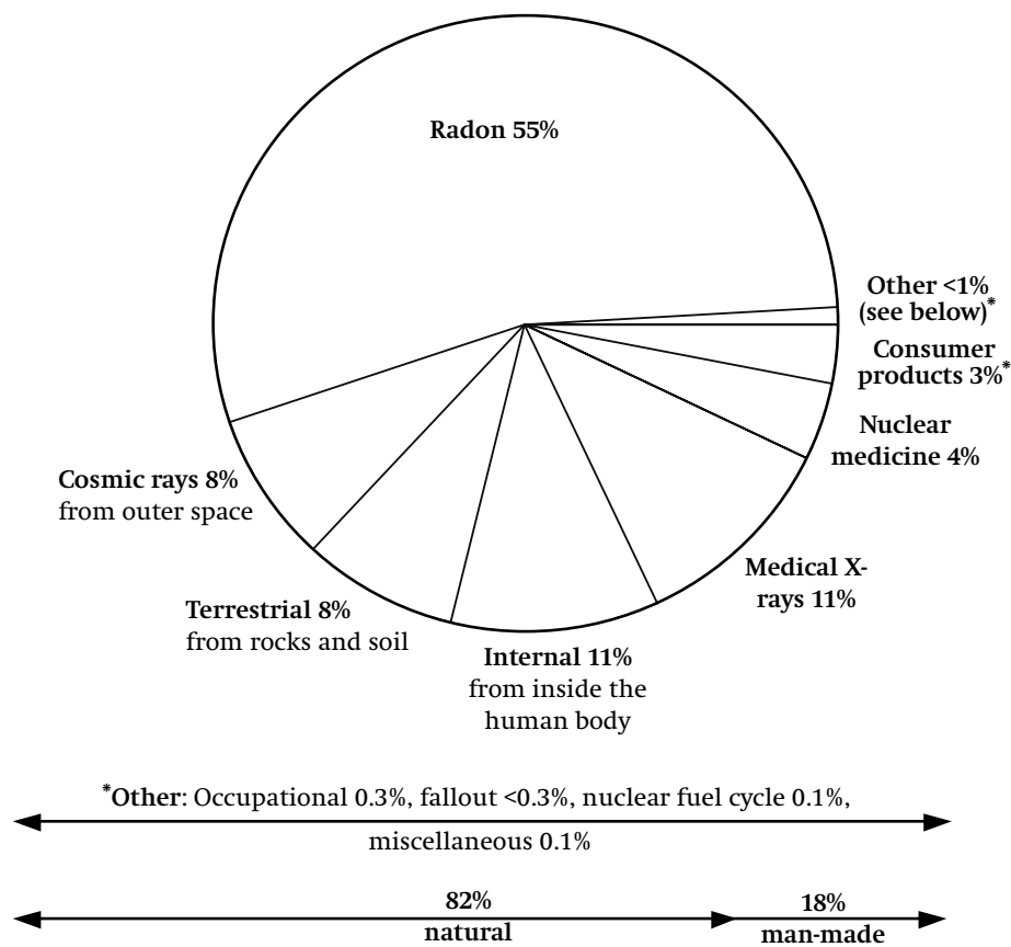
Figure 17.4 Sources of ionizing radiation exposure to the US population
