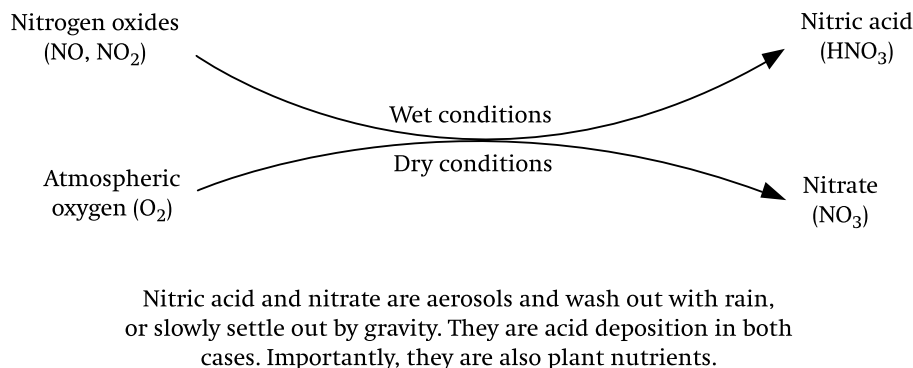
Figure 5.3 Transforming NO x gases to nitric acid and nitrate
