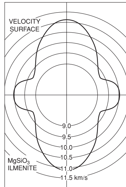
Fig. 20.13 Variation of compressional velocity with direction in the ilmenite form of \text{MgSiO}_3 . This is a stable mineral below about 500 km in cold slabs. \text{MgSiO}_3 -ilmenite is a platy mineral and may be oriented by stress, flow and recrystallization in the slab. Ice (in glaciers) and calcite (in marble) have similar crystal structures and are easily oriented by flow, giving anisotropic properties to ice and marble masses. The deep slab may also be anisotropic.
