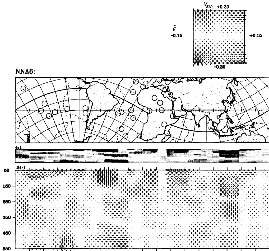
Fig. 20.8 S velocity in the upper mantle along the cross-section shown. Note low velocities at shallow depth under the western Pacific, replaced by high velocities at greater depth. The eastern Pacific is slow at all depths. The Atlantic is fast below 400 km.
