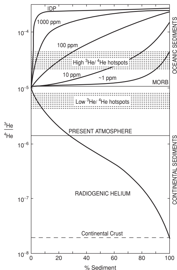
Fig. 16.6 Materials found at the surface of the Earth exhibit a range of 4 orders of magnitude in ^3\text{He}/^4\text{He} ratios. Sediments on the seafloor collect interplanetary dust particles (IDP) and these raise the helium content and helium ratio of deep sea sediments in proportion to their abundances of IDP. Continental sediments have very low ratios because of high U and Th and age. Subduction of these materials contribute to the isotopic heterogeneity of the mantle. High ^3\text{He}/^4\text{He} ratios in mantle materials can also be due to trapping of ancient gases – in U-poor environs – from degassing of rising magmas.
