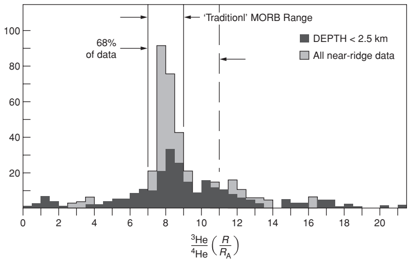
Fig. 16.1 Histogram of helium isotopes measured in samples along the global spreading ridge system, including new ridges, back-arc basins and near-ridge seamounts. In most compilations much of the right-hand side of the distribution is missing since values higher than about 9 R/R_A are filtered out. High values are attributed to plume contamination. Anomalous sections of the global ridge system are also avoided. The traditional MORB range, after filtering the data, is from 7–9 R/R_A . High R values are found in depleted components of basalts that have been identified as the most common mantle component, possibly peridotite. The high R/R_A carriers may be peridotites or olivines with low U/He ratios. The helium may be acquired from wall-rocks, by ascending magmas.
