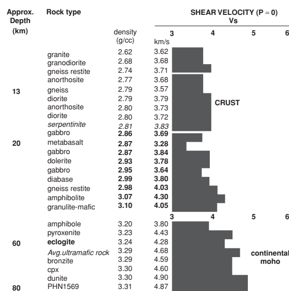
Fig. 8.3 Crustal minerals.
