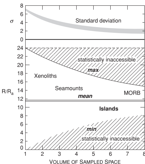
Fig. 16.7 An illustration of the central limit theorem. Midocean ridges sample very large volumes whereas seamounts and xenoliths are small-scale small-volume samples that more faithfully represent the true heterogeneity of the mantle. In this example, the range of R/R_A in the mantle is from 0 to 24. This complete range will only be evident by taking many small-scale small-volume samples. Large islands and spreading ridges average over large volumes and cannot access the whole range. The presence of high values in OIB samples does not imply that these samples are from a different part of the mantle.
