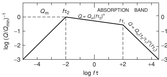
Fig. 19.4 Schematic illustration of an absorption band.
