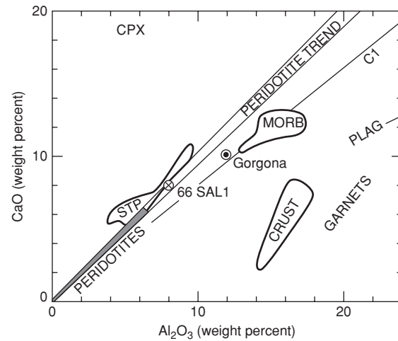
Fig. 15.4 CaO versus \text{Al}_2\text{O}_3 for igneous rocks and minerals. Note that peridotites and STP are CaO-rich compared to CI chondrites, and meteorites in general, while the continental crust is \text{Al}_2\text{O}_3 -rich. MORB falls on the CI trend, possibly suggesting that it is an extensive melt of primitive mantle. Gorgona is an island in the Pacific that has komatiitic magmas. The solar \text{CaO}/\text{Al}_2\text{O}_3 ratio is slightly higher than peridotites (Chapter 1).
