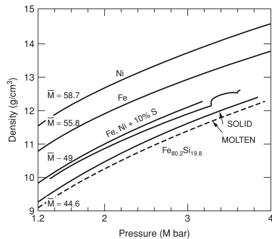
Fig. 10.1 Estimated densities of Fe, Ni and some Fe-rich alloys compared with core densities. The estimated reduction in density due to melting is shown (dashed line) for one of the alloys.
