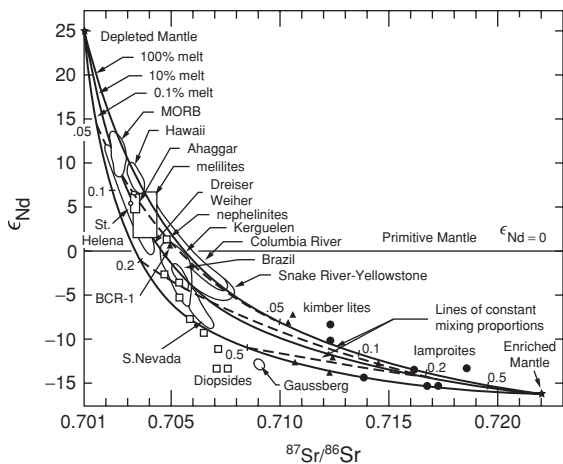
Fig. 17.2 \epsilon_{\text{Nd}} versus ^{87}\text{Sr}/^{86}\text{Sr} for mixtures involving a depleted magma or residual fluids from such a magma after crystal fractionation, and an enriched component (EM). Plots such as this are known as mantle arrays or multiple isotope plots .
