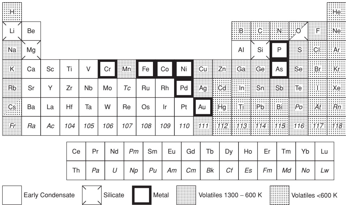
Fig. I.1 Condensation behavior of the elements. Short-lived radioactive elements are shown in italics (after Morgan and Anders, 1980).
