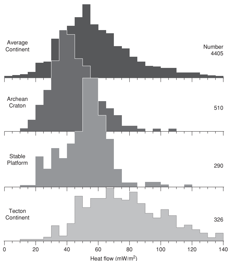
Fig. 26.3 Continental heat flow data.
