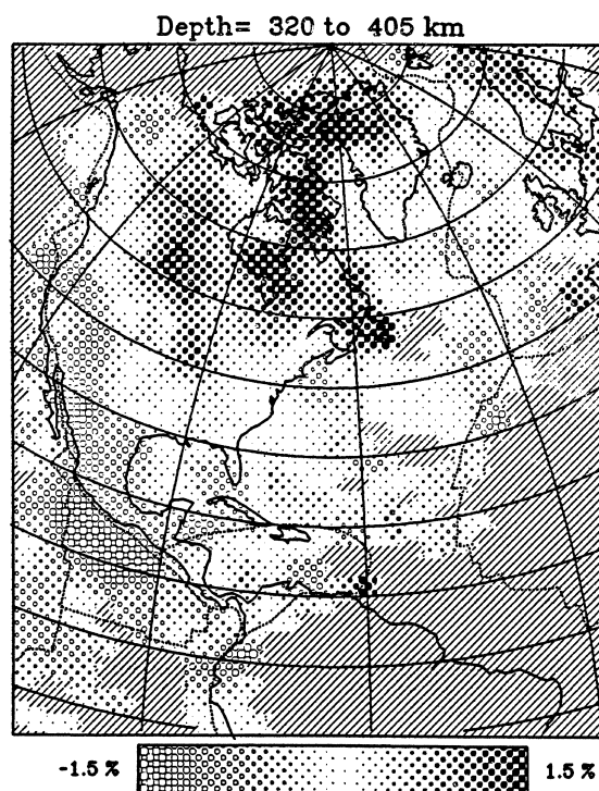
Fig. 11.11 SH velocities in the upper mantle at depths of 320 to 405 km (after Grand, 1986).
