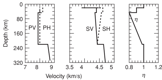
Fig. 8.5 Velocity-depth profiles for the average Earth, as determined from surface waves (Regan and Anderson, 1984). From left to right, the graphs show P-wave velocities (vertical and horizontal), S-wave velocities (vertical and horizontal) and an anisotropy parameter (1 represents isotropy).
