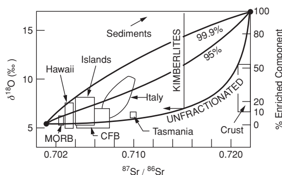
Fig. 17.4 \delta^{18}\text{O} versus ^{87}\text{Sr}/^{86}\text{Sr} for magmas, oceanic sediments, kimberlites and continental crust. Mixing curves are shown for various degrees of crystal removal from the depleted end-member. Oxygen fractionation is ignored in this calculation.
