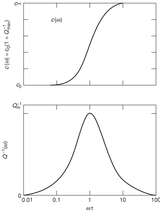
Fig. 19.1 Q^{-1} and phase velocity as a function of frequency for a standard linear solid with a single relaxation time.
