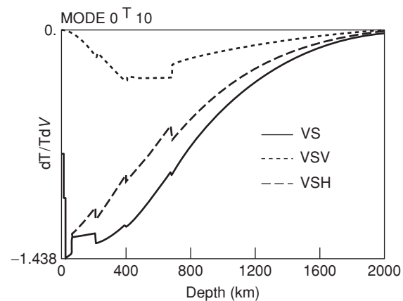
Fig. 20.14 Partial derivatives for a relative change in period of toroidal mode (Love wave) {}_0T_{10} due to a change in shear velocity as a function of depth. The solid line gives the isotropic partial derivative. The dashed lines give the effect of perturbations in two components of the velocity. Period is 720 s (after Anderson and Dziewonski, 1982).
