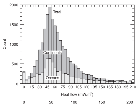
Fig. 26.4 Histograms of heat flow observations. [continental oceanic heat flow]
