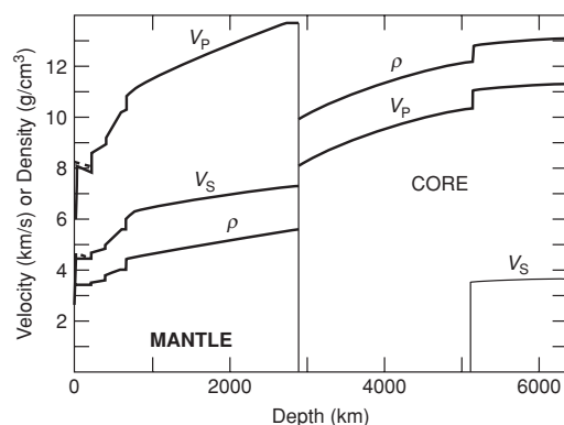
Fig. 8.1 The Preliminary Reference Earth Model (PREM). The model is anisotropic in the upper 220 km. Dashed lines are the horizontal components of the seismic velocity (after Dziewonski and Anderson, 1981).
