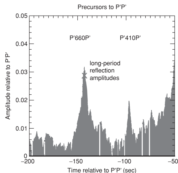
Fig. 9.3 Stacked seismograms of P'P' precursors showing the major seismic discontinuities and many minor ones (Xu et al. , 2003).
