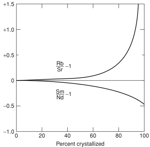
Fig. 25.5 Variation of the normalized Rb/Sr and Sm/Nd ratios in the melt fraction of a crystallizing eclogite cumulate. Equilibrium crystallization is assumed. The fractionation factor in the melt increases as freezing progresses. If melt extracts from this layer are the enriching fluids for upper-mantle metasomatism, then enrichment will increase as crystallization proceeds. Extents of melting and crystallization depend on depth and lateral locations as well as on time. Aggregated melts from a melting regime will have a variety of ratios. The crystalline residue is assumed to be 50:50 garnet: clinopyroxene.
