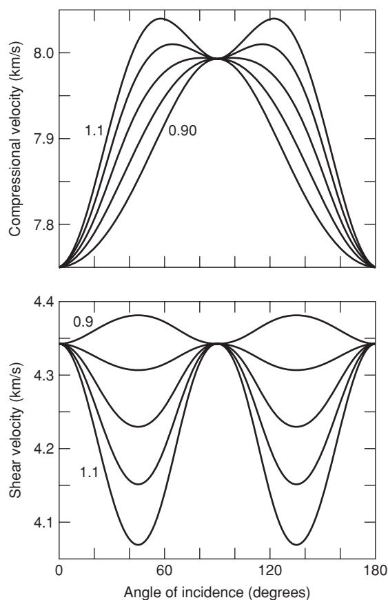
Fig. 20.4 P and S velocities as a function of angle of incidence relative to the symmetry plane and an anisotropic parameter, which varies from 0.9 to 1.1 at intervals of 0.05. Parameters are V_{PV} = 7.752 , V_{PH} = 7.994 , V_{SV} = 4.343 , all in km/s (after Dziewonski and Anderson, 1981).
