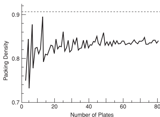
Fig. 4.6 When tiles of a given size and shape are packed on a sphere, without overlap, the packing density depends on the number n . The optimal packing density is achieved for n = 12 . This figure is for spherical caps but other shapes give similar results. The voids between the tiles have dimensions of order 10–15% of the tile dimensions so only small tiles or plates can be accommodated in the interstices (after Clare and Kepert, 1991).
