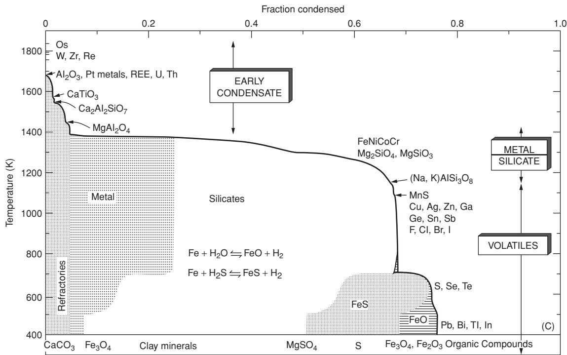
Fig. I.2 Condensation of a solar gas at 10^{-4} atm (after Morgan and Anders, 1980)
