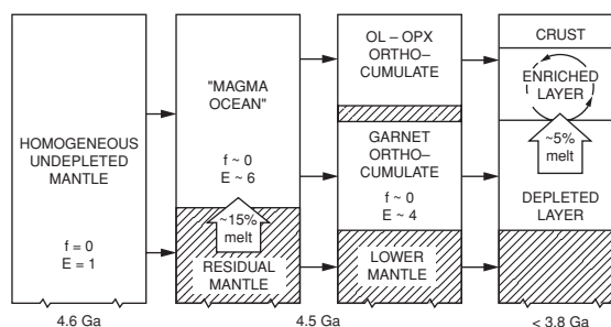
Fig. 25.1 Differentiation of a planet during accretion and early high-temperature evolution. E is the enrichment of incompatible elements, relative to the starting materials. These elements have low crystal-melt partition coefficients and therefore readily enter the melt fraction. f is the fractionation factor and gives the ratio of two incompatible elements in the melt, expressed as the difference from the starting material. Very incompatible elements occur in the same ratio in melts as in the original, or primitive, material. Isotopic ratios of these elements will evolve at the same rate as in primitive material. A magma ocean will therefore be enriched but unfractionated. As the magma ocean crystallizes, the fractionating crystals will either float or sink, leaving behind an enriched, fractionated residual liquid layer. This fluid may permeate the shallow mantle, giving an enriched geochemical signature to this region, and to the continental crust. The large difference in crystallization temperature and density of olivine–orthopyroxene (ol–opx), garnet, plagioclase and so on, means that mineralogically distinct regions can form in early Earth history.
