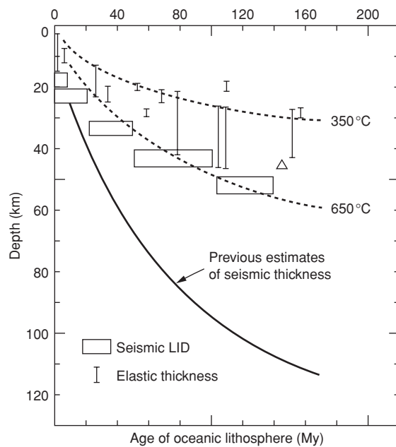
Fig. 8.4 The thickness of the lithosphere as determined from flexural loading studies and surface waves. The upper edges of the open boxes gives the thickness of the seismic LID (high-velocity layer, or seismic lithosphere). The lower edge gives the thickness of the mantle LID plus the oceanic crust (Regan and Anderson, 1984). The LID under continental shields is about 150–250 km thick.
