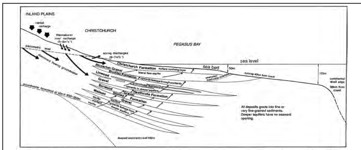
Figure 5.6.4.1 Aquifer-aquiclude sequence underlying the city of Christchurch on the Canterbury Plains (Brown, 1994)
