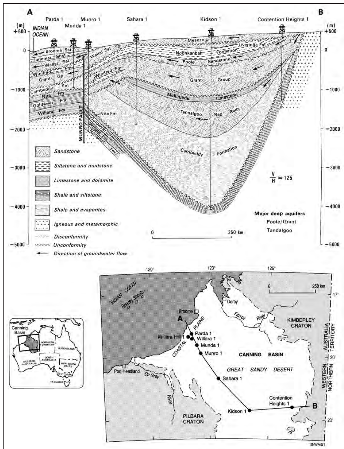
Figure 5.6.6 The Canning Basin, in the northwest of the continent
