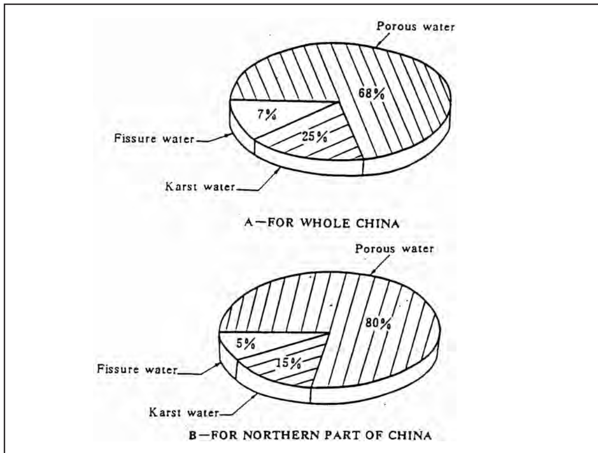
Figure 5.2.3.2.2 Percentage of various types of water well fields
