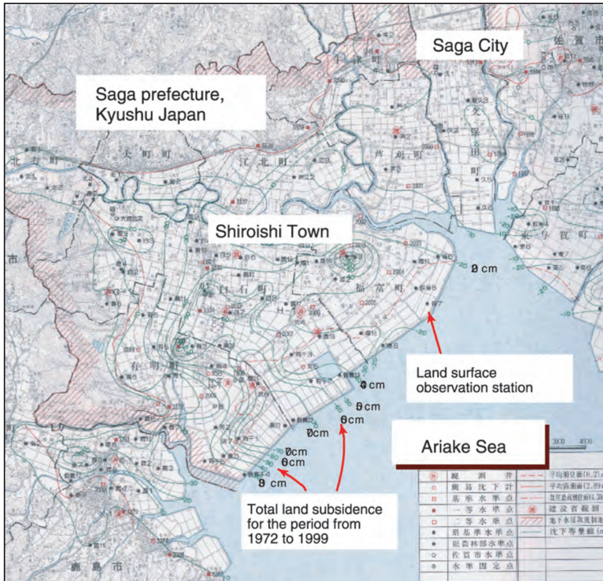
Figure 5.2.4.1.2.5 Total land subsidence from February 1972 to February 1999. The contours represent areas of equi-land subsidence, dots are the monitoring stations of groundwater level (Courtesy of Saga Prefecture Office), 1999)
