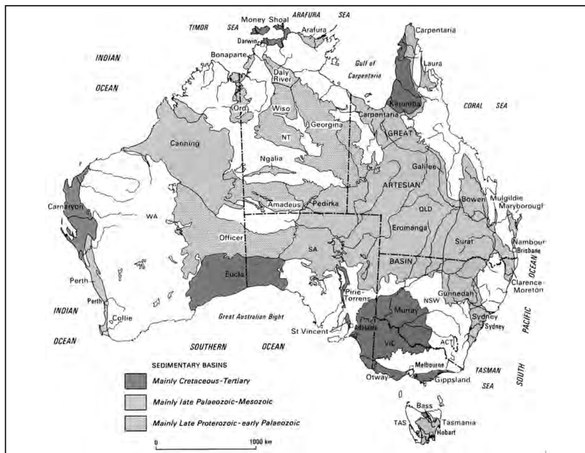
Figure 5.6.2 Number of major sedimentary basins
