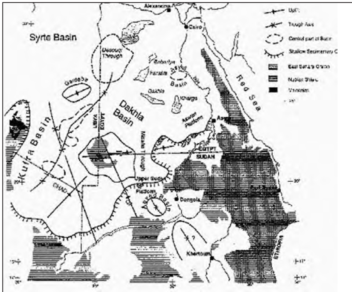
Figure 5.5.3.1.1 Structural highs and lows in the Nubian Basin (Source: Thorweihe and Heini, 1996)
