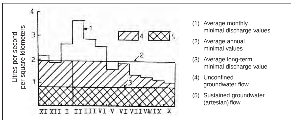
Figure 4.2.1.2 Specific river discharge values as indices of groundwater flow (after W. Wundt in: Keller, 1965)
