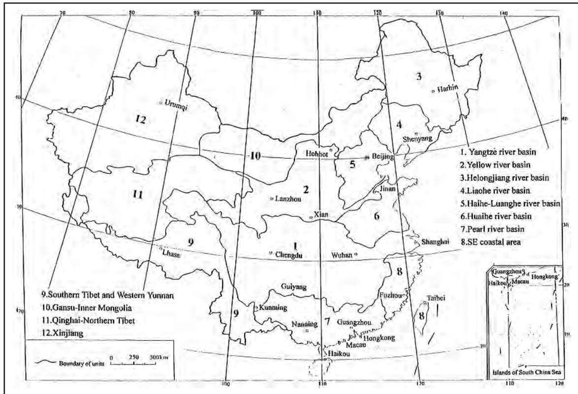
Figure 5.2.3.2.2.1 Sketch map, showing large hydrogeologic units in China
