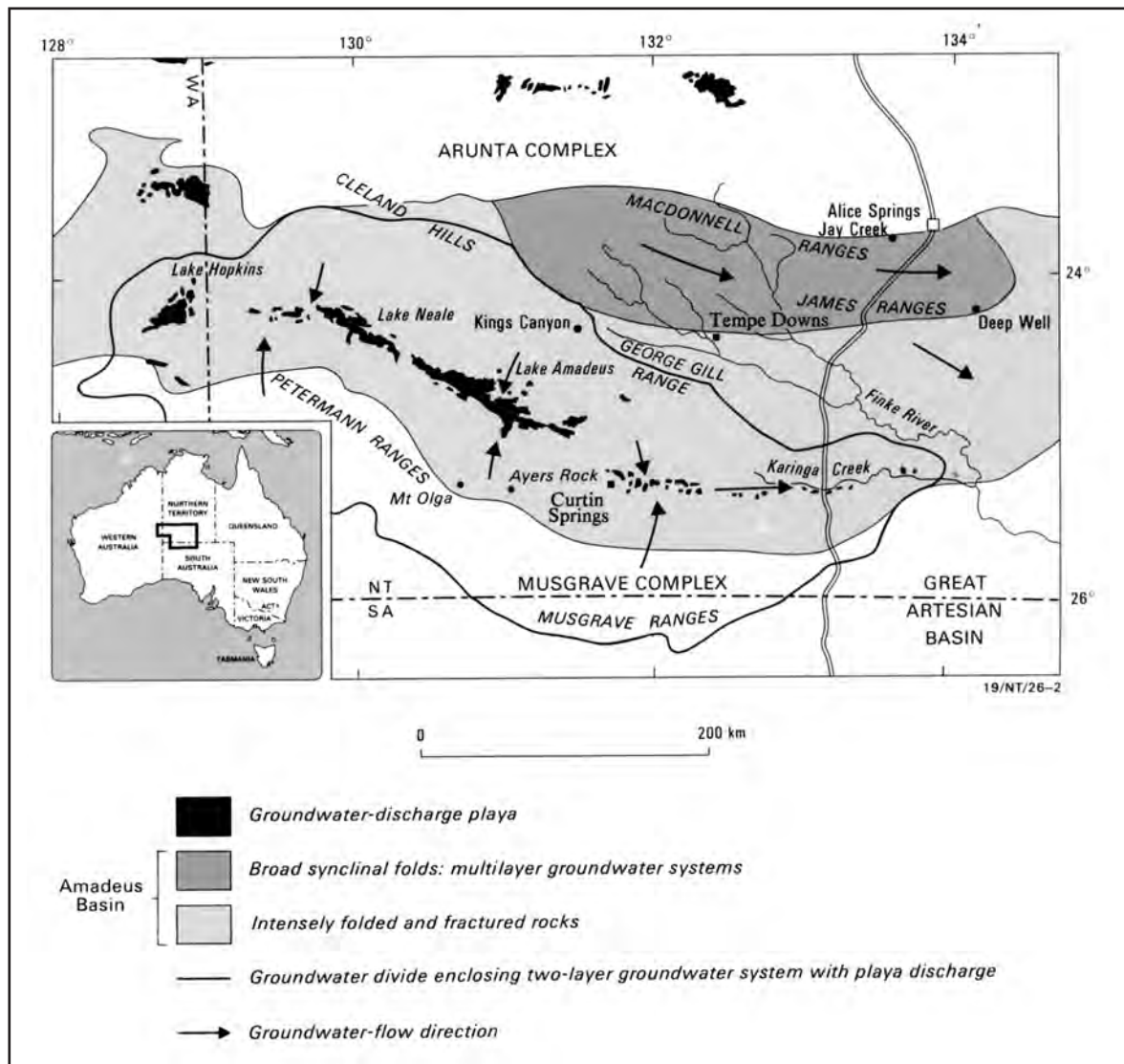
Figure 5.6.5 The Amadeus Basin, in central Australia,
