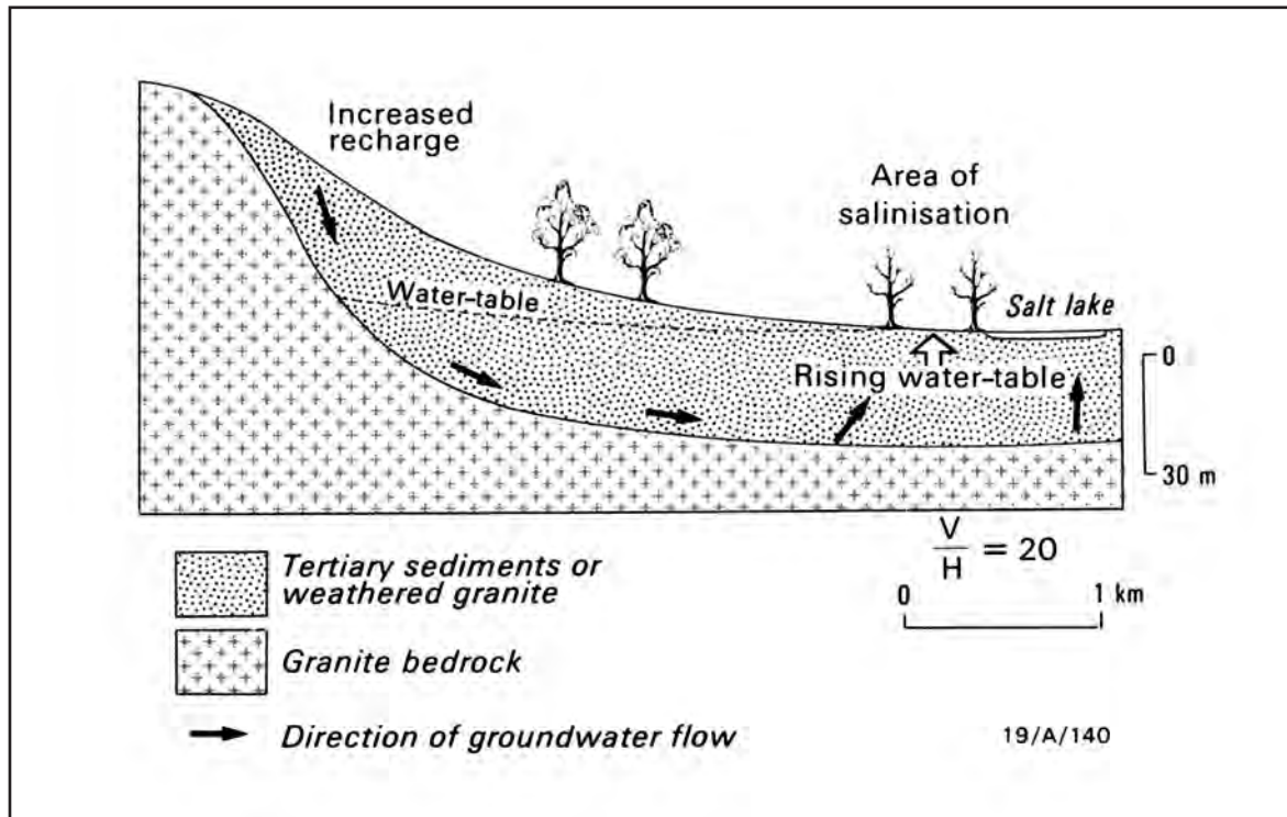
Figure 5.6.12 Native vegetation for agriculture leading to rising water tables over a timescale of several decades
