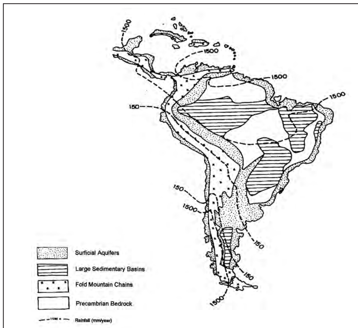
Figure 5.4.2.3 Major hydrogeological domains (Rebouças, 1991)
