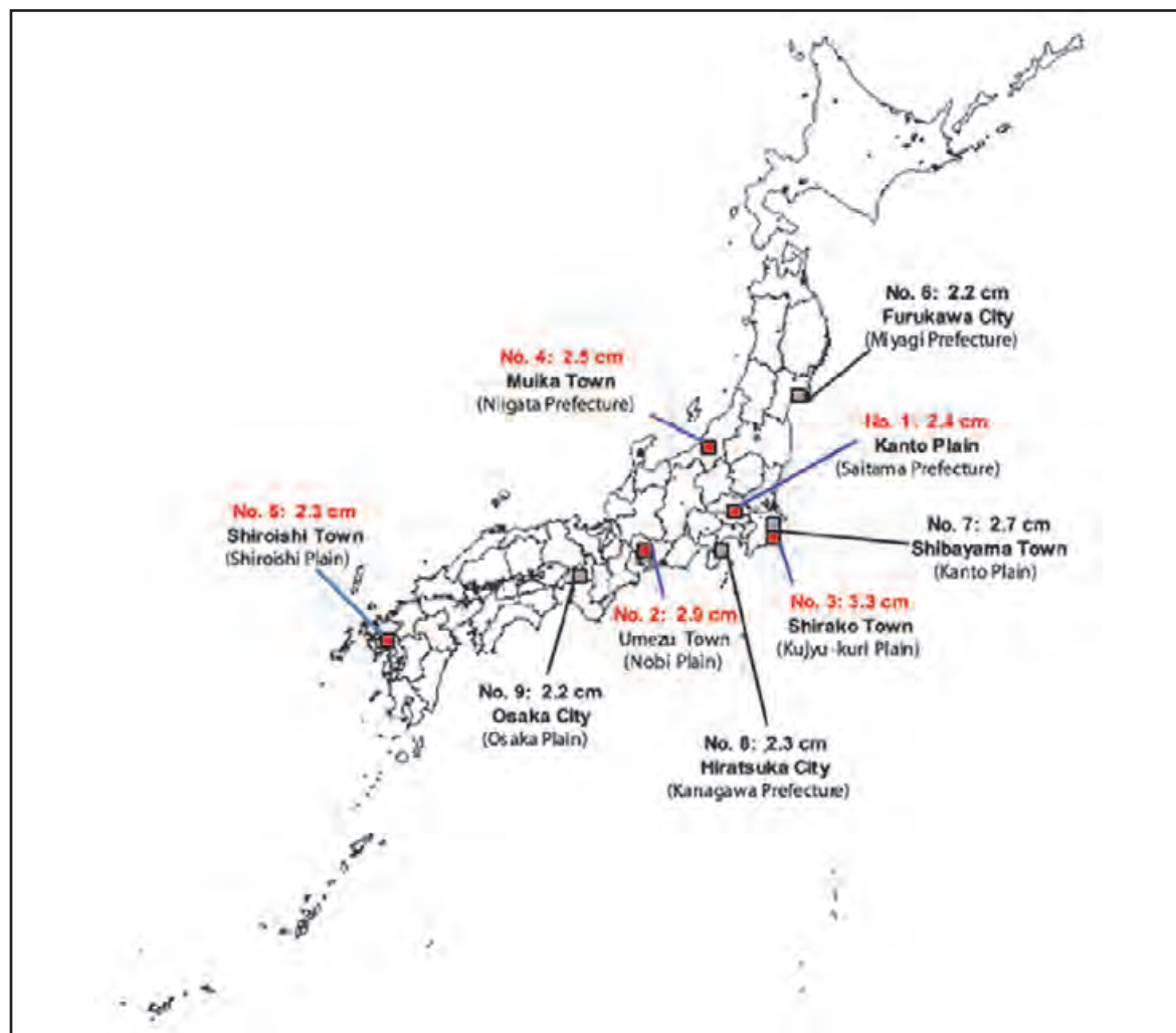
Figure 5.2.4.1.2.4 Location map of land subsidence over 2 cm. Each value in cm indicates the land subsidence in 1998
