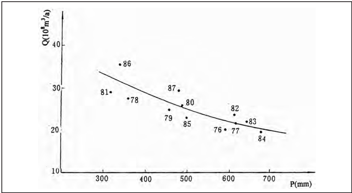
Figure 5.2.3.3.2.1 Correlation between annual precipitation (P) and extracted groundwater (Q) for farmland irrigation (Northern plain of Henan Province, 1976-87)
