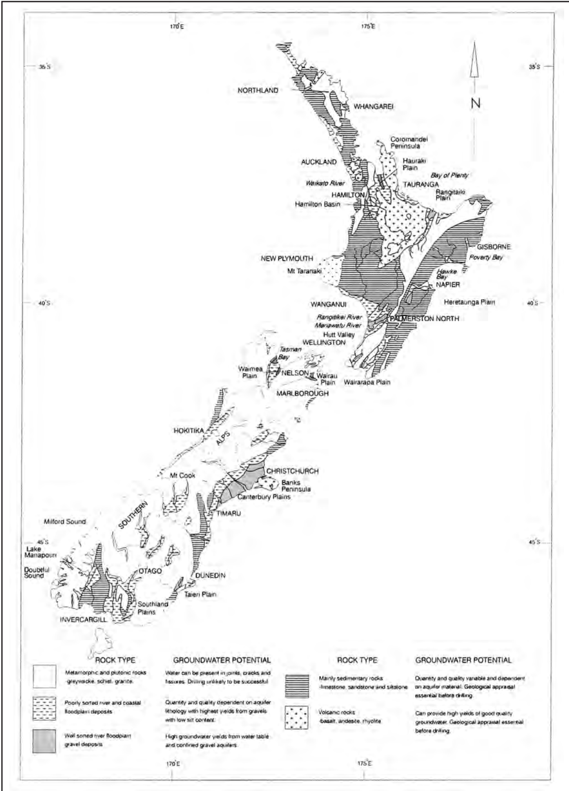
Figure 5.6.7.1 Distribution of regional hydrogeological units
