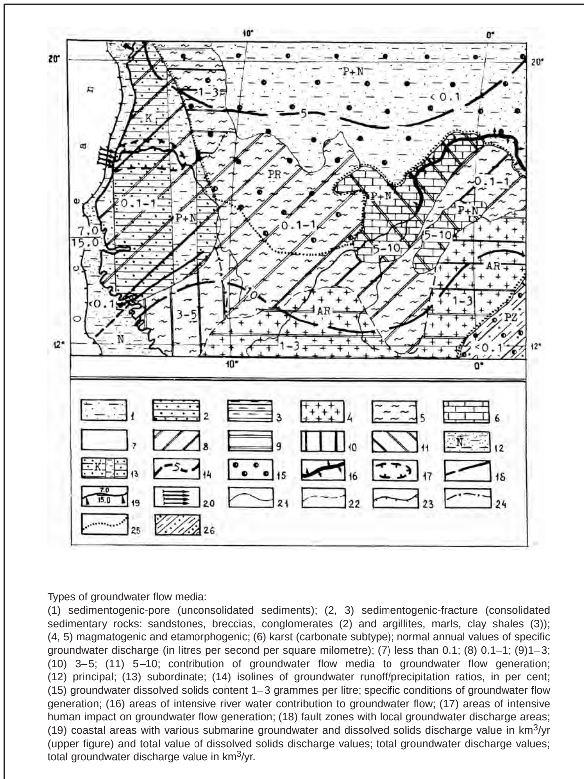
Figure 4.2.4.1 A model of the World Groundwater Flow Map on a 1:10 000 000 scale
