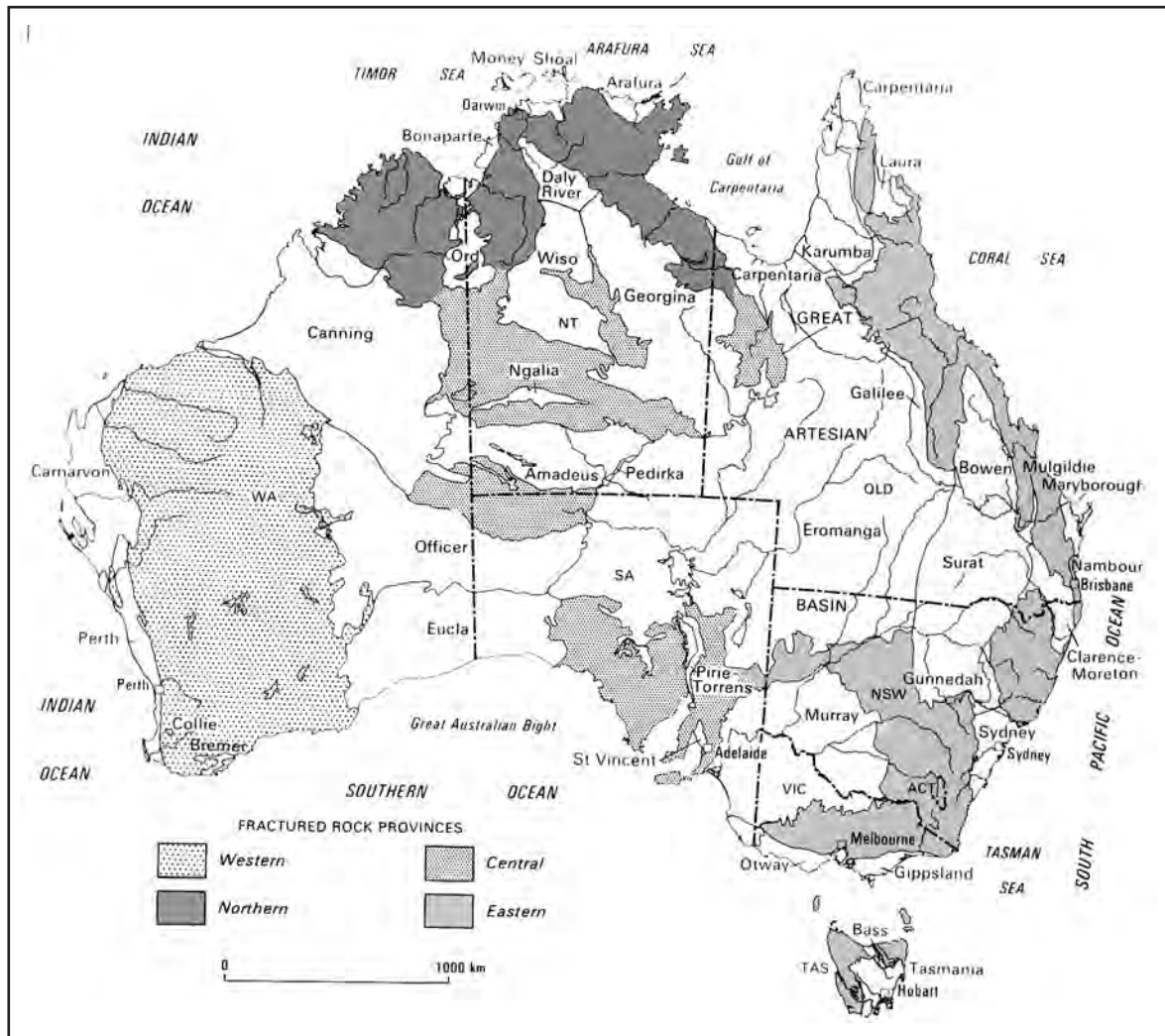
Figure 5.6.11 Four major fractured-rock groundwater provinces recognized in Australia
