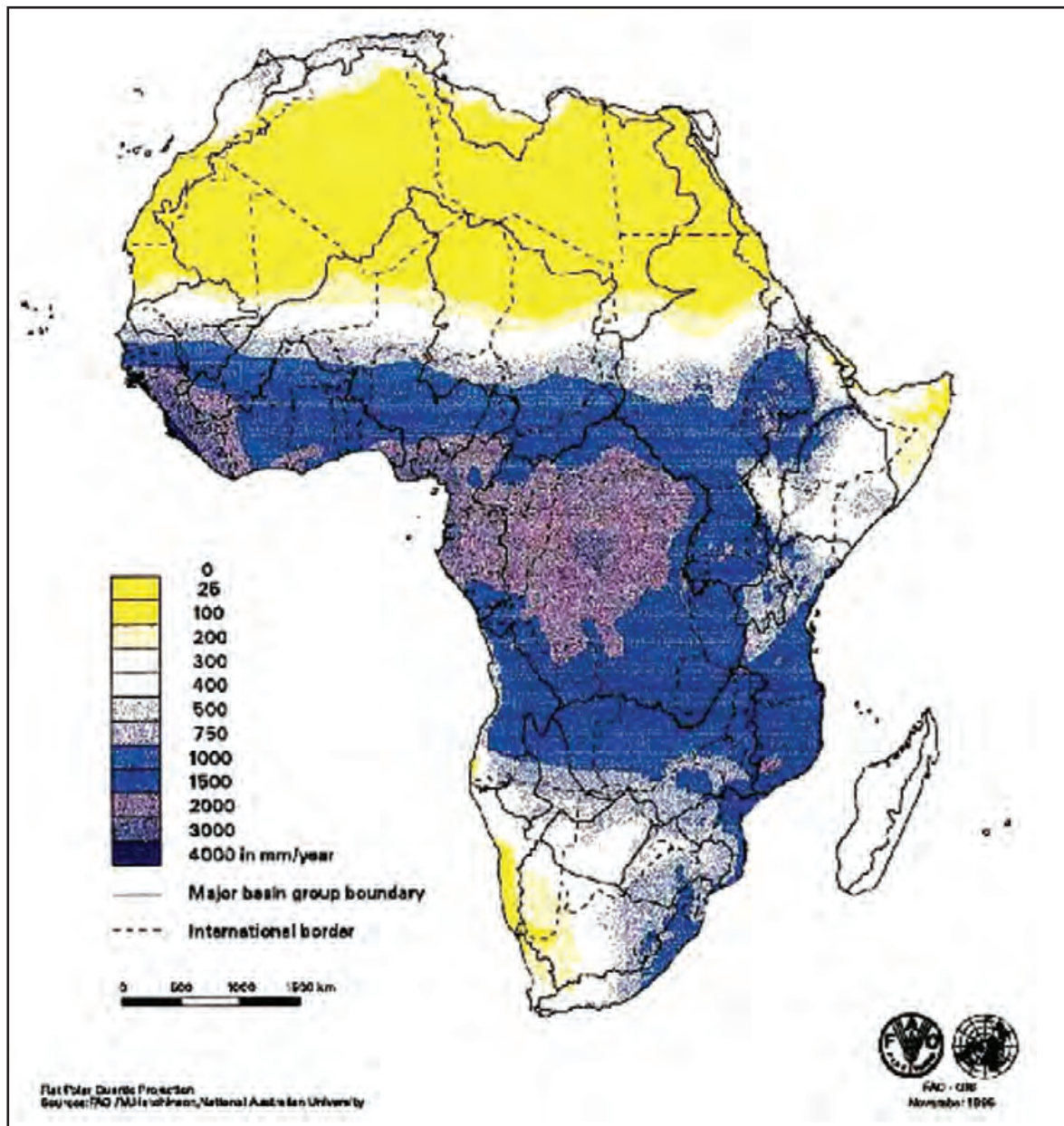
Figure 5.5.3.1 Average annual rainfall in Africa
