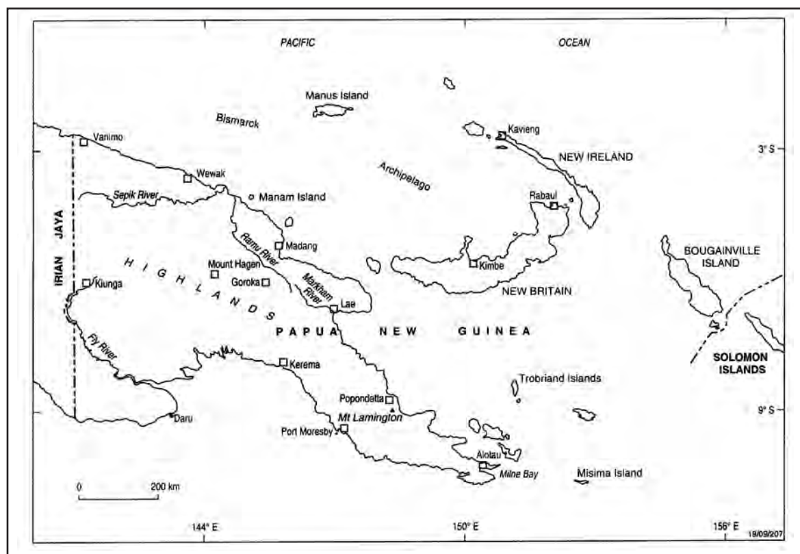
Figure 5.6.7.3 PNG's borders
