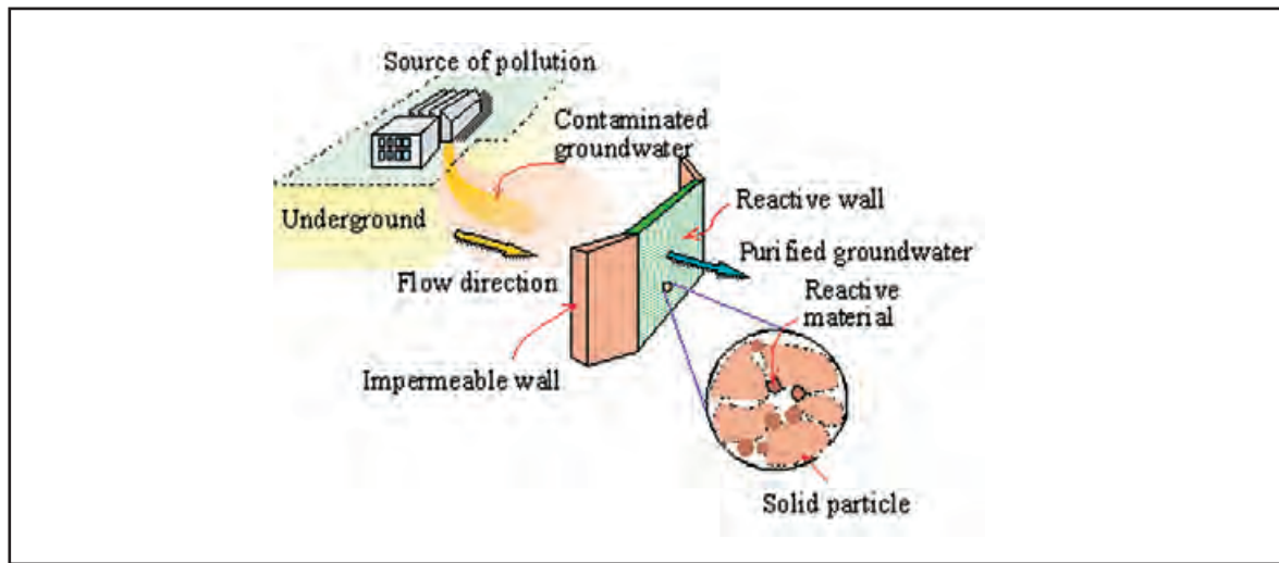
Figure 5.2.4.3.2.1 Reactive underground wall to treat contaminated groundwater (Original figure M. Shimomura et.al., English explanations are made by the author under the permission)
