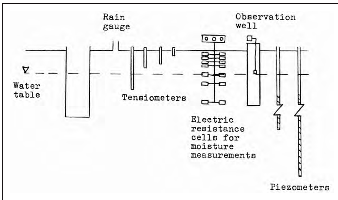
Fig 4.2.2.1 Diagram of a groundwater balance observation station (after W. Wundt in Keller, 1965)
