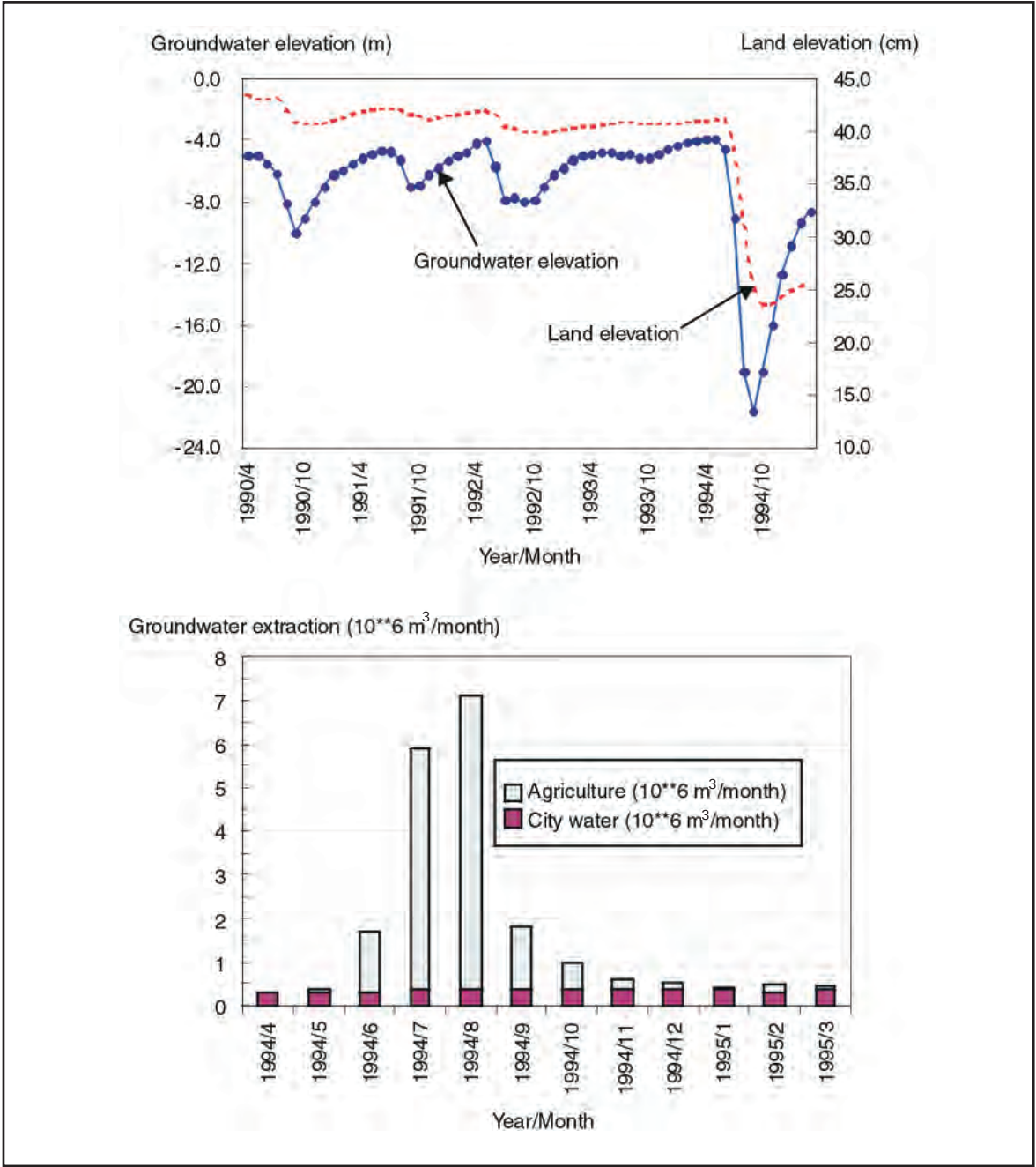
Figure 5.2.4.1.2.6 Land subsidence in Saga Prefecture, Kyushu, Japan and the variation of groundwater level, ground elevation and monthly groundwater exploitation
