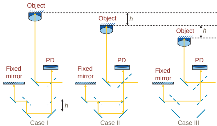
Figure 8 Three optical paths (cases I, II, and III) for interference.
