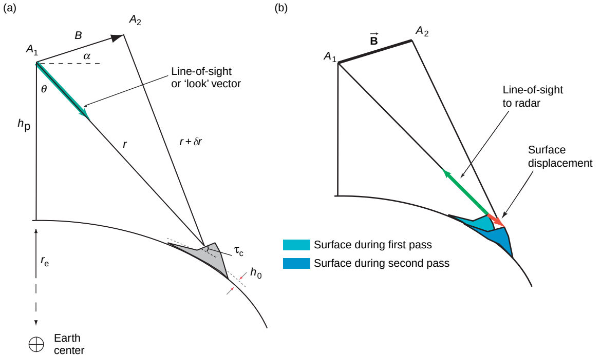
Figure 10 SAR interferometry imaging geometry in the plane normal to the flight direction for topography (a) and deformation (b) mapping.
