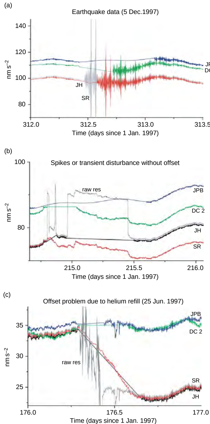
Figure 9 Examples of the data corrections done independently by different operators (identified by initials) for the removal/interpolation of (a) an earthquake, (b) disturbances without offsets, and (c) an offset caused by a helium refill. From Hinderer J, Rosat S, Crossley D, Amalvict M, Boy J-P, and Gegout P (2002a) Influence of different processing methods on the retrieval of gravity signals from GGP data. Bulletin d'Informations des Marées Terrestres 123: 9278–9301.
