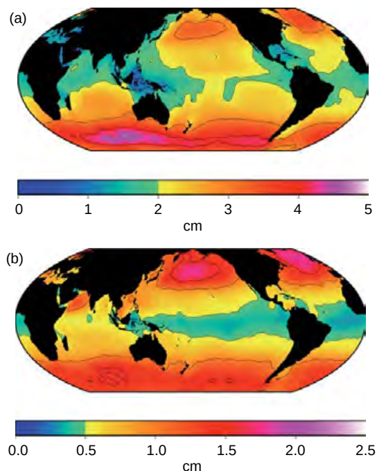
Figure 5 Estimates of possible errors in SSB. Mean error (a) is computed assuming error is 1% of mean SWH ( Chelton, 1994 ). The variable error (b) is computed assuming error is 1% of the RMS of SWH. Note that the scale of the variable portion is half the size of the mean portion.
