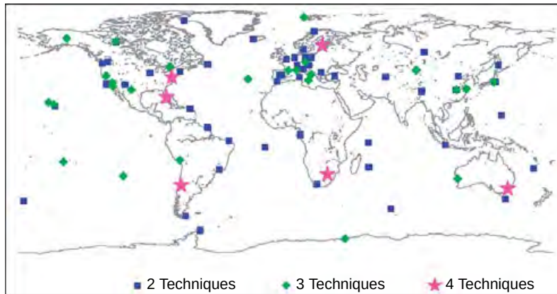
Figure 4 Distribution of co-located space geodetic stations that have at least two different operational techniques of GPS, VLBI, SLR, and DORIS. Courtesy of Z. Altamimi.
