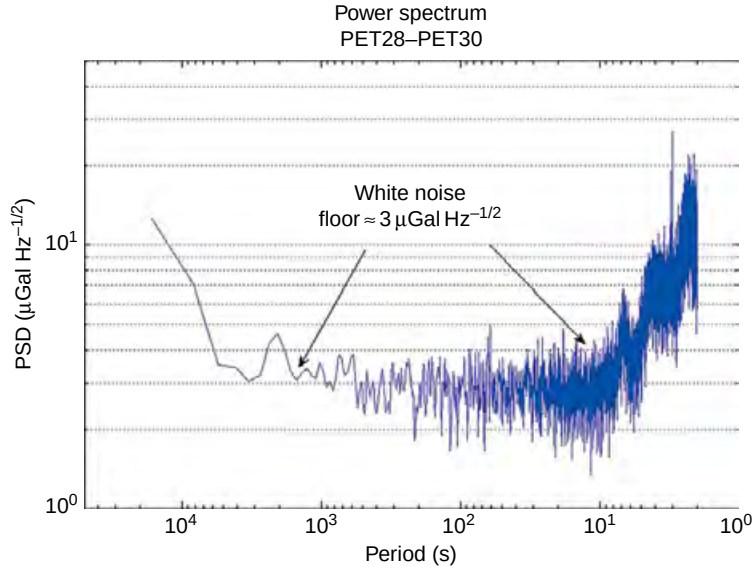
Figure 2 Difference between two PET gravity meters (1 day sampled at 1 Hz).
