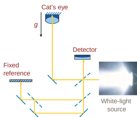
Figure 7 Schematic diagram of the Faller-Dicke absolute gravity meter (Princeton, 1963).
