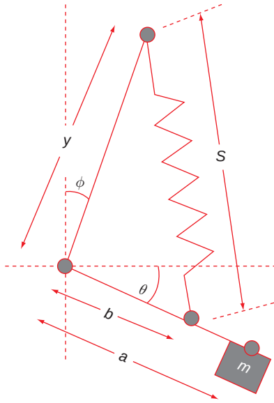
Figure 16 Tilted L&R suspension.
