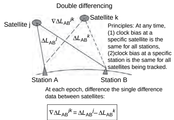
Figure 6 Diagram illustrating double differencing of GPS data. The idea is to difference away the satellite and station clock biases. Double differencing is equivalent to estimating the clock biases explicitly when processing undifferenced data.
