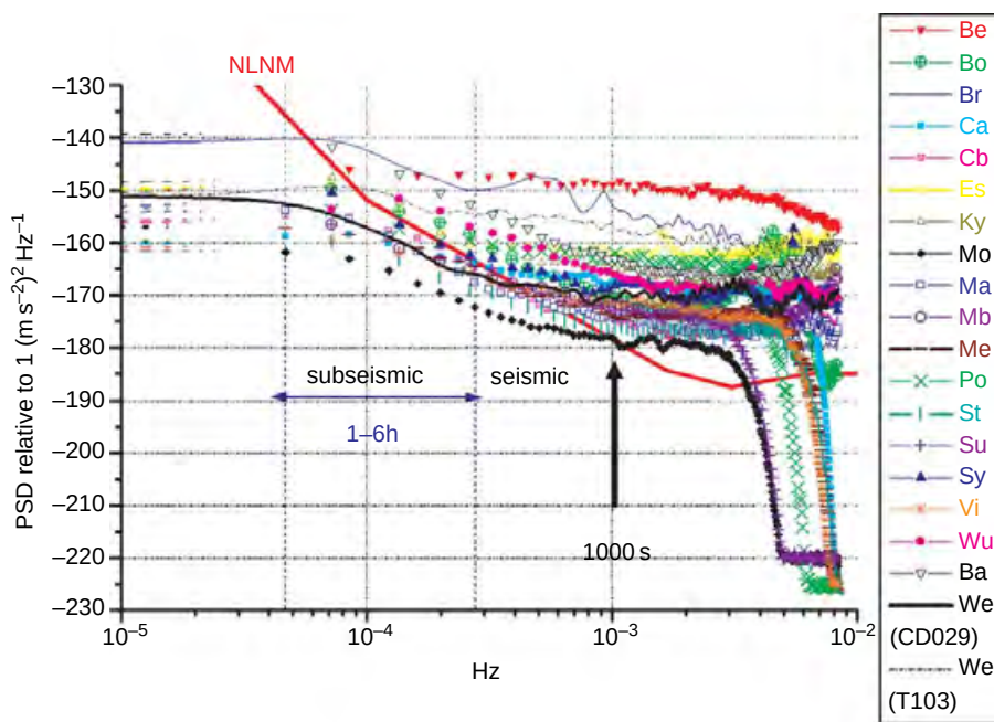
Figure 17 Noise levels of the SGs from the GGP network. Reproduced from Rosat S, Hinderer J, Crossley D, and Rivera L (2003a) The search for the Slichter Mode: Comparison of noise levels of superconducting gravimeters and investigation of a stacking method. Physics of the Earth and Planetary Interiors 140: 183–202, with permission from Elsevier.
