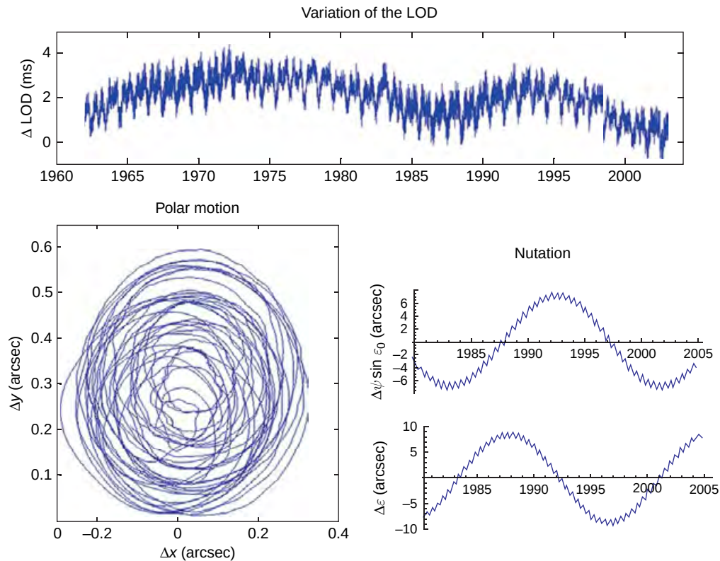
Figure 4 Observations of LOD variations, polar motion, and nutation.
