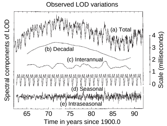
Figure 2 (a) Observed LOD variations during 1962–91 from the COMB91 combined optical astrometric and space-geodetic Earth orientation series and its decomposition into variations on (b) decadal, (c) interannual, (d) seasonal, and (e) intraseasonal timescales. Tidal variations are not shown. From Dickey JO, Marcus SL, Hide R, Eubanks TM, and Boggs DH (1994b) Angular momentum exchange among the solid Earth, atmosphere and oceans: A case study of the 1982–83. El Niño event. Journal of Geophysical Research 99(B12): 23921–23937.
