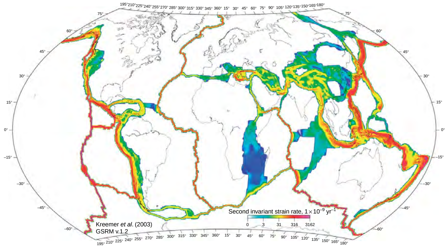
Figure 10 A global strain-rate map, derived from space geodetic data. From Kreemer C, Holt WE, Haines AJ (2003) An integrated global model of present-day plate motions and plate boundary deformation. Geophysical Journal International 154: 8-34.
