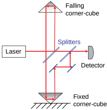
Figure 10 FG5 Mach-Zender interferometer for measuring gravity.
