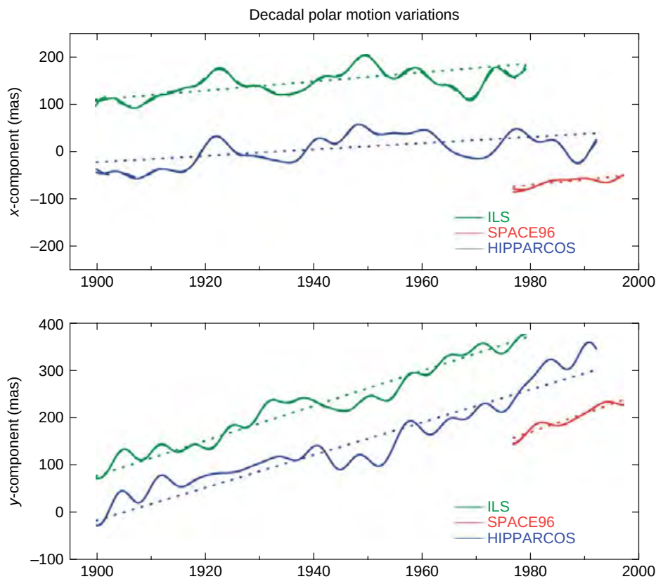
Figure 7 Observed decadal-scale polar motion variations from the ILS optical astrometric series (solid green curve), the HIPPARCOS optical astrometric series (solid blue curve), and the SPACE96 combined space-geodetic series (solid red curve). The decadal-scale variations were obtained by applying to the original series a low-pass boxcar filter having a 6-year cutoff period. The dotted lines show the linear trends in the pole path that were estimated from these series by Gross and Vondrák (1999). The dashed lines that coincide with the solid lines and that are therefore hidden from view show the model of the decadal variations that they used when estimating the trend. For clarity of display the curves have been offset from each other by an arbitrary amount. From Gross RS and Vondrák J (1999) Astrometric and space-geodetic observations of polar wander . Geophysical Research Letters 26(14): 2085–2088.
