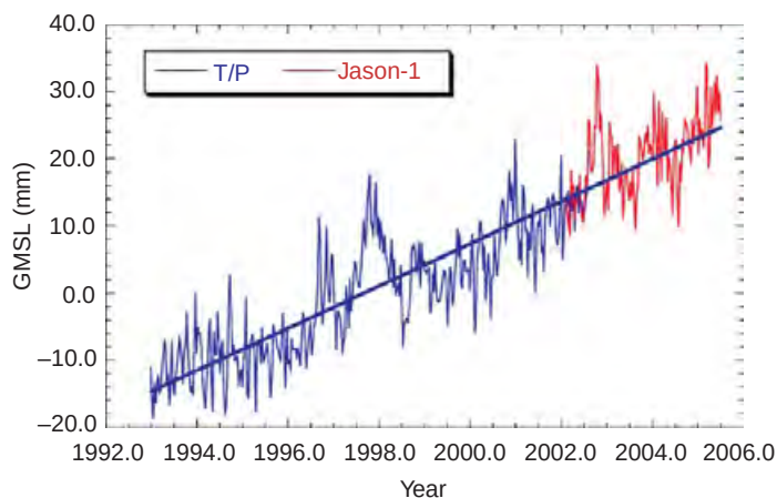
Figure 16 GMSL from corrected T/P (blue) and Jason-1 (red) data from Jan. 1993 to Jun. 2005 at 10-day intervals. The T/P data have been corrected for the oscillator error (Section 3.05.4.2), the drift in TMR (Section 3.05.2.3), and the different TOPEX_A and TOPEX_B SSB models (Section 3.05.2.4), while the Jason-1 data have had a relative bias applied (Section 3.05.4.1) and have been corrected for the biases in the JMR wet path delays (Section 3.05.2.3). The long-term linear trend is shown with a thick blue line.
