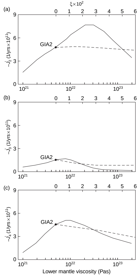
Figure 7 Solid lines – predictions of (a) \dot{J}_2 , (b) \dot{J}_3 , and (c) \dot{J}_4 due to GIA as a function of the lower-mantle viscosity (bottom abscissa scale) of the Earth model (reproduced from Figure 2). The dot labeled GIA2 is the prediction obtained with a lower-mantle viscosity of 5 \times 10^{21} Pa s. The dashed line on each frame indicates the perturbation in the prediction GIA2 associated with increasing levels of lateral heterogeneity in the lower-mantle viscosity field, as reflected by the parameter \epsilon (top abscissa scale; see text and eqn [3]). All calculations adopt an elastic lithospheric thickness of 100 km, and an upper-mantle viscosity of 5 \times 10^{20} Pa s.
