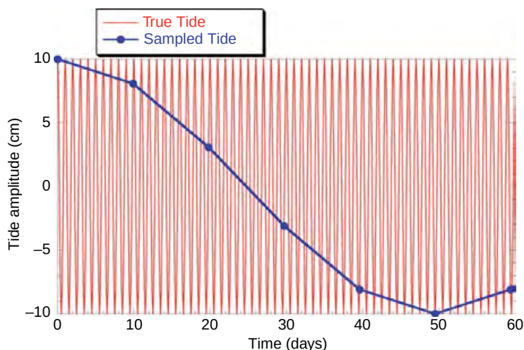
Figure 9 Aliasing of a 1 cycle-per-day signal (red) by sampling every 9.9 days (blue).
