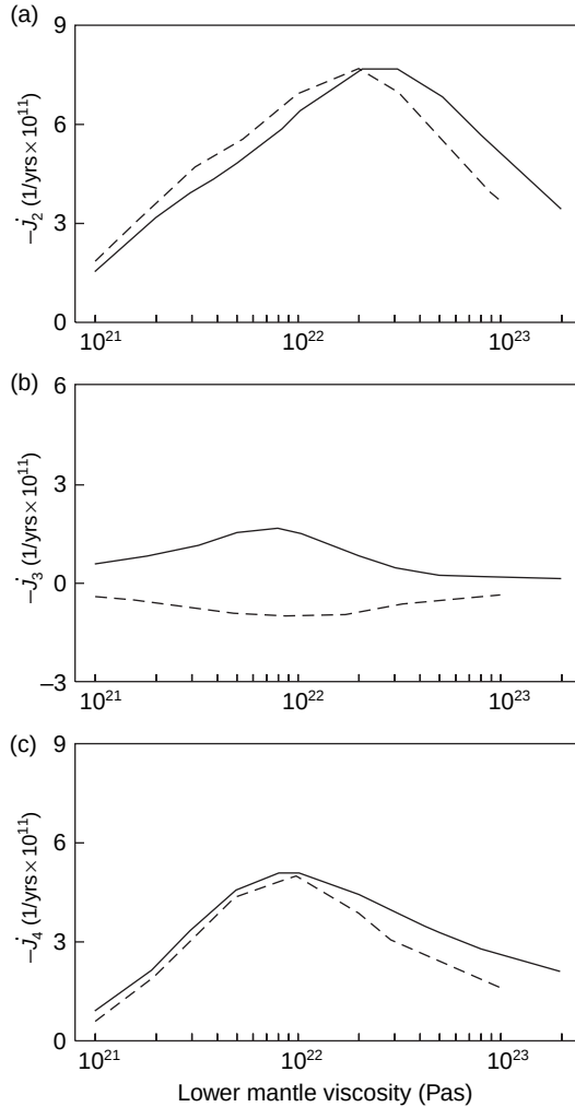
Figure 2 Solid lines – predictions of (a) \dot{J}_2 , (b) \dot{J}_3 , and (c) \dot{J}_4 due to GIA as a function of the lower-mantle viscosity (bottom abscissa scale) of the Earth model. As in Figure 1 , the predictions use a global Late Pleistocene ice history based on the ICE-3G model (Tushingham and Peltier, 1991). The dashed line on each frame is the analogous prediction based on the disk load ice model discussed in the text.
