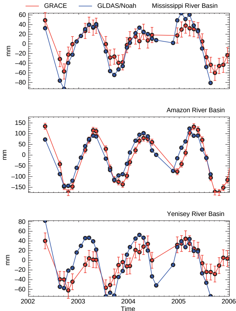
Figure 9 Water-storage results for three river basins, obtained using specially constructed averaging kernels for those basins. GRACE results, with their 68.3% confidence limits, are shown in red (postprocessed to reduce noise, as described by Swenson and Wahr (2006a)). Results from the GLDAS/Noah land surface model (Rodell, et al. , 2004a) are in blue. Figure provided by Sean Swenson.
