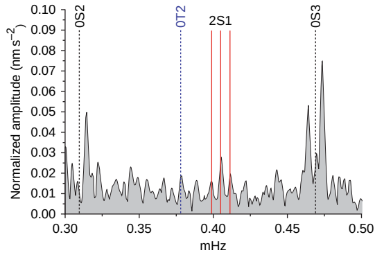
Figure 18 Normalized amplitude spectrum (in \text{nm s}^{-2} ) in the frequency band 0.3–0.5 mHz after the M_w=8.4 Peru event exhibiting the triplet of the {}_2S_1 mode. Reproduced from Rosat S, Rogister Y, Crossley D, and Hinderer J (2006) A search for the Slichter triplet with superconducting gravimeters: Impact on the density jump at the inner core boundary. Journal of Geodynamics 41: 296–306, with permission from Elsevier.
