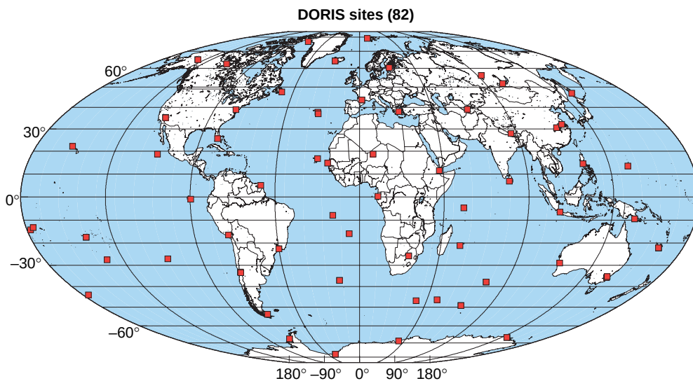
Figure 4 Locations of the 82 DORIS sites that are included in the ITRF2005 reference frame. These sites have active communication between the ground stations and the satellites that are tracked with DORIS.
