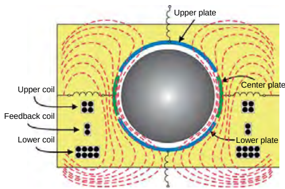
Figure 4 Schematic diagram of the Nb sphere, coils, plates, and general pattern of magnetic flux lines. Flux is excluded from the sphere and is confined externally by the Nb shield.
