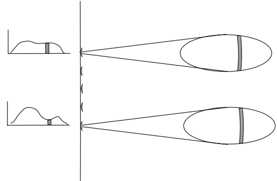
Figure 28 Radar imaging as viewed looking down at the Earth from above the sensor. The sweep of the pulse across the radar beam leads to a return echo trace for each pulse as depicted on the left. Every IPP, a pulse is sent and a trace recorded. The collection of pulses, that is, the along-track history of range profiles, is therefore a 2-D representation of the surface, albeit poorly resolved. There is considerable redundant information for any given surface element in the pulses because the beam samples each point many times as it travels along track (e.g., pulses every 5 m observed over a beam extent of 5 km). Through matched filtering techniques, a fine resolution image of the surface can be generated.
