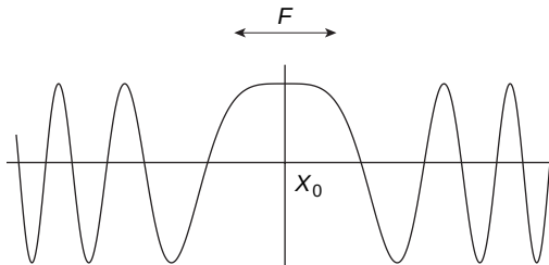
Figure 32 Illustration of the Fresnel zone, where the phase from an incident wave front varies by less than \pi/4 radians across the zone (right). Symmetric chirp at left is the real part of the azimuth chirped phasor. It is nearly constant over the Fresnel zone. The synthetic array is coherent over this length and points simply summed in azimuth will add coherently, and will be resolved at this length.
