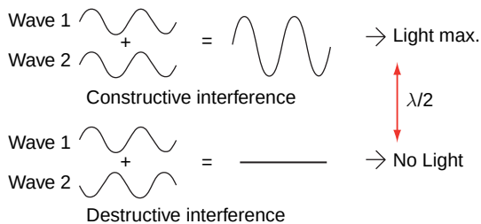
Figure 11 Two-beam interference with coherent light.
