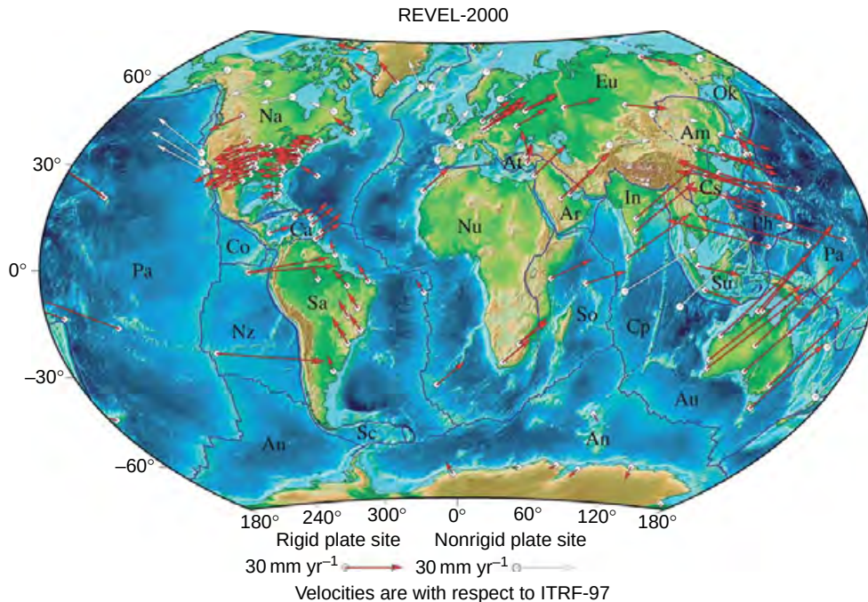
Figure 9 The REVEL-2000 plate motion model derived from GPS velocities. From Sella G, Dixon T, and Mao A (2002) REVEL : A model for recent plate velocities from space geodesy. Journal of Geophysical Research 107(B4) (doi:10.1029/2000JB000033).
