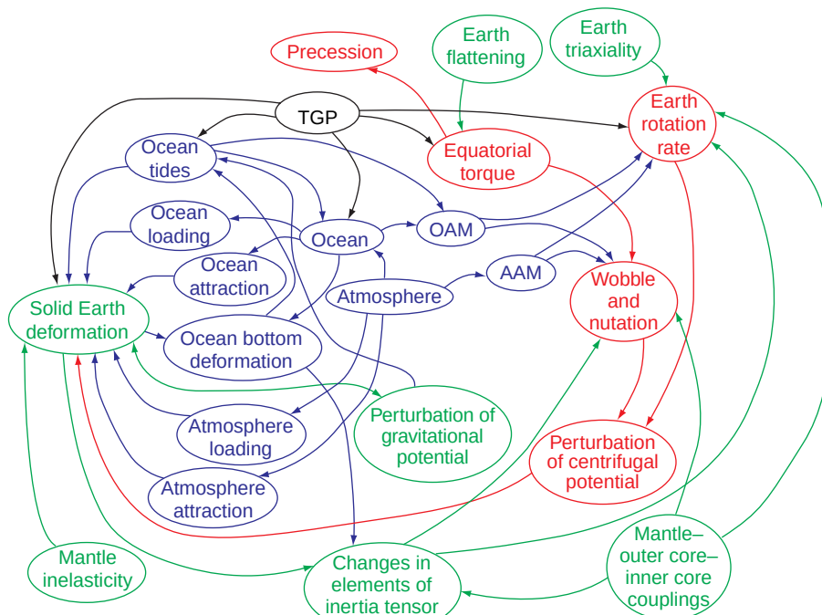
Figure 5 Chart representing all the interactions and physical processes involved in Earth orientation variations and in Earth deformations.
