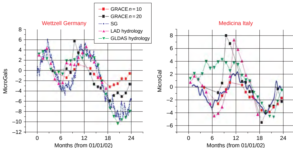
Figure 32 An example of the superposition of gravity changes seen by GRACE (in red for n=10 and in black for n=20 ) and the superconducting gravimeter in Wettzell (Germany) and Medicina (Italy) (in blue) and contributions from continental hydrology models like GLDAS (in green) and LADWorld (in purple).
