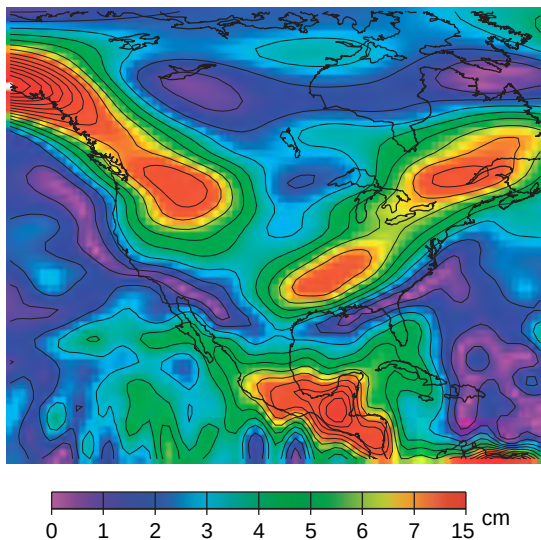
Figure 8 The amplitude of the annually varying mass signal, in units of centimeters of water thickness, recovered from GRACE during spring 2002 through spring 2006. The results have been postprocessed to reduce noise (Swenson and Wahr, 2006a), and smoothed with a 300-km Gaussian. The solid lines represent contour intervals of 1 cm.
