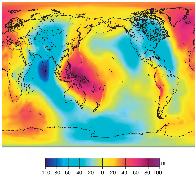
Figure 1 The time-averaged geoid anomaly from EGM96 ( Lemoine et al. , 1998 ).
