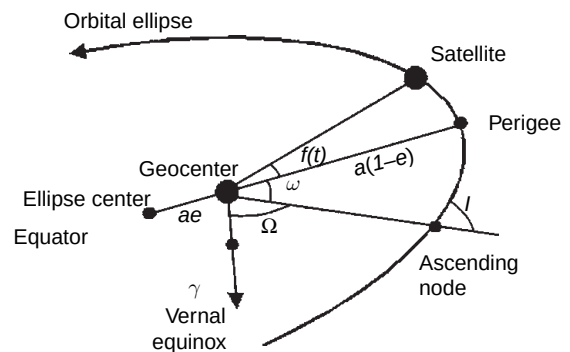
Figure 5 Diagram illustrating the Keplerian orbital elements: semimajor axis a , eccentricity e , inclination l , argument of perigee (closest approach) \omega , Right Ascension of the ascending node \Omega , and true anomaly f as a function of time t . The geocenter is the Earth center of mass; hence, satellite geodesy can realize the physical origin of the terrestrial reference system. This diagram is exaggerated, as GPS orbits are almost circular.
