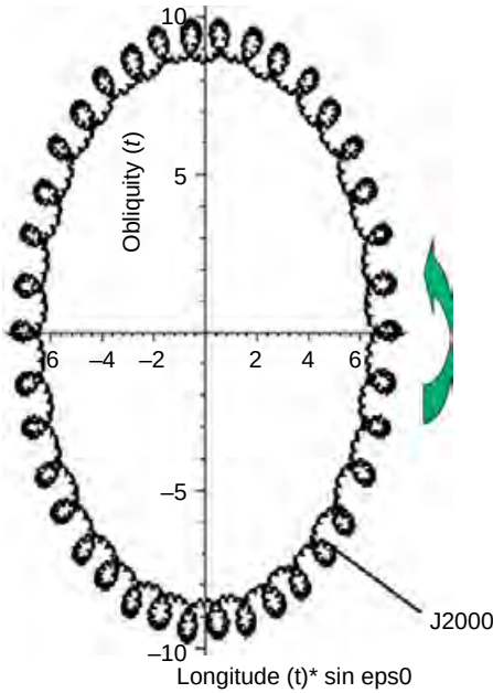
Figure 7 Representation of the changes in the position of the axis undergoing nutations alone.
