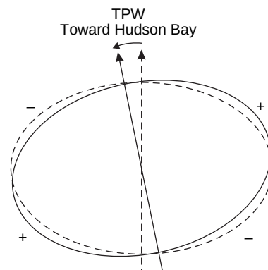
Figure 3 Schematic illustration of the geometry of the GIA-induced rotational feedback signal. The initial rotation pole and associated centrifugal potential are given by the dashed lines. A shift in the rotation pole counter-clockwise (or, as labeled on the figure, toward Hudson Bay – as expected in consequence of GIA), leads to a new orientation for both the pole and the centrifugal potential (solid lines). The so-called rotational driving potential is given by the difference between the centrifugal potential in the two states (solid minus dashed). The direct gravitational effect and deformation driven by this perturbation in the potential will act to bring the geoid (or sea surface) down in the quadrants labeled with '–' and up in quadrants labeled with '+'.
