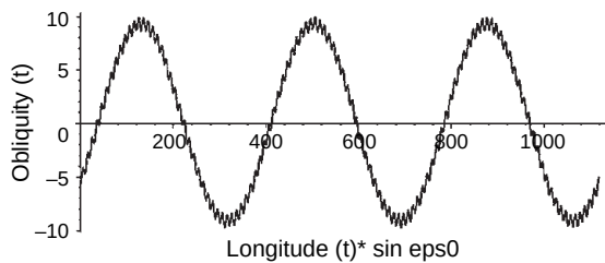
Figure 3 Representation of the changes in obliquity of the axis undergoing nutations.
