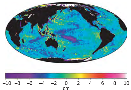
Figure 14 Difference between GSFCMSS00 (Wang, 2000) and CSRMS98 (Tapley and Kim, 2001), averaged in 0.25^\circ grids.
