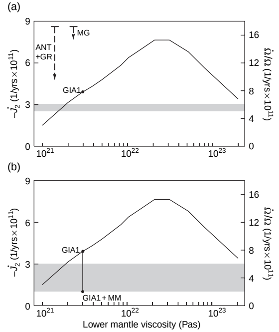
Figure 1 (a) Predictions of \dot{J}_2 due to GIA as a function of the lower-mantle viscosity of the Earth model (abscissa). The right ordinate scale refers to the normalized rate of change of the rotation rate, \dot{\Omega}/\Omega . The shaded region represents the observational constraint on \dot{J}_2 derived from satellite data by Nerem and Klosko (1996). The arrows at top left indicate the \dot{J}_2 signal associated with a net twentieth-century melting from the Antarctic and Greenland ice complexes of 1 \text{ mm yr}^{-1} equivalent eustatic sea-level rise (ANT + GR) and the melting of small ice sheets and mountain glaciers tabulated by Meier (1984) (MG; \text{ESL} = 0.4 \text{ mm yr}^{-1} ). The result labeled GIA1 is the \dot{J}_2 prediction obtained with a lower-mantle viscosity of 3 \times 10^{21} \text{ Pa s} . (b) As in frame (a), except the observational constraint is based on a new analysis of uncertainties associated with the 18.6-year tide (see text). The prediction labeled GIA1 + MM is the total signal associated with the model GIA1 and a twentieth-century melt history composed of Meier's (1984) sources plus 0.6 \text{ mm yr}^{-1} of ESL rise from polar ice sheets (total \text{ESL} = 1 \text{ mm yr}^{-1} ). All GIA calculations adopt an elastic lithospheric thickness of 100 km, and an upper-mantle viscosity of 5 \times 10^{20} \text{ Pa s} .
