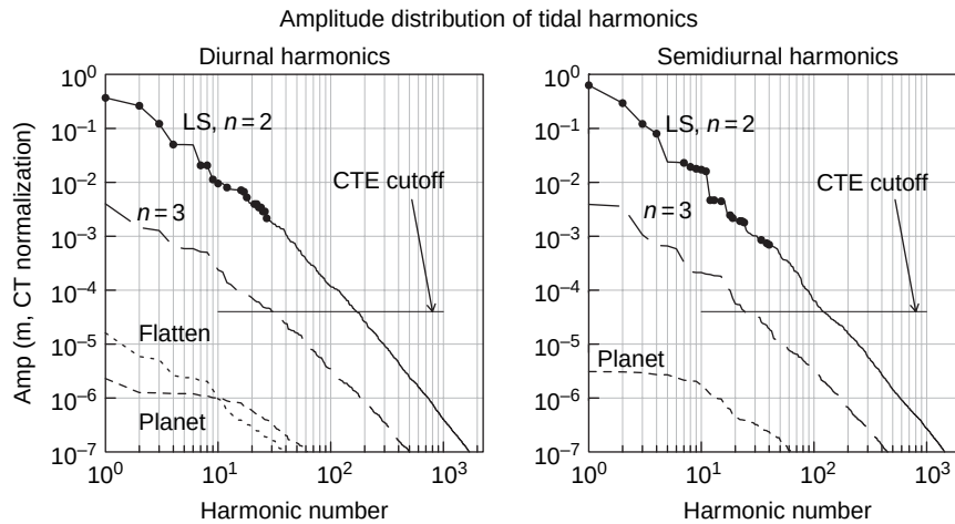
Figure 4 Distribution of harmonic amplitudes for the catalog of Hartmann and Wenzel (1995) , normalized according to Cartwright and Taylor (1971) . The line ‘LS, n=2 ’ refers to lunisolar harmonics of degree 2; those with large dots have Darwin symbols associated with them. Constituents of degree 3, from other planets, and from earth flattening are shown as separate distributions. The horizontal line shows the approximate cutoff level of the Cartwright and Taylor (1971) list.
