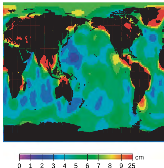
Figure 12 The rms about the mean of ocean surface mass variability deduced from GRACE for spring 2002 through spring 2006, smoothed with a 750-km Gaussian.
