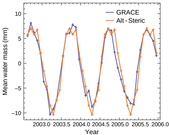
Figure 13 Compares seasonal estimates of total ocean mass from GRACE, with estimates deduced from a combination of satellite altimetry and in situ temperature and salinity measurements. Results provided by Don Chambers.
