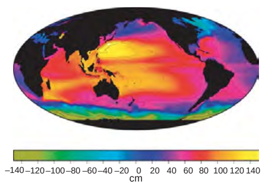
Figure 12 Global DOT from GSFCMSS00 (Wang, 2000) – GGM02C (Tapley et al. , 2005), filtered to suppress variations with wavelengths smaller than 444 km (e.g., Tapley et al. , 2003).
