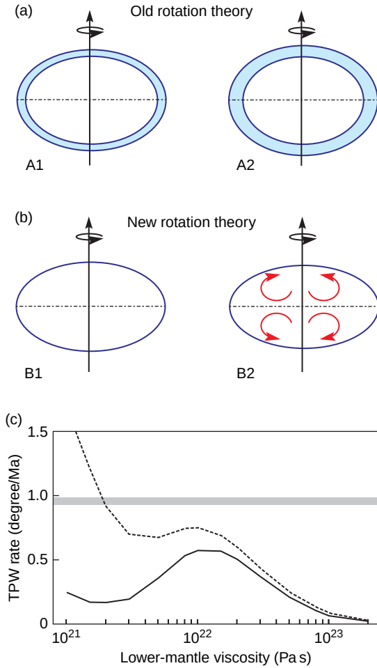
Figure 5 Schematic illustration of the difference in the underlying choice for the background oblateness of the Earth made within the (a) traditional (e.g., Wu and Peltier, 1984) and (b) new (Mitrovica et al. , 2005) GIA rotation theories (see text). (c) Predicted present-day true polar wander rate due to GIA as a function of the lower mantle viscosity of the Earth model. The dotted and solid lines are generated using the traditional and new rotation theories, respectively. All calculations adopt an elastic lithospheric thickness of 100 km, and an upper-mantle viscosity of 10^{21} Pa s. The shaded region represents an observational constraint on the TPW rate from Gross and Vondrak (1999).
