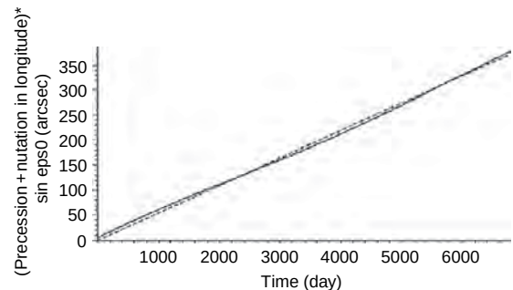
Figure 2 Representation of the changes in longitude of the axis undergoing precession and nutations.
