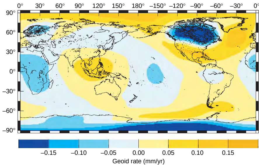
Figure 8 Perturbation in the prediction of the present-day rate of change of the geoid height due to GIA associated with the introduction of lateral variations in mantle viscosity within the lower mantle defined by \epsilon = 0.055 (as in Figure 6); that is, the prediction for the 3-D model minus the prediction based on the spherically symmetric model GIA2 (in each case, rotational feedback is not included).
