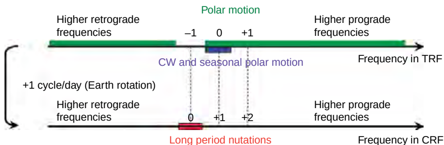
Figure 6 Definition of polar motion frequencies and precession-nutation frequency.
