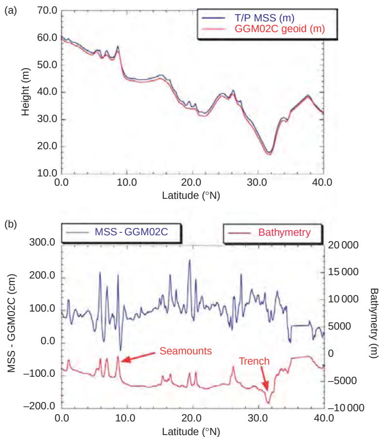
Figure 11 (a) Average SSH along a T/P pass in the western Pacific (blue), along with the GGM02C geoid (red) (Tapley et al. , 2005). (b) The difference (blue) shows the long-wavelength dynamic topography and higher-resolution geoid that is not modeled. The corresponding bathymetry is shown in red.
