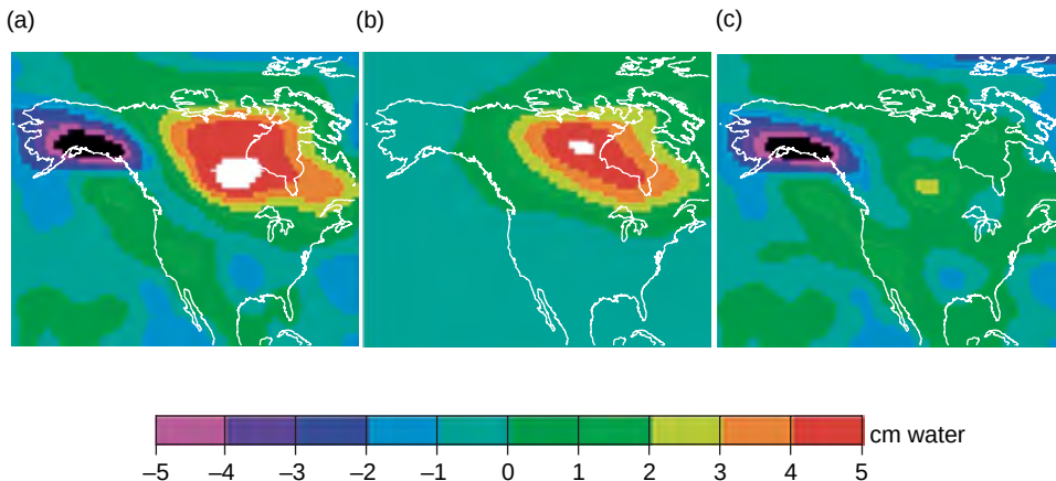
Figure 11 (a) The best-fitting linear trend for the GRACE fields between spring 2002 and spring 2004, after postprocessing the fields as described by Swenson and Wahr (2006a). Results have been smoothed with a 400-km Gaussian smoothing function. Units are in \text{cm yr}^{-1} of water thickness. (b) Predictions based on the ICE-5G PGR ice deglaciation model (Peltier, 2004). (c) The difference between (a) and (b).
