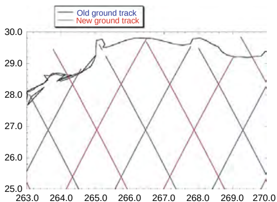
Figure 15 Ground tracks for original T/P (and current Jason-1) orbit (blue) and new T/P orbit (red) in the Gulf of Mexico.
