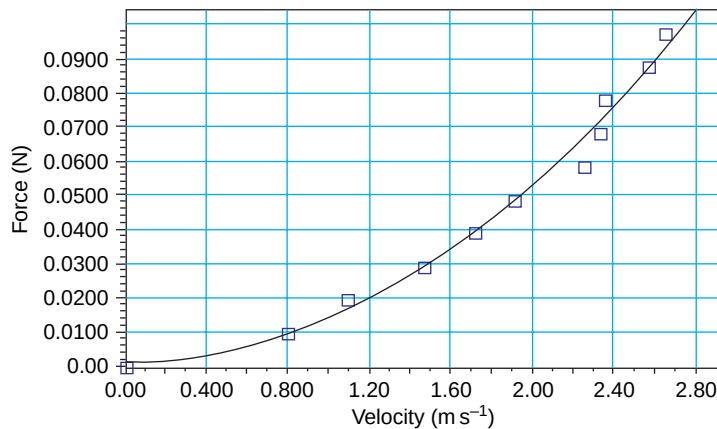
Figure 6 Air resistance vs velocity, from Hockaday.
