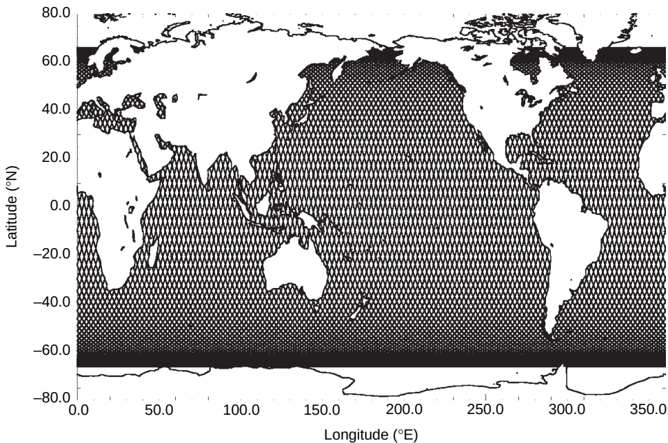
Figure 1 Ground track for TOPEX/Poseidon.
