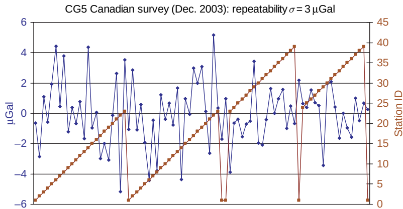
Figure 3 CG5 repeatability using data from a CG5 Survey in Northern Canada during December.
