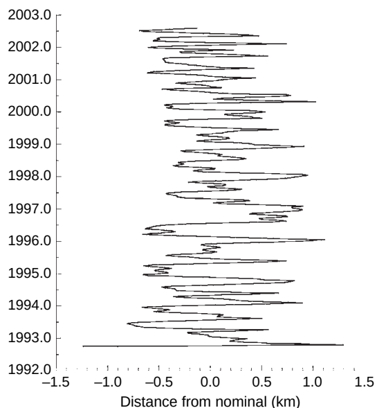
Figure 8 Plot of T/P ground track variation around nominal ground track at equator for duration of primary mission until it was moved to its current ground track. Positive excursions indicate the position is east of nominal, while negative values indicate the position is west of nominal.
