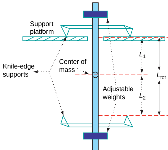
Figure 5 Schematic diagram of the Kater pendulum.
