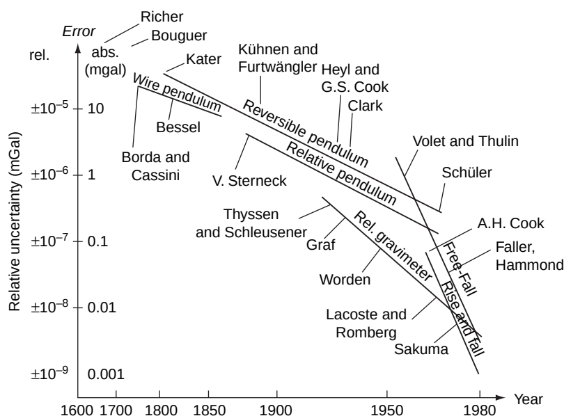
Figure 4 Accuracy of gravity meters, from Torge.
