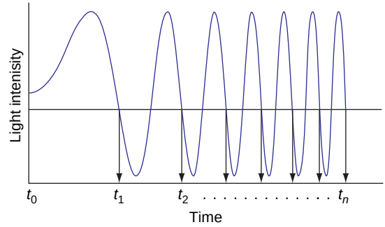
Figure 12 Two-beam interferometer signal for gravimeter with zero-crossings.
