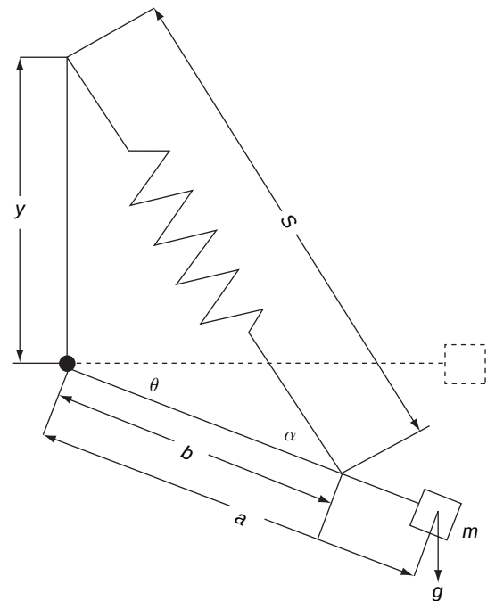
Figure 15 LaCoste and Romberg spring gravity meter suspension.
