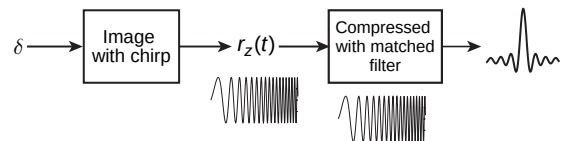
Figure 26 Illustration of the matched filter for the delta-function scene and linear FM chirp. The compressed signal is close to a sinc function.
