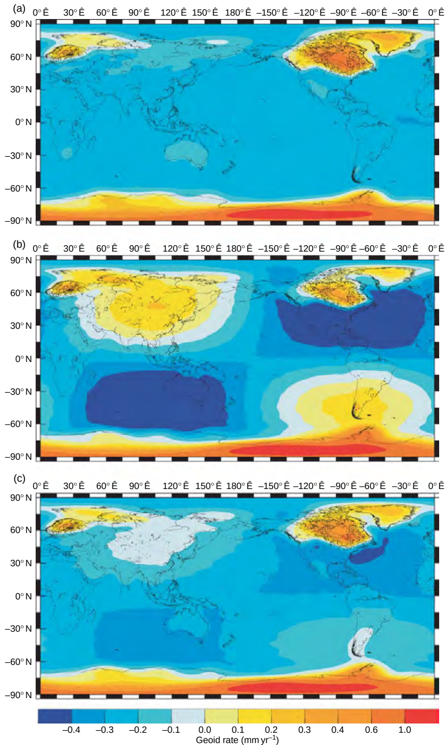
Figure 4 Maps of the predicted present-day rate of change of geoid height due to GIA computed using an Earth model with a lithospheric thickness of 120 km, an upper-mantle viscosity of 10^{21} Pa s and a lower-mantle viscosity of 2 \times 10^{21} Pa s. The predictions are distinguished on the basis of the treatment of the rotational feedback due to TPW: (a) no feedback (i.e., a nonrotating Earth model); (b) feedback computed using the traditional GIA rotation theory (e.g., Wu and Peltier, 1984); and (c) feedback computed using the new GIA rotation theory (Mitrovica et al. , 2005).
