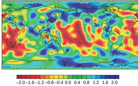
Figure 6 Map of the perturbation in the logarithm of viscosity relative to the mean value associated with model GIA2 ( 5 \times 10^{21} Pa s) at depth of 2000 km in the mantle. The field was generated by adopting \epsilon = 0.055 in eqn [3] (see text for details).
