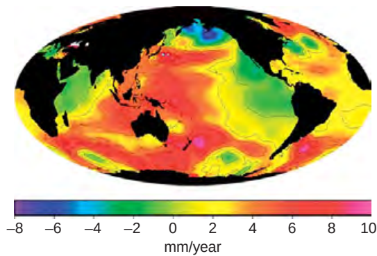
Figure 17 Map of local SL rates determined from T/P and Jason-1 data from Jan. 1993 to Dec. 2004. Data were mapped using a Gaussian with a 1000-km radius, before computing trends. All data were corrected as for Figure 16 .
