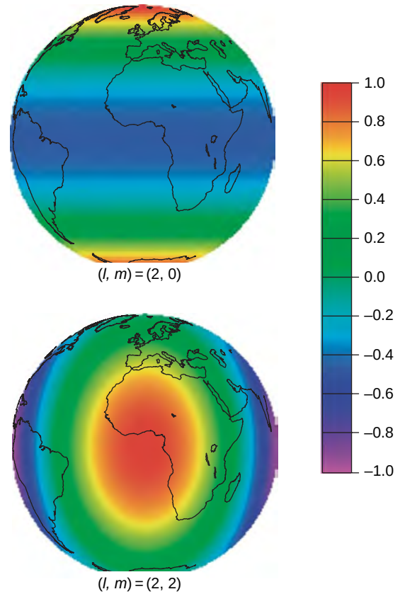
Figure 3 The spatial patterns of the Legendre functions \tilde{P}_{20} and \tilde{P}_{22} .
