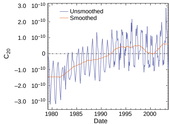
Figure 4 The blue line shows a time series of C_{20} , determined from more than 20 years of SLR measurements (data provided by Chris Cox, personal communication, 2005). The red line is a smoothed version of those values, obtained by first fitting and removing seasonal terms and then applying a 23-month moving average to the residuals.
