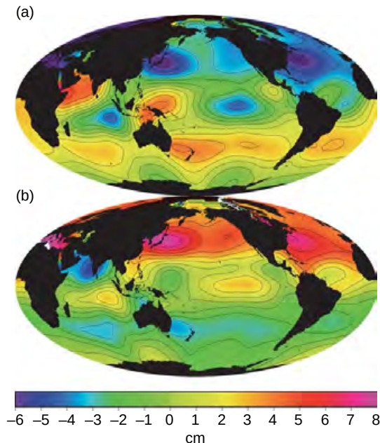
Figure 10 SSH anomalies for average Mar. (a) and average Oct. (b) based on 12 years of T/P and Jason-1 maps that have been smoothed with a 1000-km radius Gaussian.
