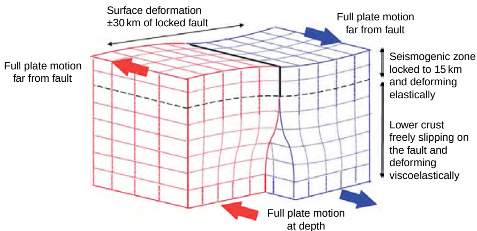
Figure 12 Deformation around a transform plate boundary, such as the San Andreas Fault.
