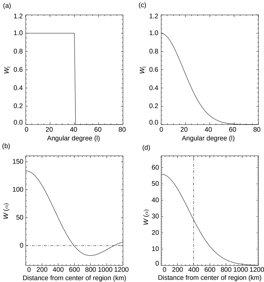
Figure 5 (a) the spectral smoothing coefficients equivalent to truncation at degree l = 40 , and (b) the corresponding smoothing function in the spatial domain. (c) The spectral smoothing coefficients for Gaussian smoothing with a 400-km radius, and (d) the corresponding smoothing function in the spatial domain.
