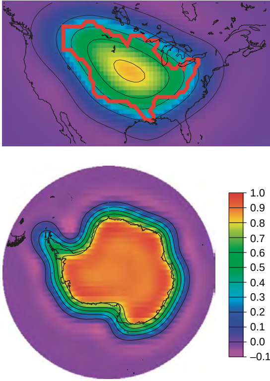
Figure 7 Averaging functions, \bar{W} (see eqn [21]), for the Mississippi River Basin and for Antarctica. The solid lines represent contour intervals of 0.2.
