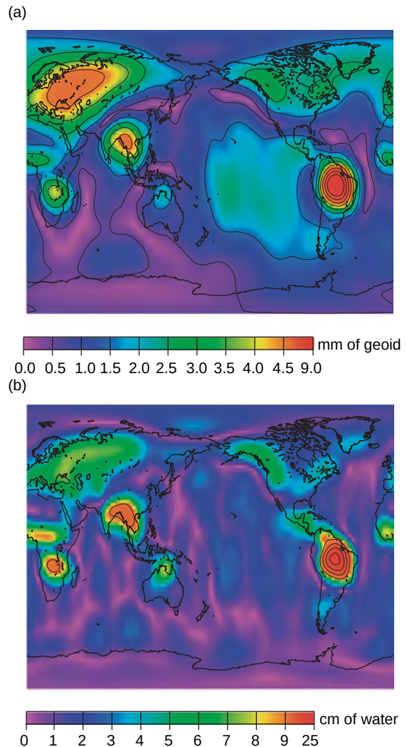
Figure 2 (a) The amplitude of the annual cycle in the geoid, fit to 4 years (spring 2002 to spring 2006) of monthly gravity field solutions from GRACE. A 750-km Gaussian smoothing function has been applied to the results. (b) The corresponding amplitude of the annual cycle in surface mass, also smoothed with a 750-km Gaussian, in units of centimeters of water thickness. The solid lines represent contour intervals of 1 mm in the top panel and 4 cm in the bottom panel.
