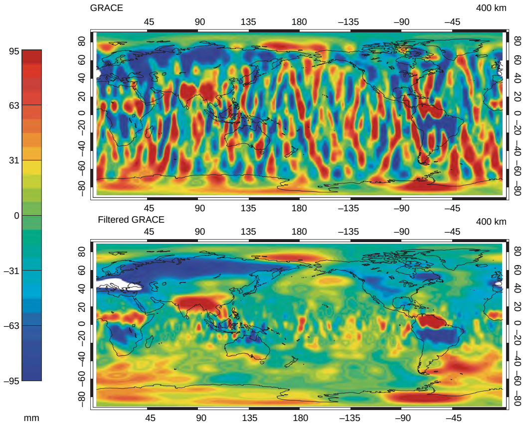
Figure 6 The top panel shows surface mass anomalies deduced from GRACE for a single month, after the temporal mean has been removed. The units are millimeters of water thickness. The bottom panel shows the same thing, but after postprocessing the Stokes coefficients to reduce noise as described by Swenson and Wahr (2006a) . Figure provided by Sean Swenson.
