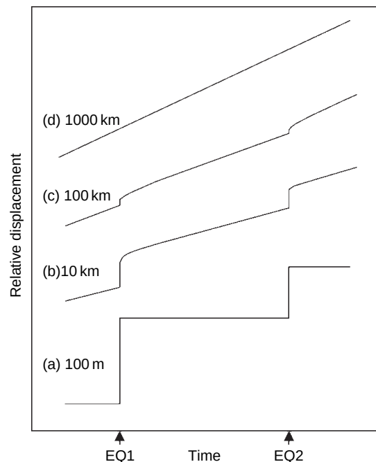
Figure 11 Schematic illustration of the effect of the earthquake cycle on geodetic station positions (see text for explanation).
