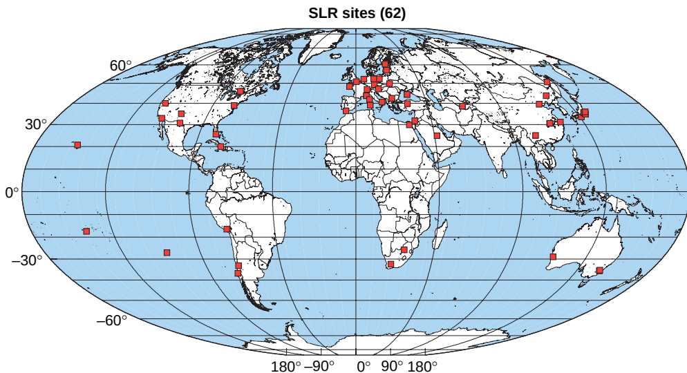
Figure 2 Locations of the 62 SLR sites that are included in the ITRF2005 reference frame. Of the sites shown, about 35 are still actively making measurements. These stations observe continuously with priorities, but not detailed scheduling, set by the International Laser Ranging Service (ILRS).
