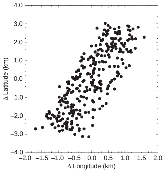
Figure 13 Sub-satellite points in one T/P bin for the entire mission.
