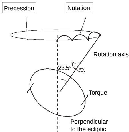
Figure 1 Definition of precession and nutation.
