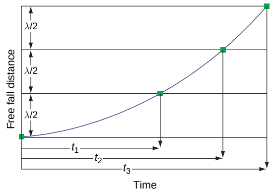
Figure 13 First four zero-crossings of the free-fall gravity meter (position vs. time).
