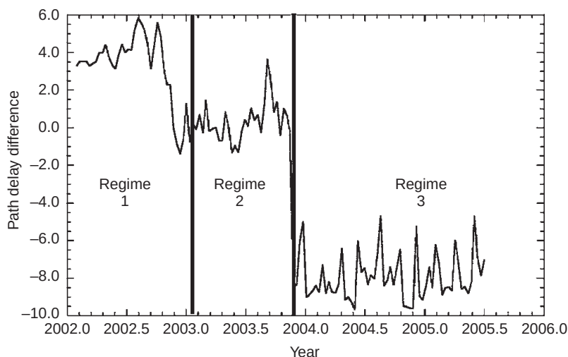
Figure 4 Path delay from JMR minus path delay estimated from ECMWF model stored on GDRs, averaged globally for each repeat cycle. Note that path delays are stored as negative values on GDRs, but that here we have differenced the positive magnitudes.
