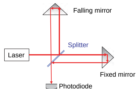
Figure 9 Michelson interferometer used to measure gravity from a falling mirror.
