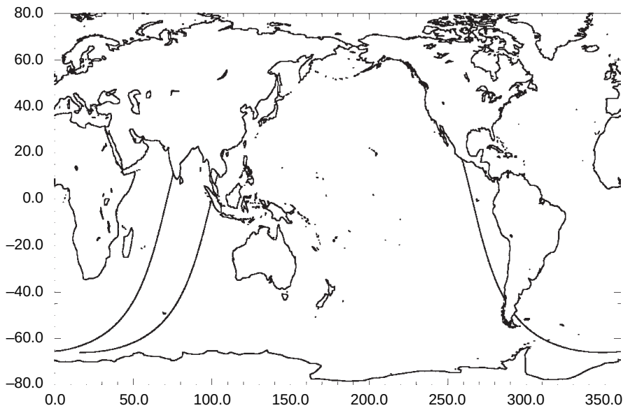
Figure 7 Plot for T/P ground track for first three passes, showing westward shift of ground track in time.
