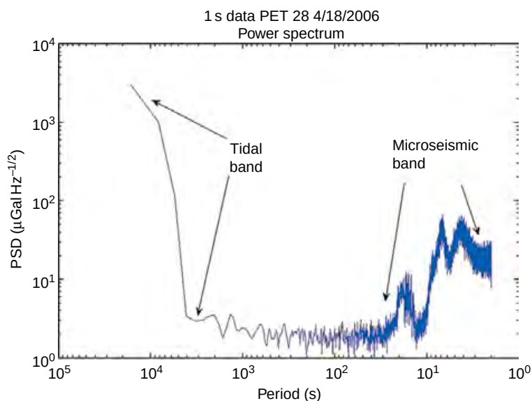
Figure 1 One day of 1 Hz measurements with a portable Earth tide gravity meter.
