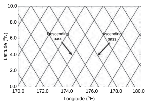
Figure 3 Crossover point for Geosat, showing ascending and descending passes.
